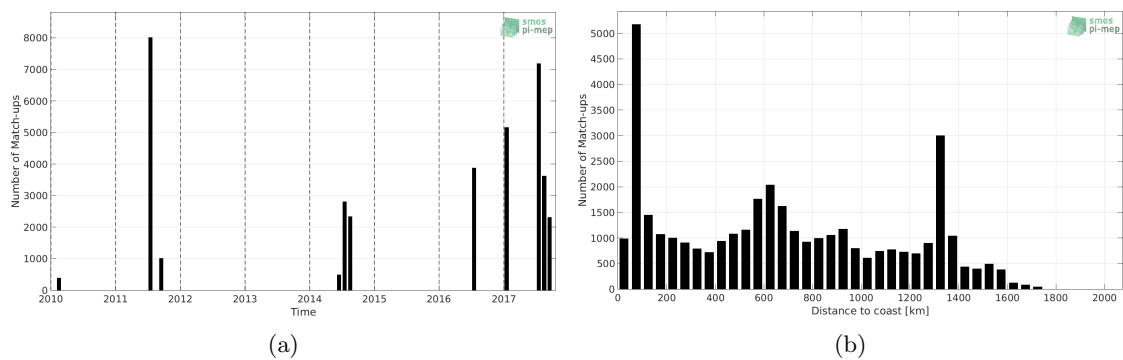
Figure 1: Number of match-ups between TSG-GOSUD-Research-vessel and SMOS-L3-CATDS-CECOS-LOCEAN-V3-18DAYS-25KM SSS as a function of time (a) and as function of the distance to coast (b) over the Gulf Stream Pi-MEP region and for the full satellite product period.
