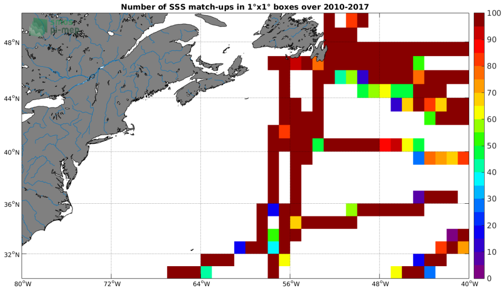
Figure 4: Number of SSS match-ups between TSG-GOSUD-Research-vessel SSS and the SMOS-L3-CATDS-CECOS-LOCEAN-V3-18DAYS-25KM SSS product for the Gulf Stream Pi-MEP region over 1°x1° boxes and for the full satellite product period.
