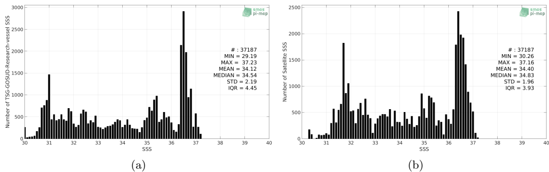
Figure 2: Histograms of SSS from TSG-GOSUD-Research-vessel (a) and SMOS-L3-CATDS-CECOS-LOCEAN-V3-18DAYS-25KM (b) considering all match-up pairs per bins of 0.1 over the Gulf Stream Pi-MEP region and for the full satellite product period.
