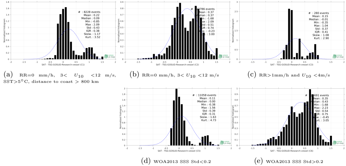
Figure 13: Normalized histogram of \Delta\text{SSS} (SMOS-L3-CATDS-CECOS-LOCEAN-V3-18DAYS-25KM - TSG-GOSUD-Research-vessel) for 5 different subdatasets corresponding to: RR=0 mm/h, 3 < U_{10} < 12 m/s, SST > 5^\circ\text{C} , distance to coast > 800 km (a), RR=0 mm/h, 3 < U_{10} < 12 m/s (b), RR > 1\text{mm/h} and U_{10} < 4\text{m/s} (c), WOA2013 SSS \text{Std} < 0.2 (d), WOA2013 SSS \text{Std} > 0.2 (e).
