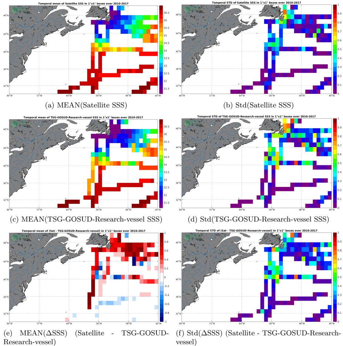
Figure 6: Temporal mean (left) and Std (right) of SSS from SMOS-L3-CATDS-CECOS-LOCEAN-V3-18DAYS-25KM (top), TSG-GOSUD-Research-vessel (middle), and of \Delta SSS (Satellite - TSG-GOSUD-Research-vessel). Only match-up pairs are used to generate these maps.
