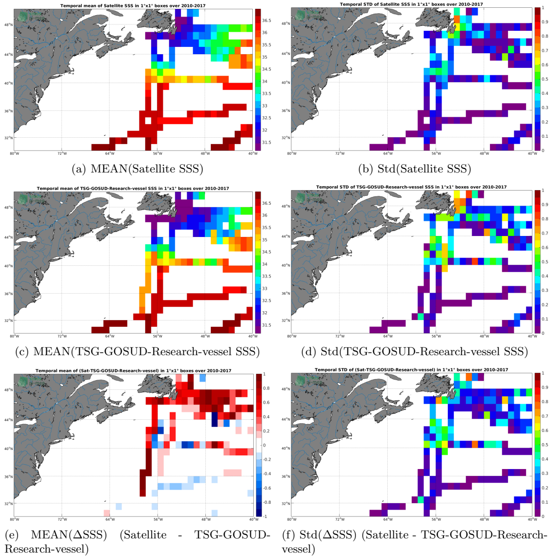
Figure 6: Temporal mean (left) and Std (right) of SSS from SMOS-L3-CATDS-CECOS-LOCEAN-V3-18DAYS-25KM (top), TSG-GOSUD-Research-vessel (middle), and of \Delta\text{SSS} (Satellite - TSG-GOSUD-Research-vessel). Only match-up pairs are used to generate these maps.
