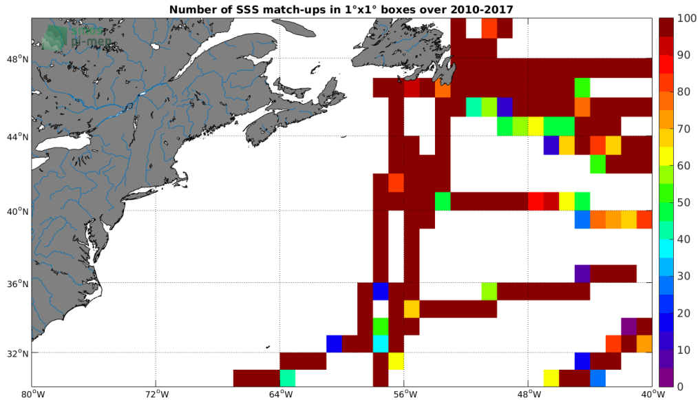
Figure 4: Number of SSS match-ups between TSG-GOSUD-Research-vessel SSS and the SMOS-L3-CATDS-CECOS-LOCEAN-V3-18DAYS-25KM SSS product for the Gulf Stream Pi-MEP region over 1^\circ \times 1^\circ boxes and for the full satellite product period.
