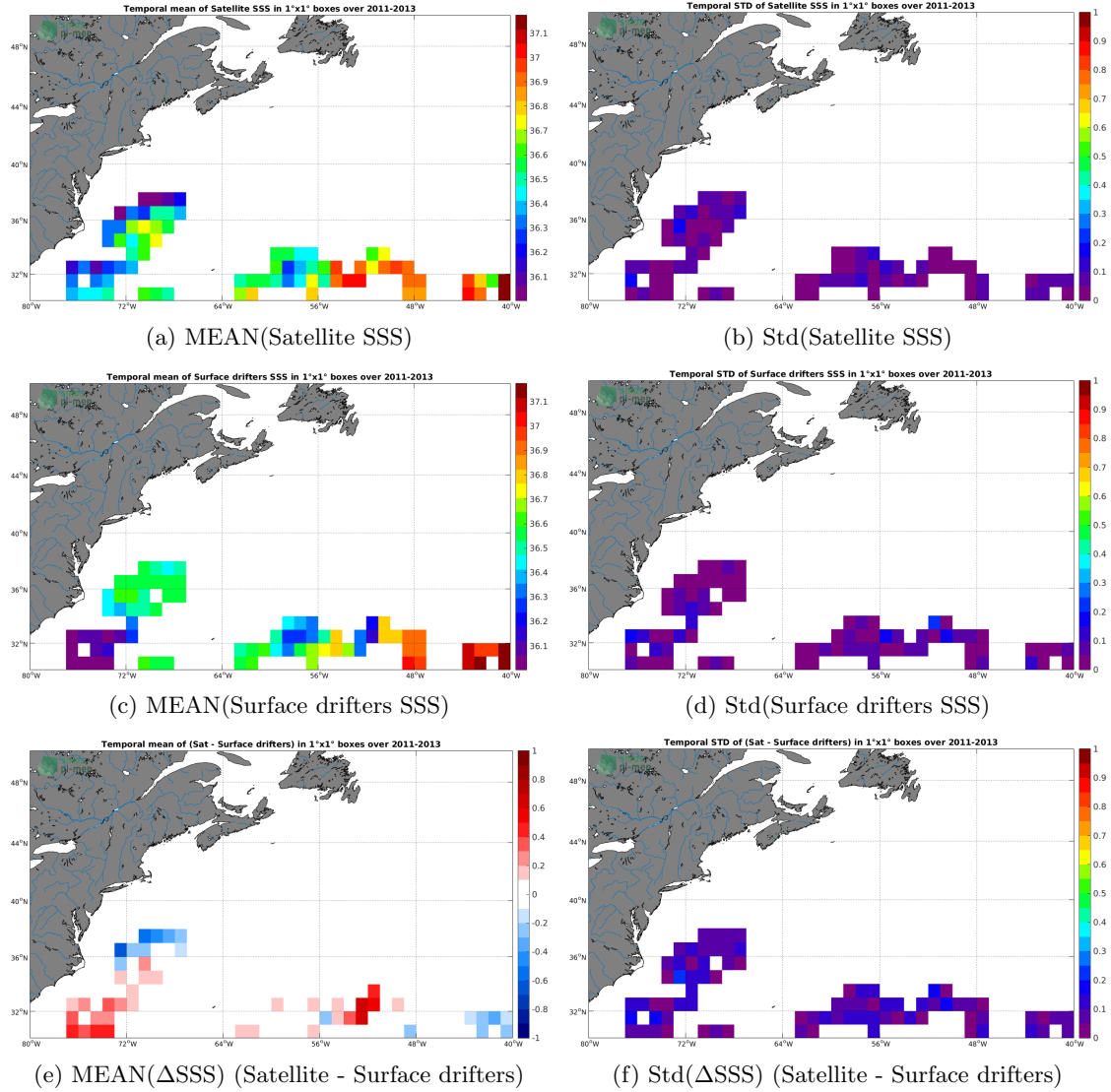
Figure 5: Temporal mean (left) and Std (right) of SSS from SMOS-L3-CATDS-CECOS-LOCEAN-V3-18DAYS-25KM (top), Surface drifters (middle), and of \Delta\text{SSS} (Satellite - Surface drifters). Only match-up pairs are used to generate these maps.
