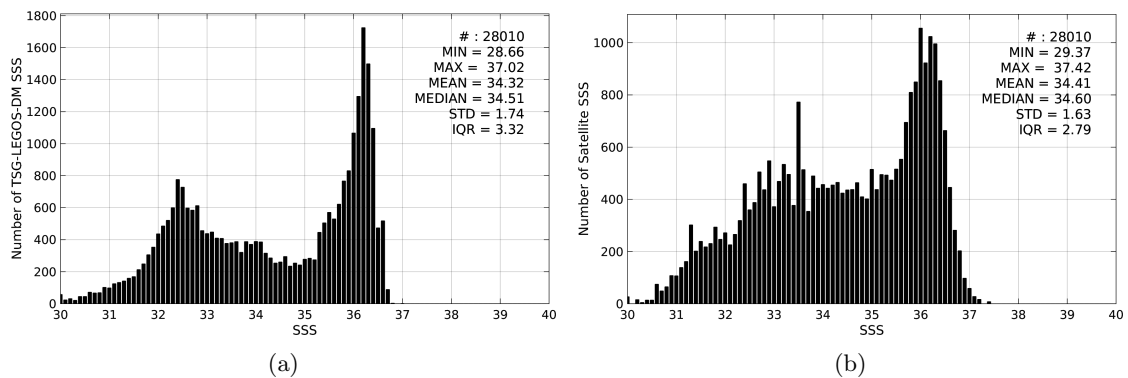
Figure 2: Histograms of SSS from TSG-LEGOS-DM (a) and SMOS-L3-CATDS-CECOS-LOCEAN-V2.1-9DAYS-25KM (b) considering all match-up pairs per bins of 0.1 over the Gulf Stream Pi-MEP region and for the full satellite product period.
