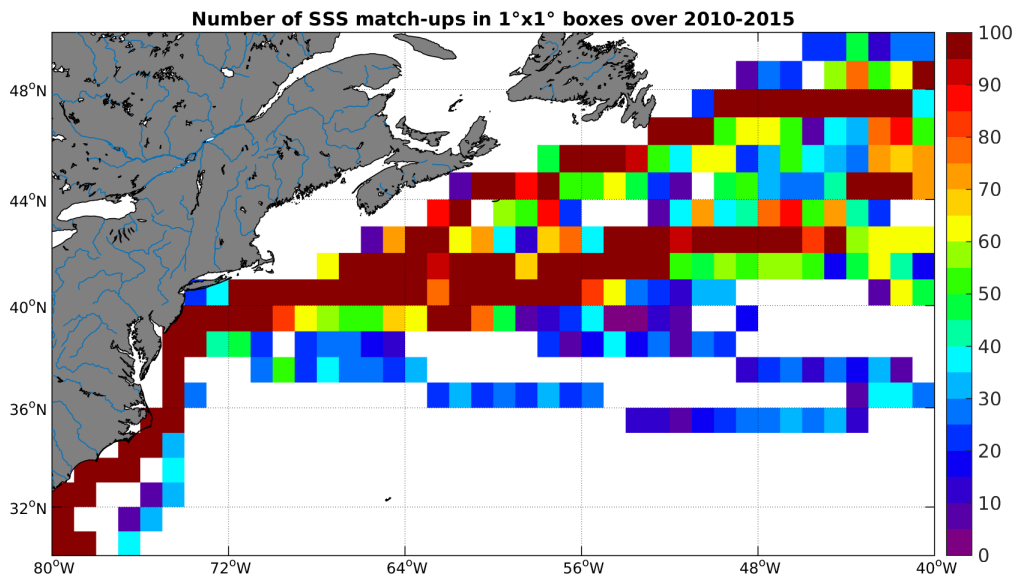
Figure 4: Number of SSS match-ups between TSG-LEGOS-DM SSS and the SMOS-L3-CATDS-CECOS-LOCEAN-V2.1-9DAYS-25KM SSS product for the Gulf Stream Pi-MEP region over 1^\circ \times 1^\circ boxes and for the full satellite product period.
