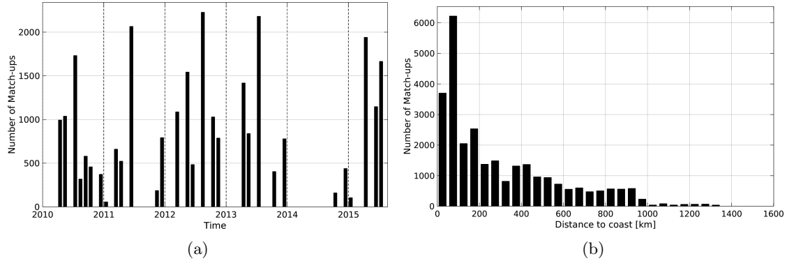
Figure 1: Number of match-ups between TSG-LEGOS-DM and SMOS-L3-CATDS-CECOS-LOCEAN-V2.1-9DAYS-25KM SSS as a function of time (a) and as function of the distance to coast (b) over the Gulf Stream Pi-MEP region and for the full satellite product period.
