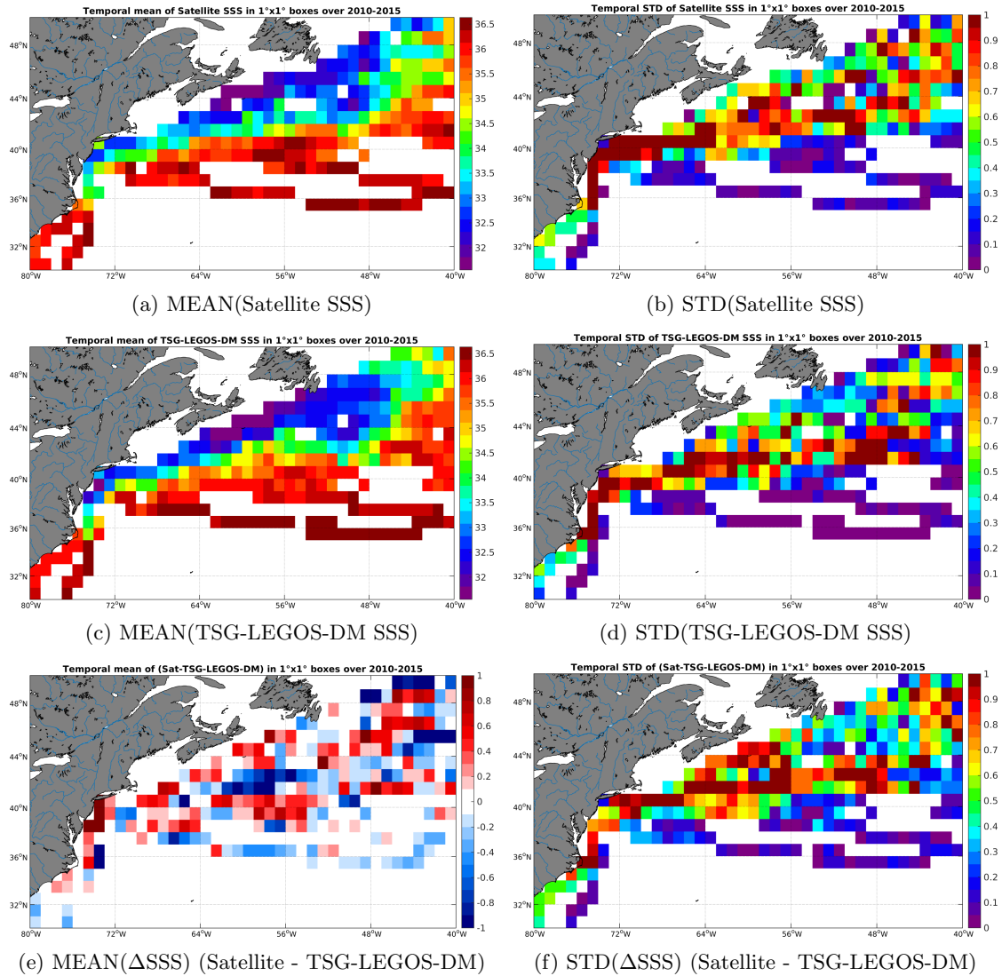
Figure 6: Temporal mean (left) and STD (right) of SSS from SMOS-L3-CATDS-CECOS-LOCEAN-V2.1-9DAYS-25KM (top), TSG-LEGOS-DM (middle), and of \Delta SSS (Satellite - TSG-LEGOS-DM). Only match-up pairs are used to generate these maps.
