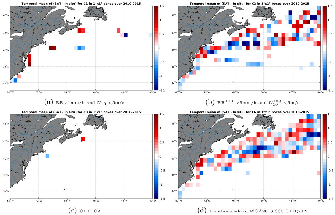
Figure 12: Temporal mean gridded over spatial boxes of size 1^\circ \times 1^\circ of \Delta SSS (SMOS-L3-CATDS-CECOS-LOCEAN-V2.1-9DAYS-25KM - TSG-LEGOS-DM) for 4 different subdatasets corresponding to: RR > 1mm/h and U_{10} < 5\text{m/s} (a), RR^{10d} > 5\text{mm/h} and U_{10}^{10d} < 5\text{m/s} (b), C1 U C2 (c), Locations where WOA2013 SSS STD > 0.2 (d).
