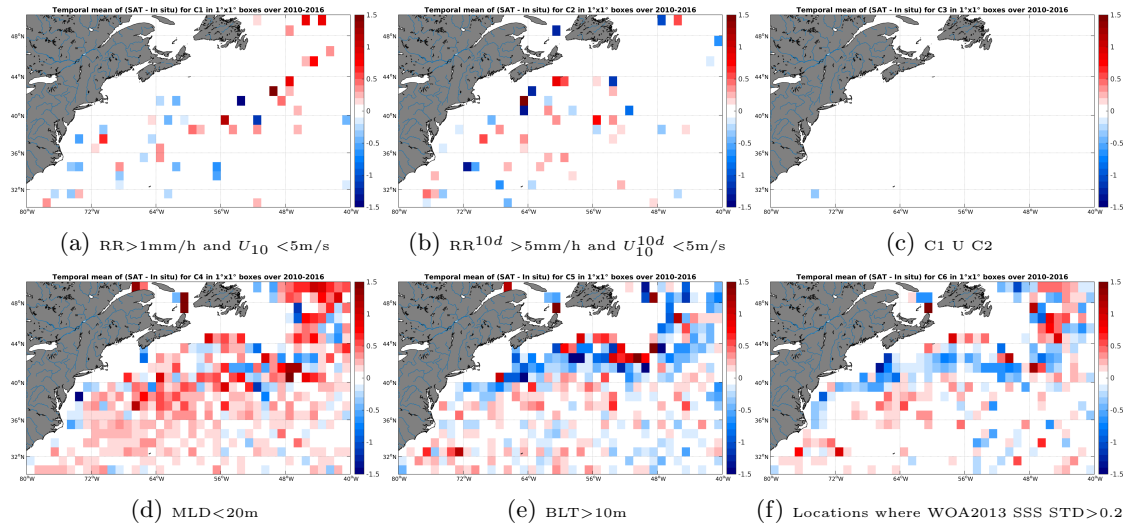
Figure 12: Temporal mean gridded over spatial boxes of size 1^\circ \times 1^\circ of \Delta SSS (SMOS-L3-CATDS-CECOS-LOCEAN-V2.1-9DAYS-25KM - Argo) for 6 different subdatasets corresponding to: RR > 1\text{mm/h} and U_{10} < 5\text{m/s} (a), RR^{10d} > 5\text{mm/h} and U_{10}^{10d} < 5\text{m/s} (b), C1 U C2 (c), MLD < 20\text{m} (d), BLT > 10\text{m} (e), Locations where WOA2013 SSS STD > 0.2 (f).
