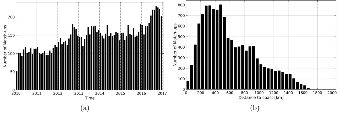
Figure 1: Number of match-ups between Argo and SMOS-L3-CATDS-CECOS-LOCEAN-V2.1-9DAYS-25KM SSS as a function of time (a) and as function of the distance to coast (b) over the Gulf Stream Pi-MEP region and for the full satellite product period.
