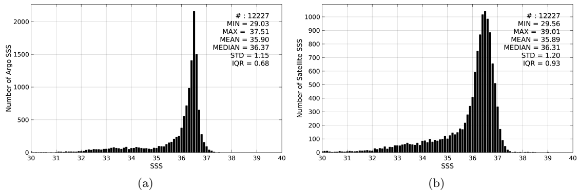
Figure 2: Histograms of SSS from Argo (a) and SMOS-L3-CATDS-CECOS-LOCEAN-V2.1-9DAYS-25KM (b) considering all match-up pairs per bins of 0.1 over the Gulf Stream Pi-MEP region and for the full satellite product period.
