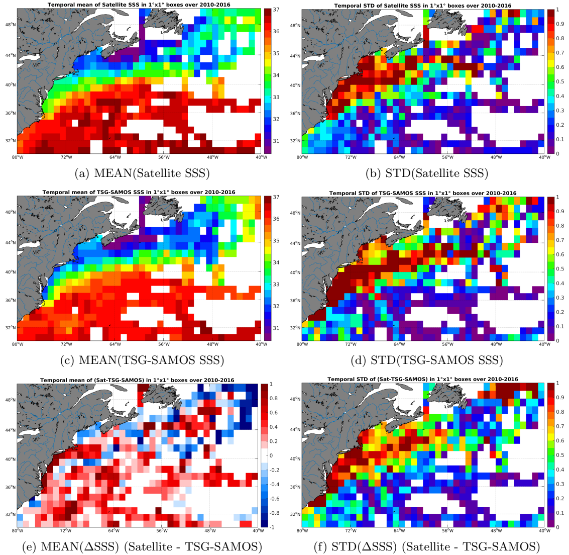
Figure 6: Temporal mean (left) and STD (right) of SSS from SMOS-L3-CATDS-CECOS-LOCEAN-V2-9DAYS-25KM (top), TSG-SAMOS (middle), and of \Delta SSS (Satellite - TSG-SAMOS). Only match-up pairs are used to generate these maps.
