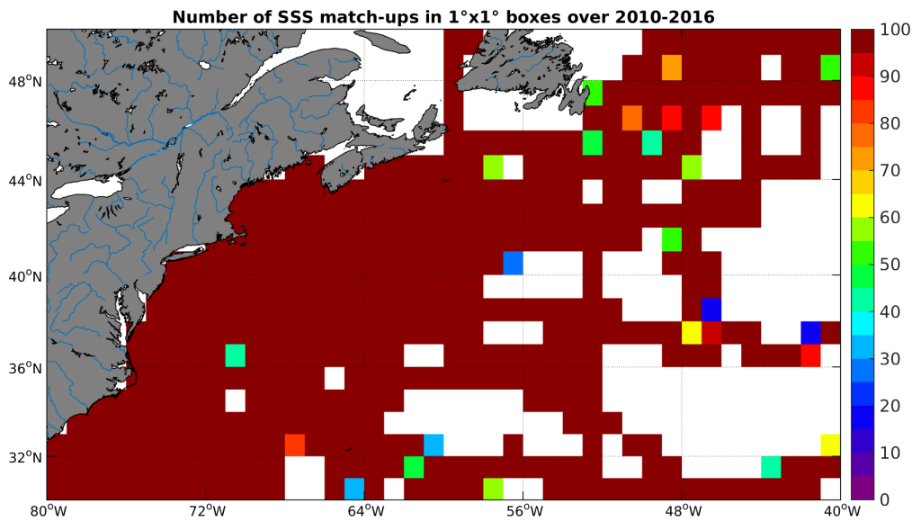
Figure 4: Number of SSS match-ups between TSG-SAMOS SSS and the SMOS-L3-CATDS-CECOS-LOCEAN-V2-9DAYS-25KM SSS product for the Gulf Stream Pi-MEP region over 1^\circ \times 1^\circ boxes and for the full satellite product period.
