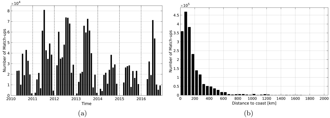
Figure 1: Number of match-ups between TSG-SAMOS and SMOS-L3-CATDS-CECOS-LOCEAN-V2-9DAYS-25KM SSS as a function of time (a) and as function of the distance to coast (b) over the Gulf Stream Pi-MEP region and for the full satellite product period.
