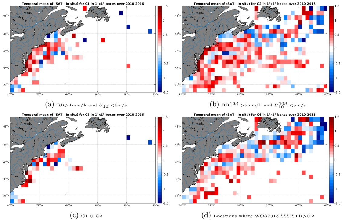
Figure 12: Temporal mean gridded over spatial boxes of size 1^\circ \times 1^\circ of \Delta SSS (SMOS-L3-CATDS-CECOS-LOCEAN-V2-9DAYS-25KM - TSG-SAMOS) for 4 different subdatasets corresponding to: RR > 1\text{mm/h} and U_{10} < 5\text{m/s} (a), RR^{10d} > 5\text{mm/h} and U_{10}^{10d} < 5\text{m/s} (b), C1 U C2 (c), Locations where WOA2013 SSS STD > 0.2 (d).
