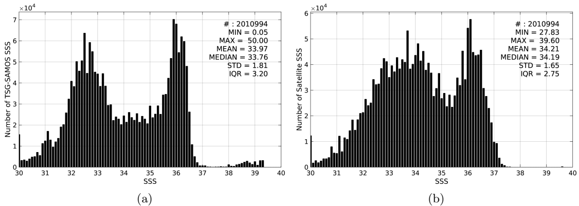
Figure 2: Histograms of SSS from TSG-SAMOS (a) and SMOS-L3-CATDS-CECOS-LOCEAN-V2-9DAYS-25KM (b) considering all match-up pairs per bins of 0.1 over the Gulf Stream Pi-MEP region and for the full satellite product period.
