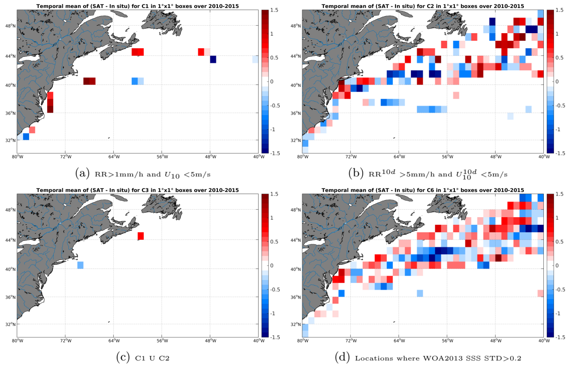
Figure 12: Temporal mean gridded over spatial boxes of size 1^\circ \times 1^\circ of \Delta SSS (SMOS-L3-CATDS-CECOS-LOCEAN-V2-9DAYS-25KM - TSG-LEGOS-DM) for 4 different subdatasets corresponding to: RR > 1 mm/h and U_{10} < 5 m/s (a), RR 10d > 5 mm/h and U_{10}^{10d} < 5 m/s (b), C1 U C2 (c), Locations where WOA2013 SSS STD > 0.2 (d).
