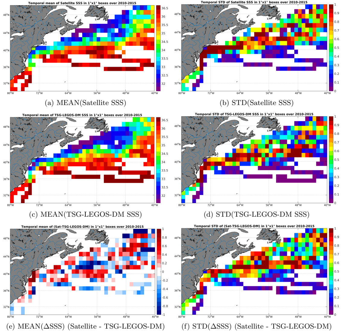
Figure 6: Temporal mean (left) and STD (right) of SSS from SMOS-L3-CATDS-CECOS-LOCEAN-V2-9DAYS-25KM (top), TSG-LEGOS-DM (middle), and of \Delta SSS (Satellite - TSG-LEGOS-DM). Only match-up pairs are used to generate these maps.
