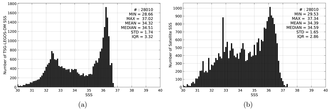
Figure 2: Histograms of SSS from TSG-LEGOS-DM (a) and SMOS-L3-CATDS-CECOS-LOCEAN-V2-9DAYS-25KM (b) considering all match-up pairs per bins of 0.1 over the Gulf Stream Pi-MEP region and for the full satellite product period.
