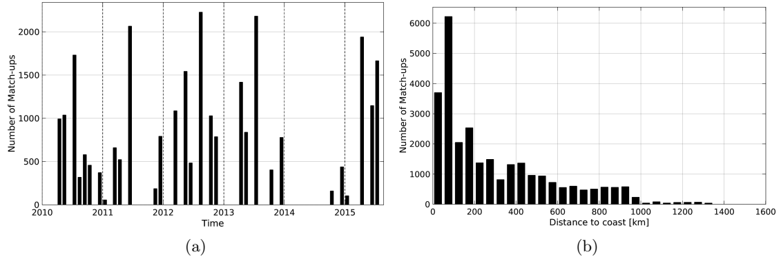
Figure 1: Number of match-ups between TSG-LEGOS-DM and SMOS-L3-CATDS-CECOS-LOCEAN-V2-9DAYS-25KM SSS as a function of time (a) and as function of the distance to coast (b) over the Gulf Stream Pi-MEP region and for the full satellite product period.
