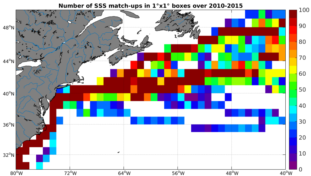
Figure 4: Number of SSS match-ups between TSG-LEGOS-DM SSS and the SMOS-L3-CATDS-CECOS-LOCEAN-V2-9DAYS-25KM SSS product for the Gulf Stream Pi-MEP region over 1^\circ \times 1^\circ boxes and for the full satellite product period.
