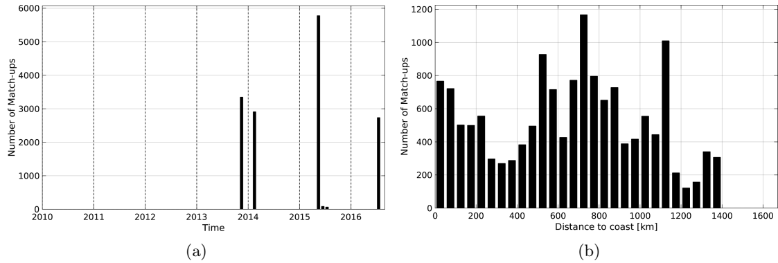
Figure 1: Number of match-ups between TSG-GOSUD-Sailing-ship and SMOS-L3-CATDS-CECOS-LOCEAN-V2-9DAYS-25KM SSS as a function of time (a) and as function of the distance to coast (b) over the Gulf Stream Pi-MEP region and for the full satellite product period.
