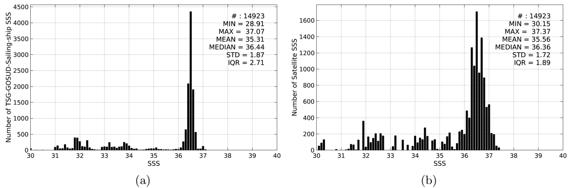
Figure 2: Histograms of SSS from TSG-GOSUD-Sailing-ship (a) and SMOS-L3-CATDS-CECOS-LOCEAN-V2-9DAYS-25KM (b) considering all match-up pairs per bins of 0.1 over the Gulf Stream Pi-MEP region and for the full satellite product period.
