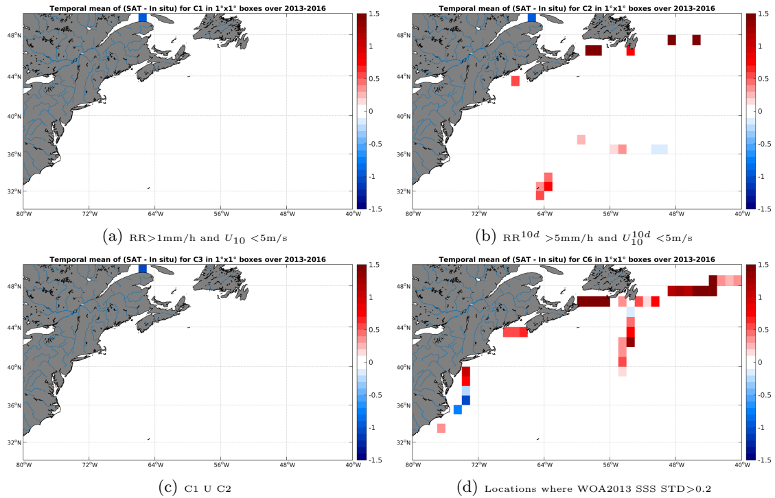
Figure 12: Temporal mean gridded over spatial boxes of size 1°x1° of \Delta SSS (SMOS-L3-CATDS-CECOS-LOCEAN-V2-9DAYS-25KM - TSG-GOSUD-Sailing-ship) for 4 different subdatasets corresponding to:RR>1mm/h and U_{10} < 5 m/s (a), RR^{10d} > 5 mm/h and U_{10}^{10d} < 5 m/s (b), C1 U C2 (c),Locations where WOA2013 SSS STD>0.2 (d).
