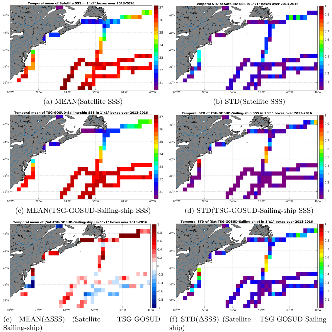
Figure 6: Temporal mean (left) and STD (right) of SSS from SMOS-L3-CATDS-CECOS-LOCEAN-V2-9DAYS-25KM (top), TSG-GOSUD-Sailing-ship (middle), and of \Delta SSS (Satellite - TSG-GOSUD-Sailing-ship). Only match-up pairs are used to generate these maps.
