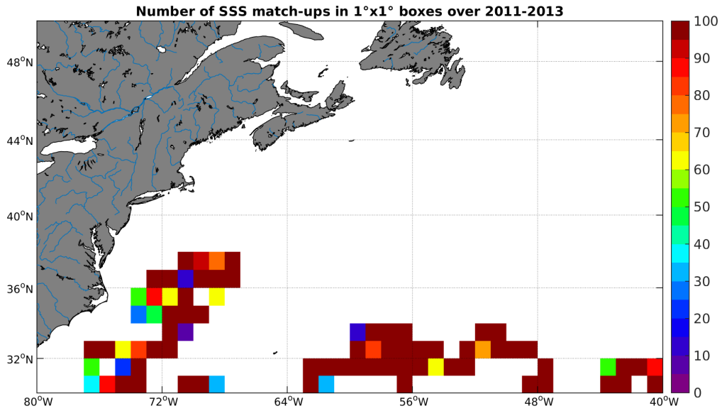
Figure 3: Number of SSS match-ups between Surface drifters SSS and the SMOS-L3-CATDS-CECOS-LOCEAN-V2-9DAYS-25KM SSS product for the Gulf Stream Pi-MEP region over 1^\circ \times 1^\circ boxes and for the full satellite product period.
