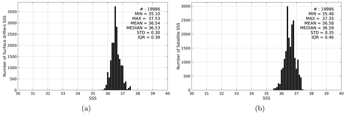
Figure 2: Histograms of SSS from Surface drifters (a) and SMOS-L3-CATDS-CECOS-LOCEAN-V2-9DAYS-25KM (b) considering all match-up pairs per bins of 0.1 over the Gulf Stream Pi-MEP region and for the full satellite product period.
