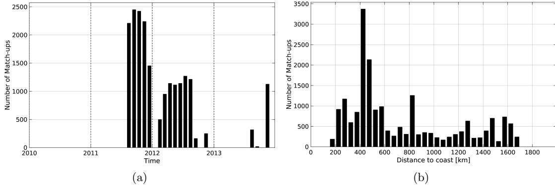
Figure 1: Number of match-ups between Surface drifters and SMOS-L3-CATDS-CECOS-LOCEAN-V2-9DAYS-25KM SSS as a function of time (a) and as function of the distance to coast (b) over the Gulf Stream Pi-MEP region and for the full satellite product period.
