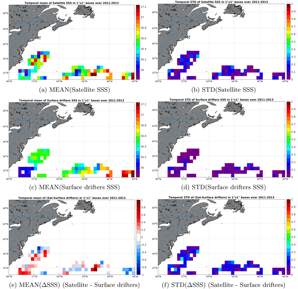
Figure 5: Temporal mean (left) and STD (right) of SSS from SMOS-L3-CATDS-CECOS-LOCEAN-V2-9DAYS-25KM (top), Surface drifters (middle), and of \Delta SSS (Satellite - Surface drifters). Only match-up pairs are used to generate these maps.
