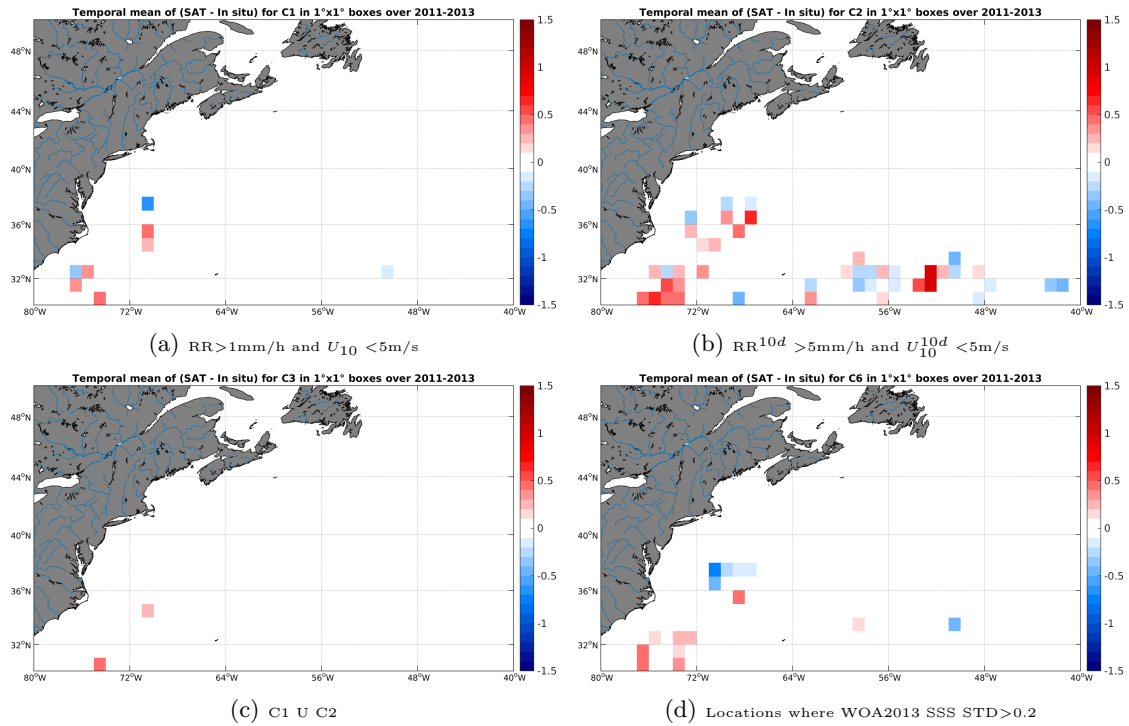
Figure 11: Temporal mean gridded over spatial boxes of size 1^\circ \times 1^\circ of \Delta SSS (SMOS-L3-CATDS-CECOS-LOCEAN-V2-9DAYS-25KM - Surface drifters) for 4 different subdatasets corresponding to: RR > 1mm/h and U_{10} < 5 m/s (a), RR^{10d} > 5 mm/h and U_{10}^{10d} < 5 m/s (b), C1 U C2 (c), Locations where WOA2013 SSS STD > 0.2 (d).
