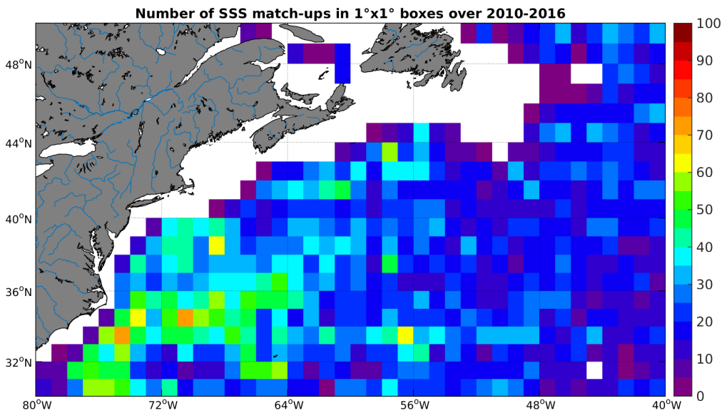
Figure 4: Number of SSS match-ups between Argo SSS and the SMOS-L3-CATDS-CECOS-LOCEAN-V2-9DAYS-25KM SSS product for the Gulf Stream Pi-MEP region over 1°x1° boxes and for the full satellite product period.
