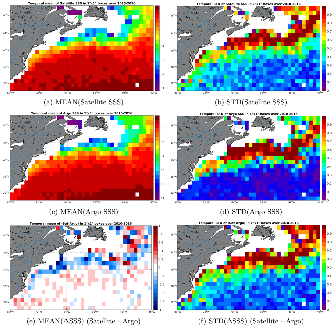
Figure 6: Temporal mean (left) and STD (right) of SSS from SMOS-L3-CATDS-CECOS-LOCEAN-V2-9DAYS-25KM (top), Argo (middle), and of \Delta SSS (Satellite - Argo). Only match-up pairs are used to generate these maps.
