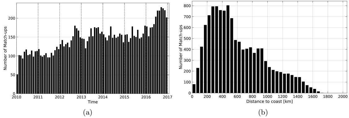
Figure 1: Number of match-ups between Argo and SMOS-L3-CATDS-CECOS-LOCEAN-V2-9DAYS-25KM SSS as a function of time (a) and as function of the distance to coast (b) over the Gulf Stream Pi-MEP region and for the full satellite product period.
