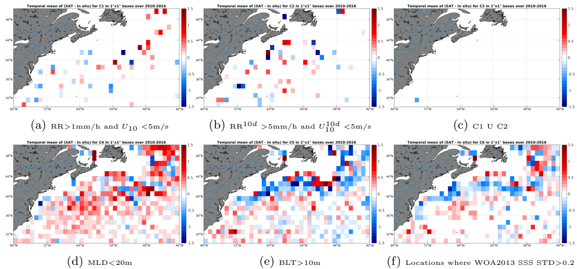
Figure 12: Temporal mean gridded over spatial boxes of size 1^\circ \times 1^\circ of \Delta SSS (SMOS-L3-CATDS-CECOS-LOCEAN-V2-9DAYS-25KM - Argo) for 6 different subdatasets corresponding to:RR>1mm/h and U_{10} < 5\text{m/s} (a), RR^{10d} > 5\text{mm/h} and U_{10}^{10d} < 5\text{m/s} (b), C1 U C2 (c),MLD<20m (d),BLT>10m (e),Locations where WOA2013 SSS STD>0.2 (f).
