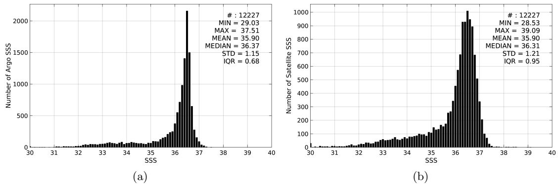
Figure 2: Histograms of SSS from Argo (a) and SMOS-L3-CATDS-CECOS-LOCEAN-V2-9DAYS-25KM (b) considering all match-up pairs per bins of 0.1 over the Gulf Stream Pi-MEP region and for the full satellite product period.
