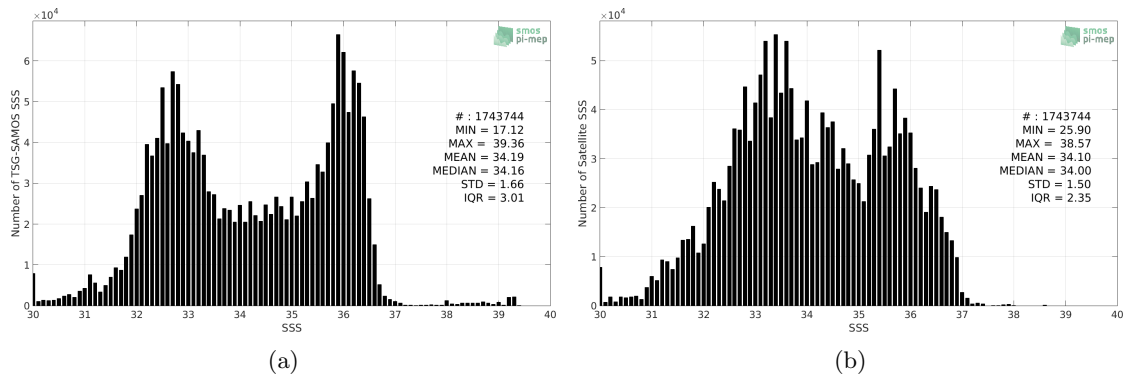
Figure 2: Histograms of SSS from TSG-SAMOS (a) and SMOS L3 v2 - Monthly - 0.25 Deg (CATDS-CECOS-IFREMER) (b) considering all match-up pairs per bins of 0.1 over the Gulf Stream Pi-MEP region and for the full satellite product period.
