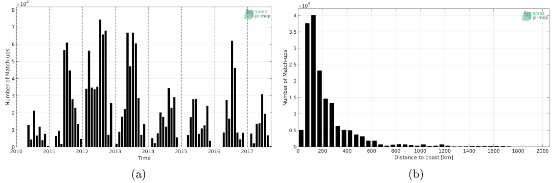
Figure 1: Number of match-ups between TSG-SAMOS and SMOS-L3-CATDS-IFREMER-CECOS-V2-MONTHLY-0.25DEG SSS as a function of time (a) and as function of the distance to coast (b) over the Gulf Stream Pi-MEP region and for the full satellite product period.
