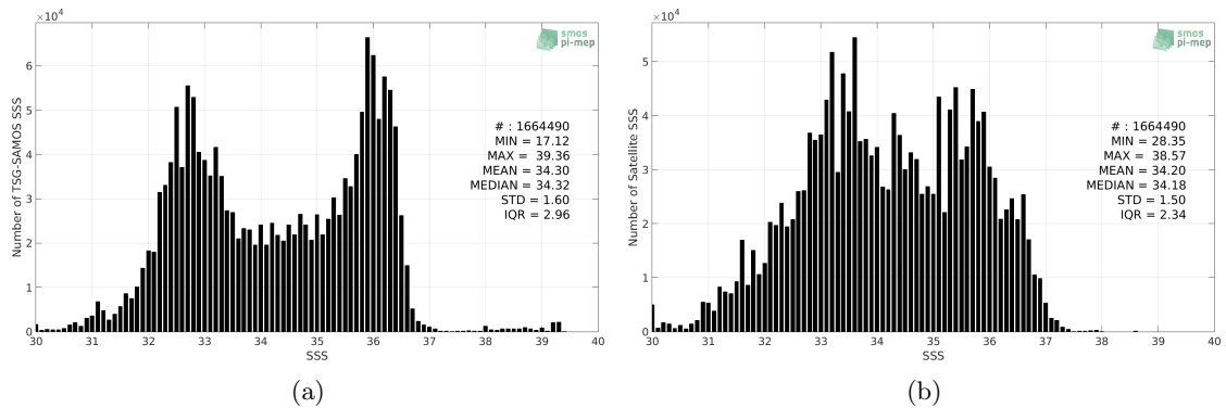
Figure 2: Histograms of SSS from TSG-SAMOS (a) and SMOS-L3-CATDS-IFREMER-CECOS-V2-MONTHLY-0.25DEG (b) considering all match-up pairs per bins of 0.1 over the Gulf Stream Pi-MEP region and for the full satellite product period.
