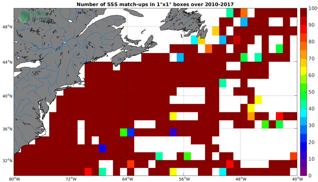
Figure 4: Number of SSS match-ups between TSG-SAMOS SSS and the SMOS-L3-CATDS-IFREMER-CECOS-V2-MONTHLY-0.25DEG SSS product for the Gulf Stream Pi-MEP region over 1^\circ \times 1^\circ boxes and for the full satellite product period.
