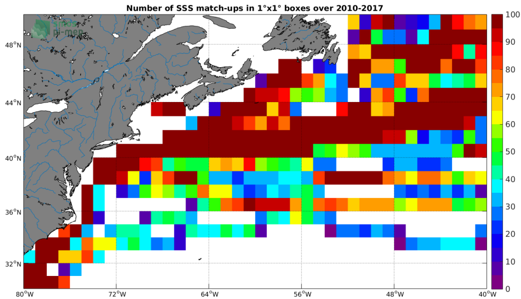
Figure 4: Number of SSS match-ups between TSG (LEGOS-DM) SSS and the SMOS SSS L3 v2 - Monthly - 0.25 Deg (CATDS-CECOS-IFREMER) SSS product for the Gulf Stream Pi-MEP region over 1^\circ \times 1^\circ boxes and for the full satellite product period.
