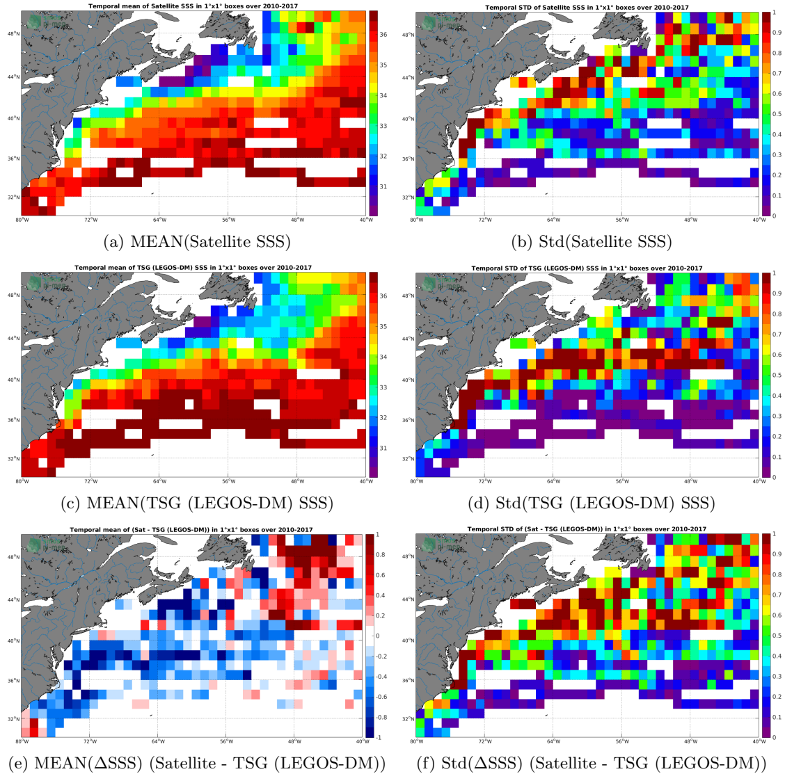
Figure 6: Temporal mean (left) and Std (right) of SSS from SMOS SSS L3 v2 - Monthly - 0.25 Deg (CATDS-CECOS-IFREMER) (top), TSG (LEGOS-DM) ( in situ ) dataset (middle), and of \Delta SSS (Satellite - TSG (LEGOS-DM)). Only match-up pairs are used to generate these maps.
