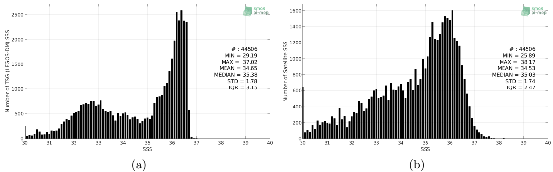
Figure 2: Histograms of SSS from TSG (LEGOS-DM) (a) and SMOS SSS L3 v2 - Monthly - 0.25 Deg (CATDS-CECOS-IFREMER) (b) considering all match-up pairs per bins of 0.1 over the Gulf Stream Pi-MEP region and for the full satellite product period.
