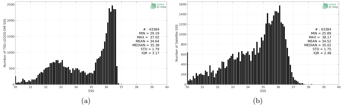
Figure 2: Histograms of SSS from TSG-LEGOS-DM (a) and SMOS L3 v2 - Monthly - 0.25 Deg (CATDS-CECOS-IFREMER) (b) considering all match-up pairs per bins of 0.1 over the Gulf Stream Pi-MEP region and for the full satellite product period.
