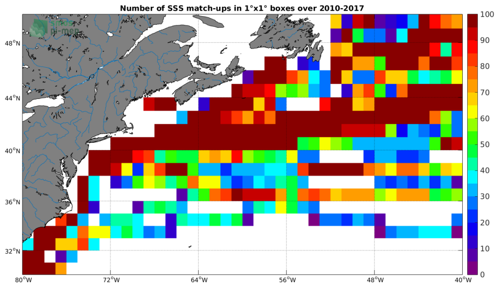
Figure 4: Number of SSS match-ups between TSG-LEGOS-DM SSS and the SMOS L3 v2 - Monthly - 0.25 Deg (CATDS-CECOS-IFREMER) SSS product for the Gulf Stream Pi-MEP region over 1^\circ \times 1^\circ boxes and for the full satellite product period.
