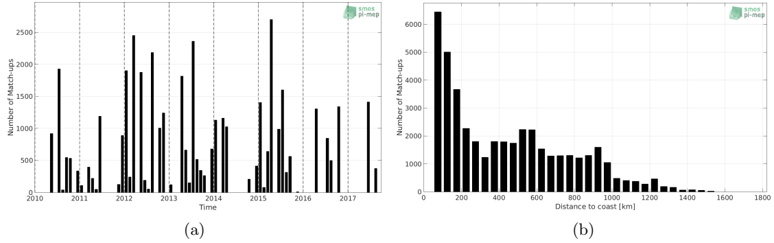
Figure 1: Number of match-ups between TSG-LEGOS-DM and SMOS L3 v2 - Monthly - 0.25 Deg (CATDS-CECOS-IFREMER) SSS as a function of time (a) and as function of the distance to coast (b) over the Gulf Stream Pi-MEP region and for the full satellite product period.
