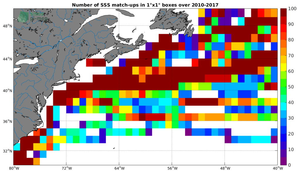
Figure 4: Number of SSS match-ups between TSG-LEGOS-DM SSS and the SMOS-L3-CATDS-IFREMER-CECOS-V2-MONTHLY-0.25DEG SSS product for the Gulf Stream Pi-MEP region over 1^\circ \times 1^\circ boxes and for the full satellite product period.
