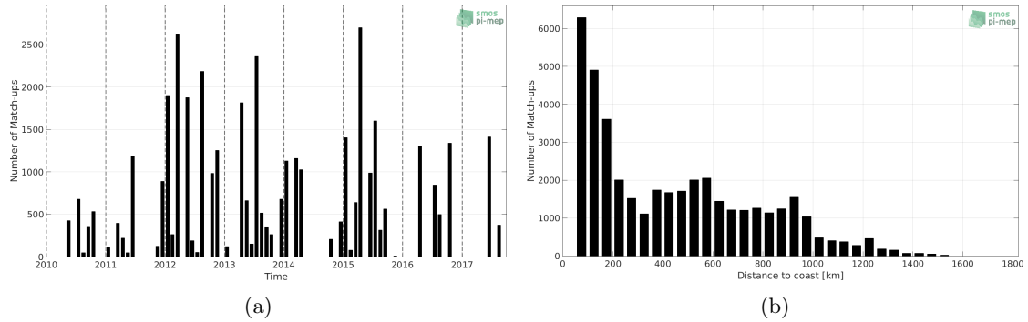
Figure 1: Number of match-ups between TSG-LEGOS-DM and SMOS-L3-CATDS-IFREMER-CECOS-V2-MONTHLY-0.25DEG SSS as a function of time (a) and as function of the distance to coast (b) over the Gulf Stream Pi-MEP region and for the full satellite product period.
