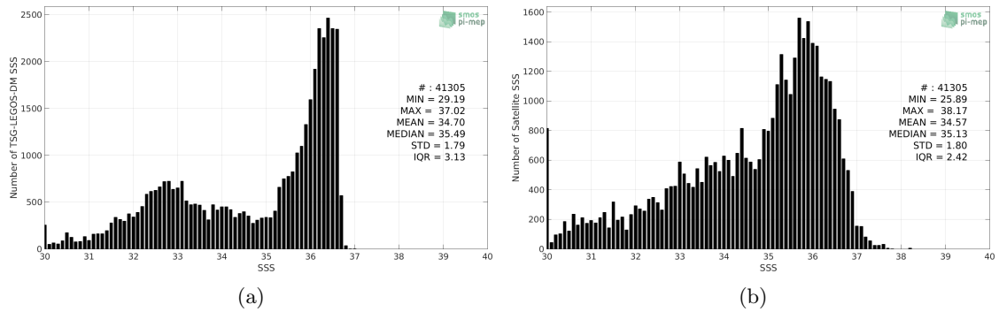
Figure 2: Histograms of SSS from TSG-LEGOS-DM (a) and SMOS-L3-CATDS-IFREMER-CECOS-V2-MONTHLY-0.25DEG (b) considering all match-up pairs per bins of 0.1 over the Gulf Stream Pi-MEP region and for the full satellite product period.
