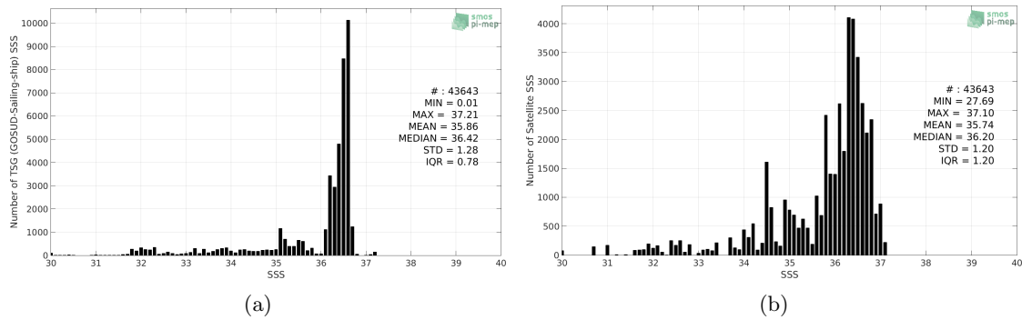
Figure 2: Histograms of SSS from TSG (GOSUD-Sailing-ship) (a) and SMOS SSS L3 v2 - Monthly - 0.25 Deg (CATDS-CECOS-IFREMER) (b) considering all match-up pairs per bins of 0.1 over the Gulf Stream Pi-MEP region and for the full satellite product period.
