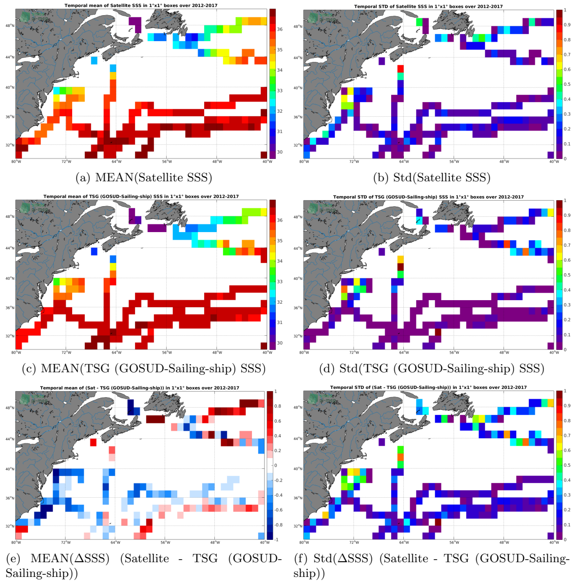
Figure 6: Temporal mean (left) and Std (right) of SSS from SMOS SSS L3 v2 - Monthly - 0.25 Deg (CATDS-CECOS-IFREMER) (top), TSG (GOSUD-Sailing-ship) (middle), and of \Delta SSS (Satellite - TSG (GOSUD-Sailing-ship)). Only match-up pairs are used to generate these maps.
