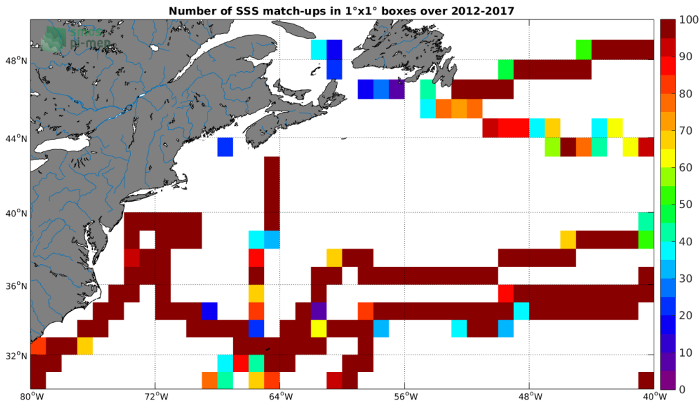
Figure 4: Number of SSS match-ups between TSG (GOSUD-Sailing-ship) SSS and the SMOS SSS L3 v2 - Monthly - 0.25 Deg (CATDS-CECOS-IFREMER) SSS product for the Gulf Stream Pi-MEP region over 1^\circ \times 1^\circ boxes and for the full satellite product period.
