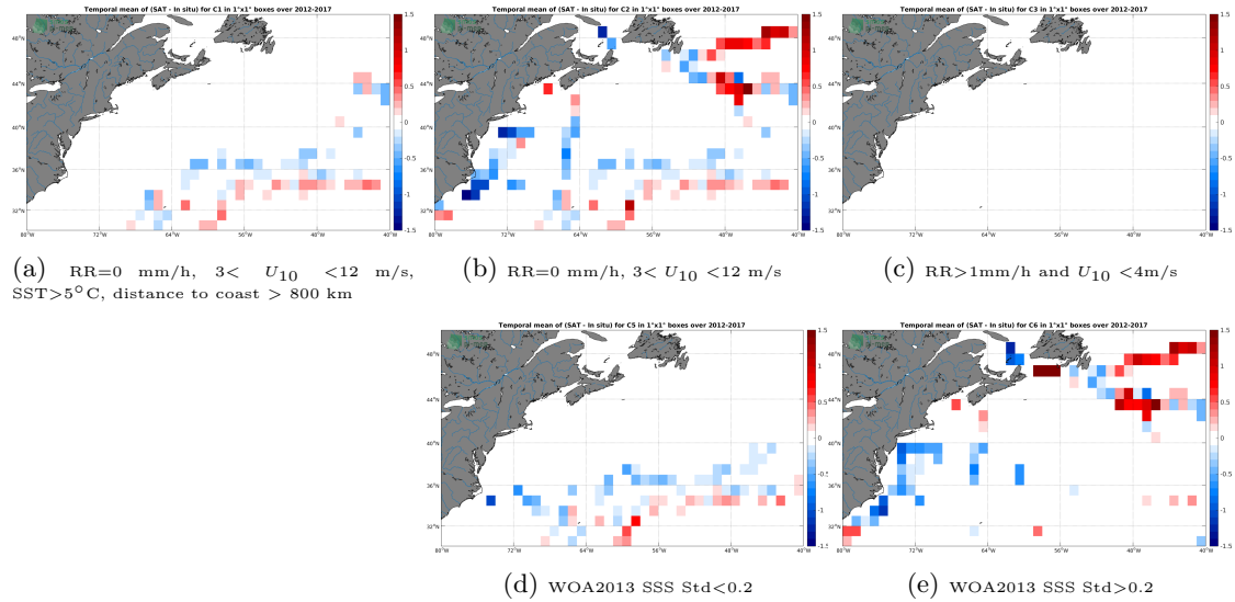
Figure 12: Temporal mean gridded over spatial boxes of size 1^{\circ}\times 1^{\circ} of \Delta SSS (SMOS L3 v2 - Monthly - 0.25 Deg (CATDS-CECOS-IFREMER) - TSG-GOSUD-Sailing-ship) for 5 different subdatasets corresponding to:RR=0 mm/h, 3 < U_{10} < 12 m/s, SST >5^{\circ}\text{C} , distance to coast > 800 km (a), RR=0 mm/h, 3 < U_{10} < 12 m/s (b), RR >1 mm/h and U_{10} < 4 m/s (c), WOA2013 SSS Std <0.2 (d), WOA2013 SSS Std >0.2 (e).
