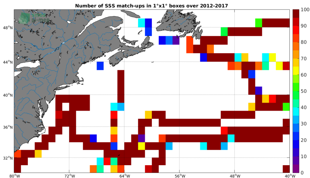
Figure 4: Number of SSS match-ups between TSG-GOSUD-Sailing-ship SSS and the SMOS L3 v2 - Monthly - 0.25 Deg (CATDS-CECOS-IFREMER) SSS product for the Gulf Stream Pi-MEP region over 1^\circ \times 1^\circ boxes and for the full satellite product period.
