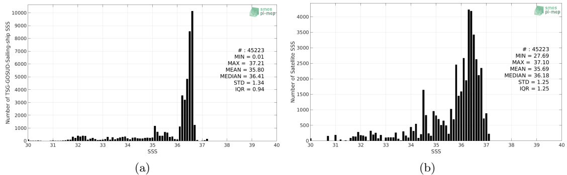
Figure 2: Histograms of SSS from TSG-GOSUD-Sailing-ship (a) and SMOS L3 v2 - Monthly - 0.25 Deg (CATDS-CECOS-IFREMER) (b) considering all match-up pairs per bins of 0.1 over the Gulf Stream Pi-MEP region and for the full satellite product period.
