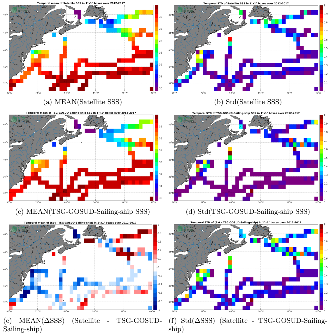
Figure 6: Temporal mean (left) and Std (right) of SSS from SMOS L3 v2 - Monthly - 0.25 Deg (CATDS-CECOS-IFREMER) (top), TSG-GOSUD-Sailing-ship (middle), and of \Delta SSS (Satellite - TSG-GOSUD-Sailing-ship). Only match-up pairs are used to generate these maps.
