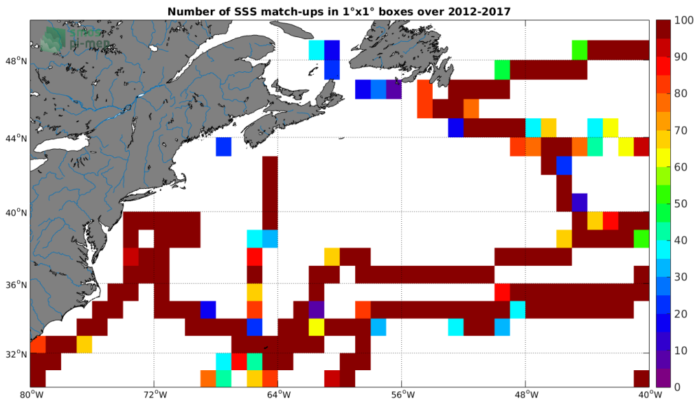
Figure 4: Number of SSS match-ups between TSG-GOSUD-Sailing-ship SSS and the SMOS-L3-CATDS-IFREMER-CECOS-V2-MONTHLY-0.25DEG SSS product for the Gulf Stream Pi-MEP region over 1^\circ \times 1^\circ boxes and for the full satellite product period.
