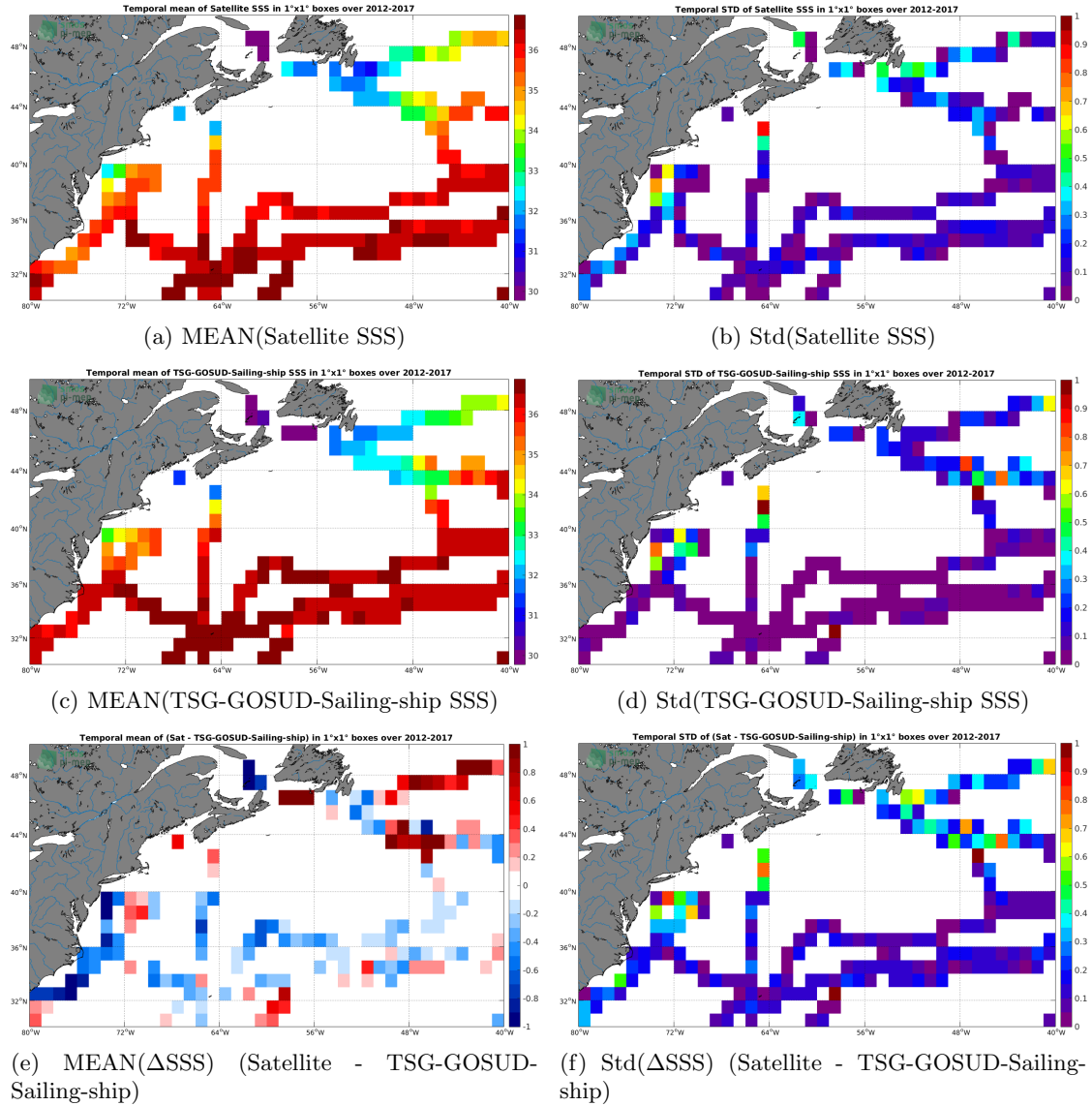
Figure 6: Temporal mean (left) and Std (right) of SSS from SMOS-L3-CATDS-IFREMER-CECOS-V2-MONTHLY-0.25DEG (top), TSG-GOSUD-Sailing-ship (middle), and of \Delta SSS (Satellite - TSG-GOSUD-Sailing-ship). Only match-up pairs are used to generate these maps.
