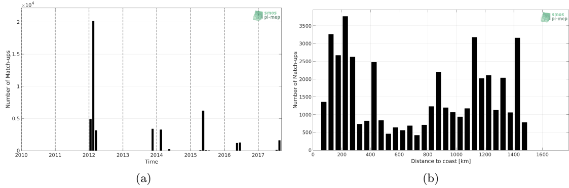
Figure 1: Number of match-ups between TSG-GOSUD-Sailing-ship and SMOS-L3-CATDS-IFREMER-CECOS-V2-MONTHLY-0.25DEG SSS as a function of time (a) and as function of the distance to coast (b) over the Gulf Stream Pi-MEP region and for the full satellite product period.
