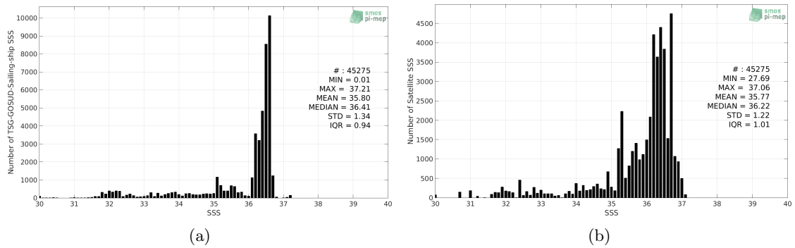
Figure 2: Histograms of SSS from TSG-GOSUD-Sailing-ship (a) and SMOS-L3-CATDS-IFREMER-CECOS-V2-MONTHLY-0.25DEG (b) considering all match-up pairs per bins of 0.1 over the Gulf Stream Pi-MEP region and for the full satellite product period.
