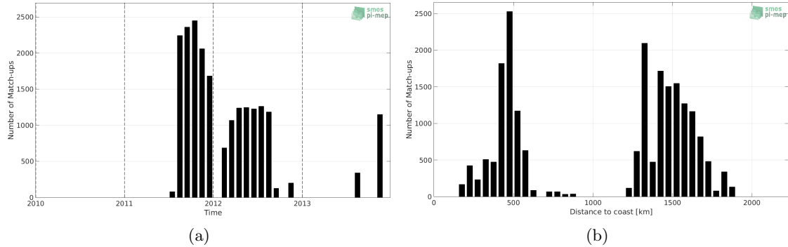
Figure 1: Number of match-ups between Surface drifters and SMOS L3 v2 - Monthly - 0.25 Deg (CATDS-CECOS-IFREMER) SSS as a function of time (a) and as function of the distance to coast (b) over the Gulf Stream Pi-MEP region and for the full satellite product period.
