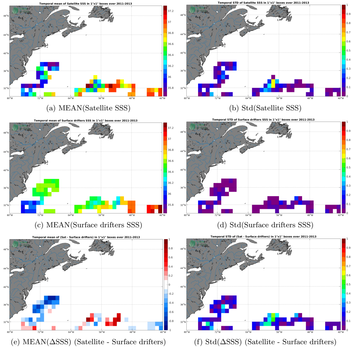
Figure 5: Temporal mean (left) and Std (right) of SSS from SMOS L3 v2 - Monthly - 0.25 Deg (CATDS-CECOS-IFREMER) (top), Surface drifters (middle), and of \Delta SSS (Satellite - Surface drifters). Only match-up pairs are used to generate these maps.
