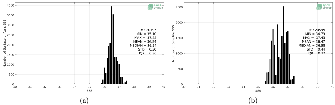
Figure 2: Histograms of SSS from Surface drifters (a) and SMOS L3 v2 - Monthly - 0.25 Deg (CATDS-CECOS-IFREMER) (b) considering all match-up pairs per bins of 0.1 over the Gulf Stream Pi-MEP region and for the full satellite product period.
