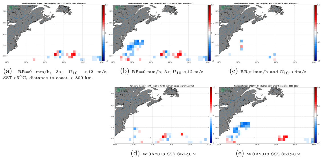
Figure 11: Temporal mean gridded over spatial boxes of size 1^{\circ}\times 1^{\circ} of \Delta\text{SSS} (SMOS L3 v2 - Monthly - 0.25 Deg (CATDS-CECOS-IFREMER) - Surface drifters) for 5 different subdatasets corresponding to:RR=0 mm/h, 3 < U_{10} < 12 m/s, SST >5^{\circ}\text{C} , distance to coast > 800 km (a), RR=0 mm/h, 3 < U_{10} < 12 m/s (b), RR >1 mm/h and U_{10} < 4 m/s (c), WOA2013 SSS Std <0.2 (d), WOA2013 SSS Std >0.2 (e).
