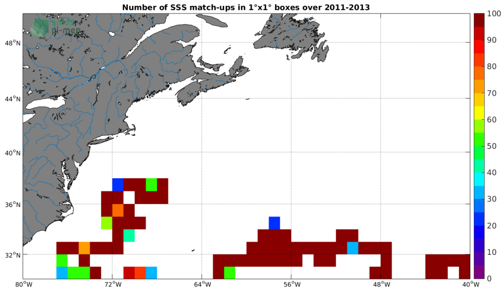
Figure 3: Number of SSS match-ups between Surface drifters SSS and the SMOS L3 v2 - Monthly - 0.25 Deg (CATDS-CECOS-IFREMER) SSS product for the Gulf Stream Pi-MEP region over 1^\circ \times 1^\circ boxes and for the full satellite product period.
