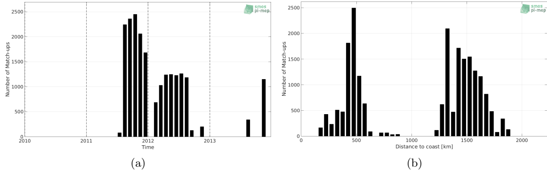
Figure 1: Number of match-ups between Surface drifters and SMOS-L3-CATDS-IFREMER-CECOS-V2-MONTHLY-0.25DEG SSS as a function of time (a) and as function of the distance to coast (b) over the Gulf Stream Pi-MEP region and for the full satellite product period.
