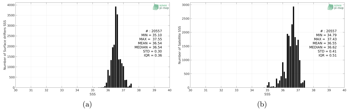
Figure 2: Histograms of SSS from Surface drifters (a) and SMOS-L3-CATDS-IFREMER-CECOS-V2-MONTHLY-0.25DEG (b) considering all match-up pairs per bins of 0.1 over the Gulf Stream Pi-MEP region and for the full satellite product period.
