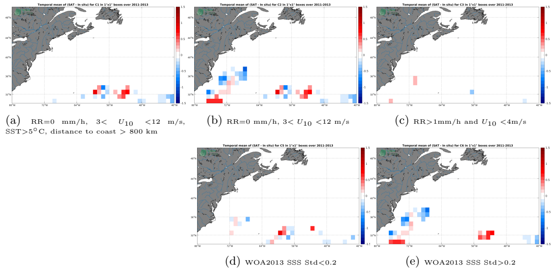
Figure 11: Temporal mean gridded over spatial boxes of size 1^\circ \times 1^\circ of \Delta SSS (SMOS-L3-CATDS-IFREMER-CECOS-V2-MONTHLY-0.25DEG - Surface drifters) for 5 different subdatasets corresponding to: RR=0 mm/h, 3 < U_{10} < 12 m/s, SST > 5^\circ C , distance to coast > 800 km (a), RR=0 mm/h, 3 < U_{10} < 12 m/s (b), RR > 1 mm/h and U_{10} < 4 m/s (c), WOA2013 SSS Std < 0.2 (d), WOA2013 SSS Std > 0.2 (e).
