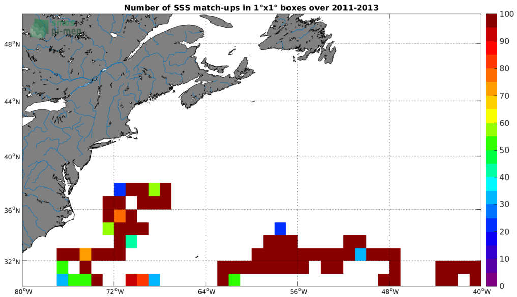
Figure 3: Number of SSS match-ups between Surface drifters SSS and the SMOS-L3-CATDS-IFREMER-CECOS-V2-MONTHLY-0.25DEG SSS product for the Gulf Stream Pi-MEP region over 1°x1° boxes and for the full satellite product period.
