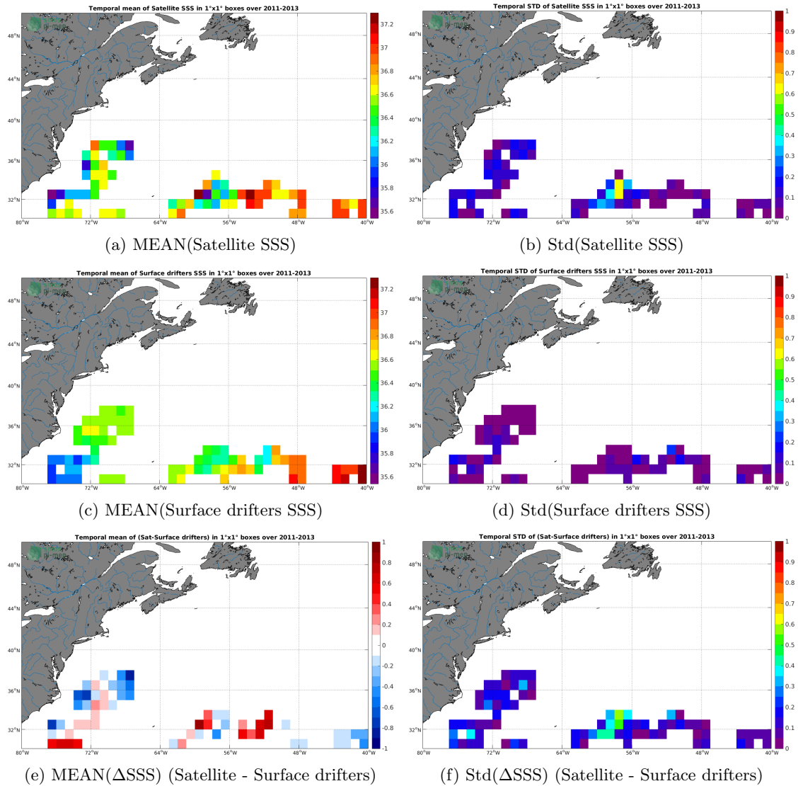
Figure 5: Temporal mean (left) and Std (right) of SSS from SMOS-L3-CATDS-IFREMER-CECOS-V2-MONTHLY-0.25DEG (top), Surface drifters (middle), and of \Delta SSS (Satellite - Surface drifters). Only match-up pairs are used to generate these maps.
