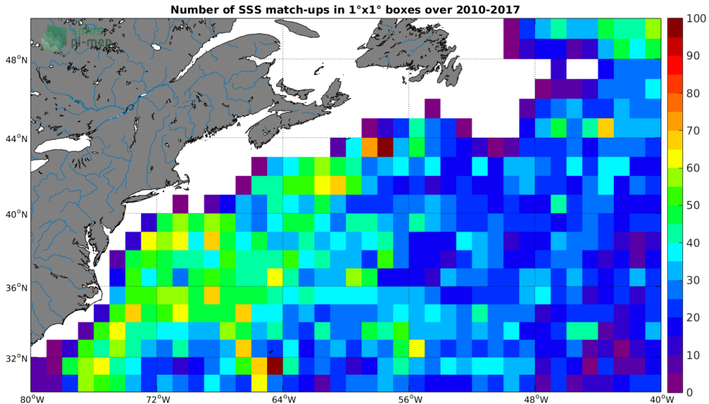
Figure 4: Number of SSS match-ups between Argos SSS and the SMOS SSS L3 v2 - Monthly - 0.25 Deg (CATDS-CECOS-IFREMER) SSS product for the Gulf Stream Pi-MEP region over 1^\circ \times 1^\circ boxes and for the full satellite product period.
