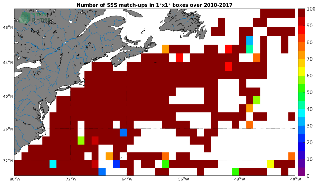
Figure 4: Number of SSS match-ups between TSG (SAMOS) SSS and the SMOS SSS L3 v2 - Daily - 0.5 Deg (CATDS-CECOS-IFREMER) SSS product for the Gulf Stream Pi-MEP region over 1^\circ \times 1^\circ boxes and for the full satellite product period.
