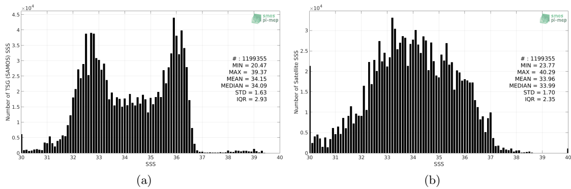
Figure 2: Histograms of SSS from TSG (SAMOS) (a) and SMOS SSS L3 v2 - Daily - 0.5 Deg (CATDS-CECOS-IFREMER) (b) considering all match-up pairs per bins of 0.1 over the Gulf Stream Pi-MEP region and for the full satellite product period.
