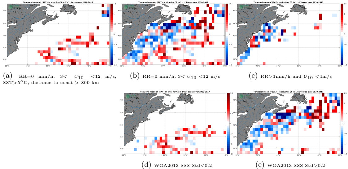
Figure 12: Temporal mean gridded over spatial boxes of size 1^{\circ}\times 1^{\circ} of \Delta\text{SSS} (SMOS SSS L3 v2 - Daily - 0.5 Deg (CATDS-CECOS-IFREMER) - TSG (SAMOS)) for 5 different subdatasets corresponding to:RR=0 mm/h, 3 < U_{10} < 12 m/s, SST >5^{\circ}\text{C} , distance to coast > 800 km (a), RR=0 mm/h, 3 < U_{10} < 12 m/s (b), RR >1 mm/h and U_{10} < 4 m/s (c), WOA2013 SSS Std <0.2 (d), WOA2013 SSS Std >0.2 (e).
