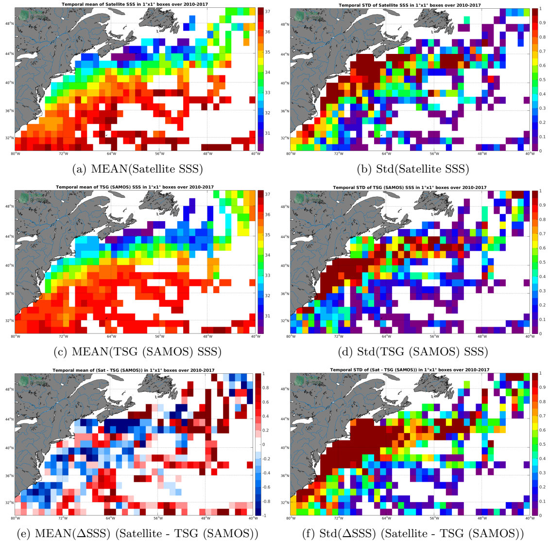
Figure 6: Temporal mean (left) and Std (right) of SSS from SMOS SSS L3 v2 - Daily - 0.5 Deg (CATDS-CECOS-IFREMER) (top), TSG (SAMOS) (middle), and of \Delta SSS (Satellite - TSG (SAMOS)). Only match-up pairs are used to generate these maps.
