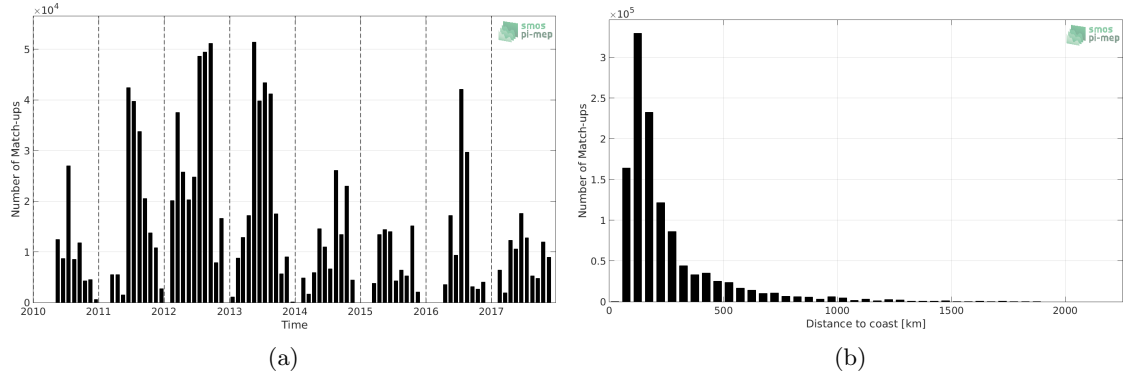
Figure 1: Number of match-ups between TSG (SAMOS) and SMOS SSS L3 v2 - Daily - 0.5 Deg (CATDS-CECOS-IFREMER) SSS as a function of time (a) and as function of the distance to coast (b) over the Gulf Stream Pi-MEP region and for the full satellite product period.
