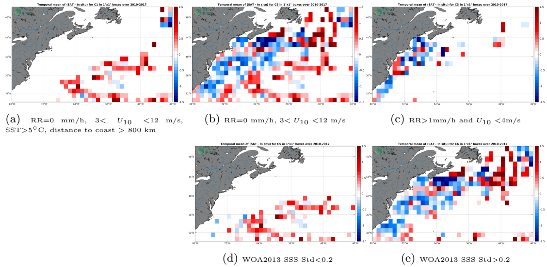
Figure 12: Temporal mean gridded over spatial boxes of size 1^\circ \times 1^\circ of \Delta SSS (SMOS L3 v2 - Daily - 0.5 Deg (CATDS-CECOS-IFREMER) - TSG-SAMOS) for 5 different subdatasets corresponding to:RR=0 mm/h, 3 < U_{10} < 12 m/s, SST >5^\circ C, distance to coast > 800 km (a), RR=0 mm/h, 3 < U_{10} < 12 m/s (b), RR >1 mm/h and U_{10} < 4 m/s (c), WOA2013 SSS Std <0.2 (d), WOA2013 SSS Std >0.2 (e).
