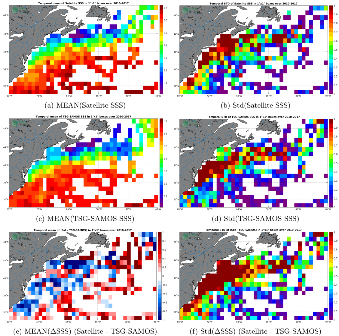
Figure 6: Temporal mean (left) and Std (right) of SSS from SMOS L3 v2 - Daily - 0.5 Deg (CATDS-CECOS-IFREMER) (top), TSG-SAMOS (middle), and of \Delta SSS (Satellite - TSG-SAMOS). Only match-up pairs are used to generate these maps.
