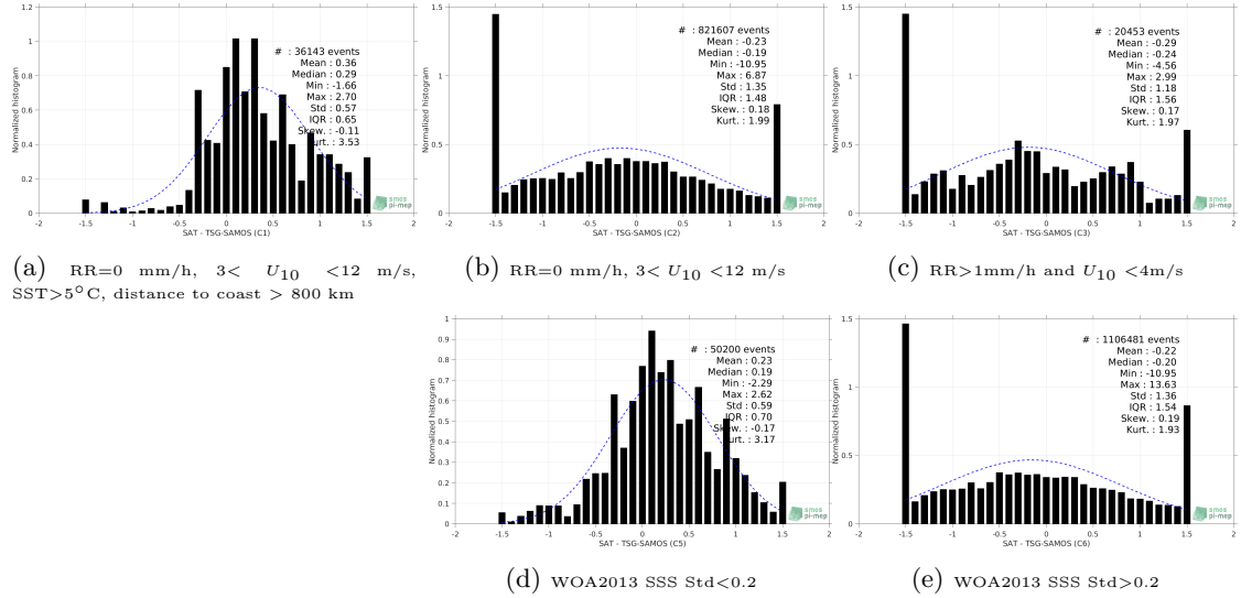
Figure 13: Normalized histogram of \Delta SSS (SMOS L3 v2 - Daily - 0.5 Deg (CATDS-CECOS-IFREMER) - TSG-SAMOS) for 5 different subdatasets corresponding to: RR=0 mm/h, 3 < U_{10} < 12 m/s, SST > 5°C, distance to coast > 800 km (a), RR=0 mm/h, 3 < U_{10} < 12 m/s (b), RR > 1mm/h and U_{10} < 4 m/s (c), WOA2013 SSS Std < 0.2 (d), WOA2013 SSS Std > 0.2 (e).
