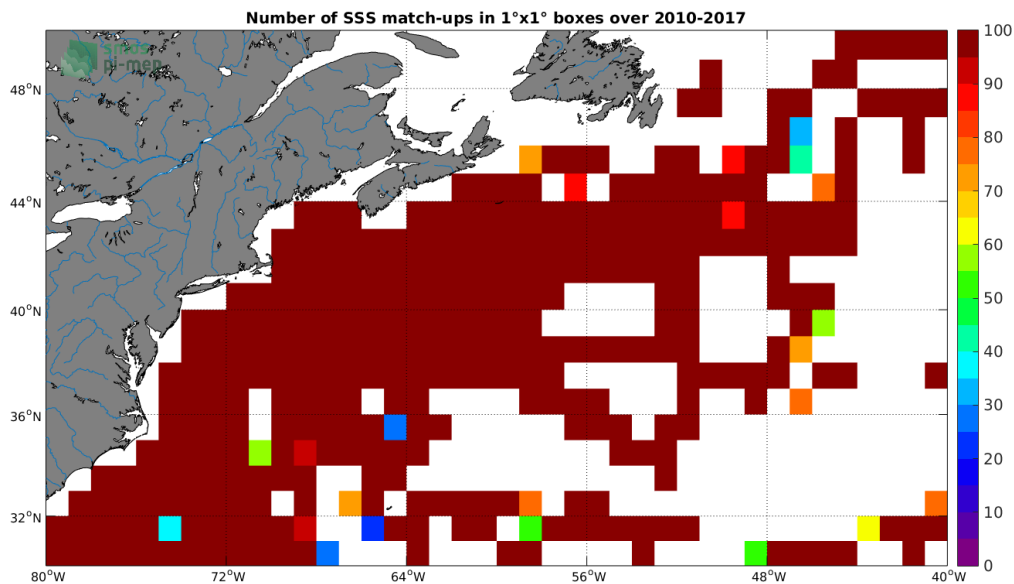
Figure 4: Number of SSS match-ups between TSG-SAMOS SSS and the SMOS L3 v2 - Daily - 0.5 Deg (CATDS-CECOS-IFREMER) SSS product for the Gulf Stream Pi-MEP region over 1^\circ \times 1^\circ boxes and for the full satellite product period.
