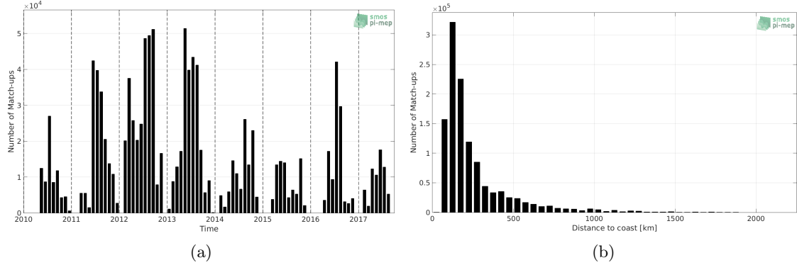
Figure 1: Number of match-ups between TSG-SAMOS and SMOS L3 v2 - Daily - 0.5 Deg (CATDS-CECOS-IFREMER) SSS as a function of time (a) and as function of the distance to coast (b) over the Gulf Stream Pi-MEP region and for the full satellite product period.
