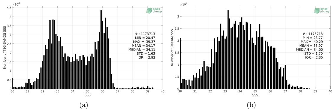
Figure 2: Histograms of SSS from TSG-SAMOS (a) and SMOS L3 v2 - Daily - 0.5 Deg (CATDS-CECOS-IFREMER) (b) considering all match-up pairs per bins of 0.1 over the Gulf Stream Pi-MEP region and for the full satellite product period.
