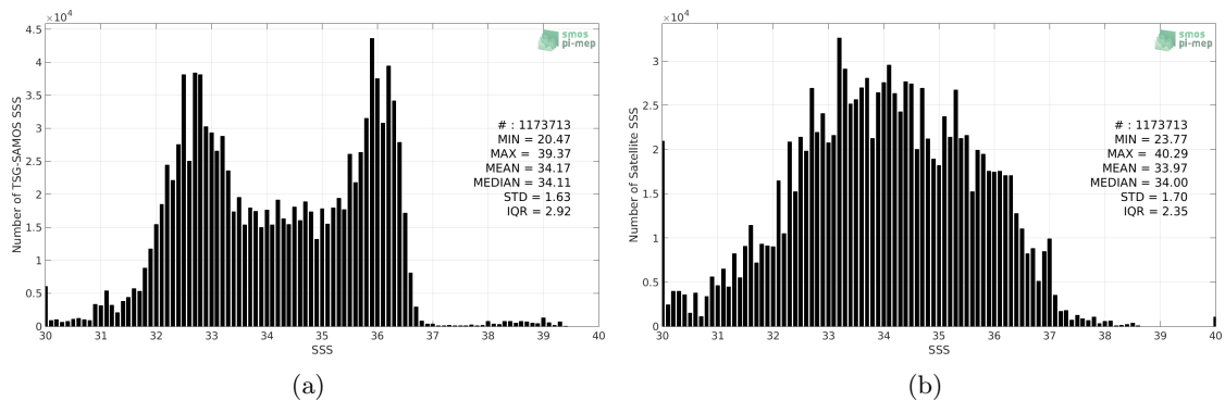
Figure 2: Histograms of SSS from TSG-SAMOS (a) and SMOS-L3-CATDS-CECOS-IFREMER-V2-1DAY-0.5DEG (b) considering all match-up pairs per bins of 0.1 over the Gulf Stream Pi-MEP region and for the full satellite product period.
