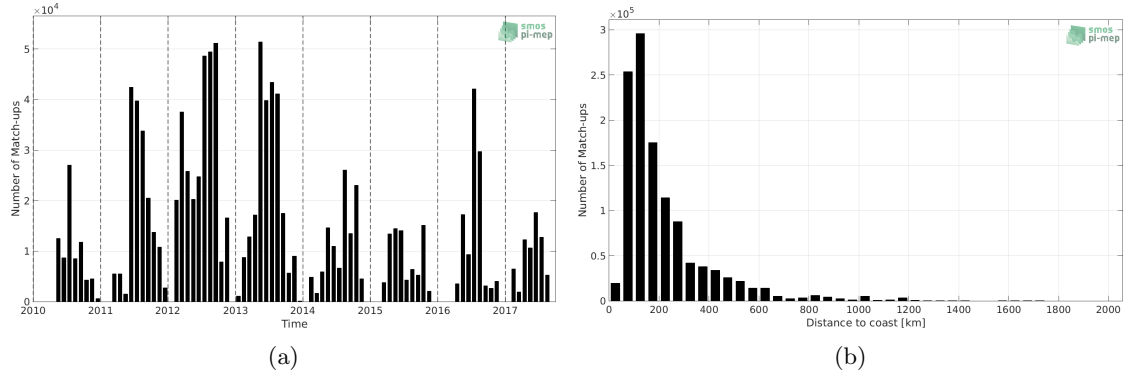
Figure 1: Number of match-ups between TSG-SAMOS and SMOS-L3-CATDS-CECOS-IFREMER-V2-1DAY-0.5DEG SSS as a function of time (a) and as function of the distance to coast (b) over the Gulf Stream Pi-MEP region and for the full satellite product period.
