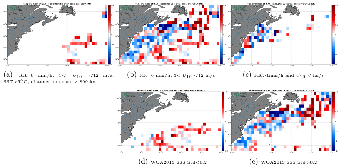
Figure 12: Temporal mean gridded over spatial boxes of size 1^\circ \times 1^\circ of \Delta SSS (SMOS-L3-CATDS-CECOS-IFREMER-V2-1DAY-0.5DEG - TSG-SAMOS) for 5 different subdatasets corresponding to:RR=0 mm/h, 3 < U_{10} < 12 m/s, SST >5^\circ C, distance to coast > 800 km (a), RR=0 mm/h, 3 < U_{10} < 12 m/s (b), RR >1 mm/h and U_{10} < 4 m/s (c), WOA2013 SSS Std <0.2 (d), WOA2013 SSS Std >0.2 (e).
