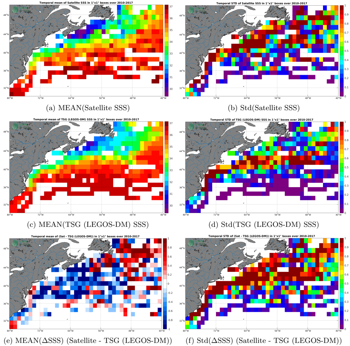
Figure 6: Temporal mean (left) and Std (right) of SSS from SMOS SSS L3 v2 - Daily - 0.5 Deg (CATDS-CECOS-IFREMER) (top), TSG (LEGOS-DM) ( in situ ) dataset (middle), and of \Delta SSS (Satellite - TSG (LEGOS-DM)). Only match-up pairs are used to generate these maps.
