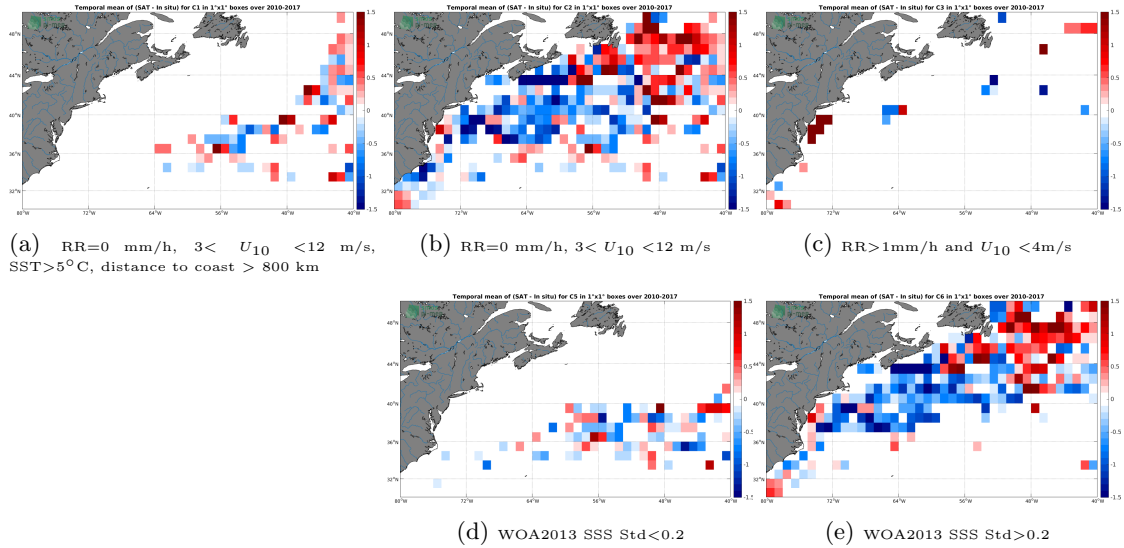
Figure 12: Temporal mean gridded over spatial boxes of size 1^{\circ}\times 1^{\circ} of \Delta\text{SSS} (SMOS SSS L3 v2 - Daily - 0.5 Deg (CATDS-CECOS-IFREMER) - TSG (LEGOS-DM)) for 5 different subdatasets corresponding to:RR=0 mm/h, 3 < U_{10} < 12 m/s, SST >5^{\circ}\text{C} , distance to coast > 800 km (a), RR=0 mm/h, 3 < U_{10} < 12 m/s (b), RR >1 mm/h and U_{10} < 4 m/s (c), WOA2013 SSS Std <0.2 (d), WOA2013 SSS Std >0.2 (e).
