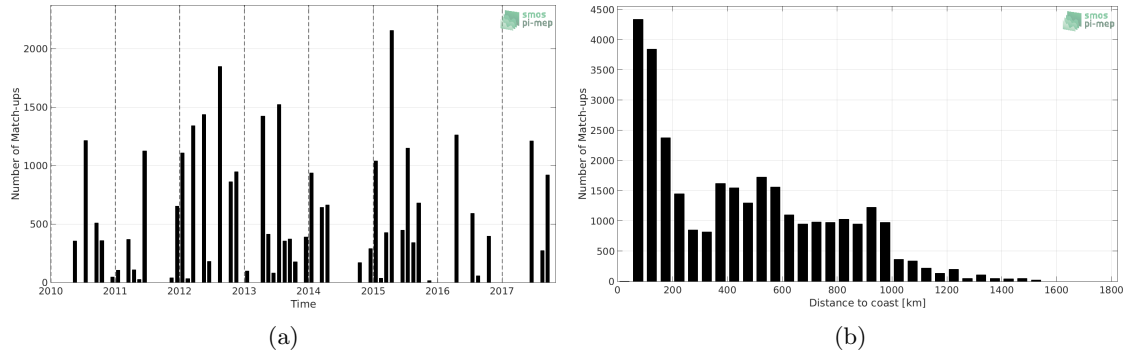
Figure 1: Number of match-ups between TSG (LEGOS-DM) and SMOS SSS L3 v2 - Daily - 0.5 Deg (CATDS-CECOS-IFREMER) SSS as a function of time (a) and as function of the distance to coast (b) over the Gulf Stream Pi-MEP region and for the full satellite product period.
