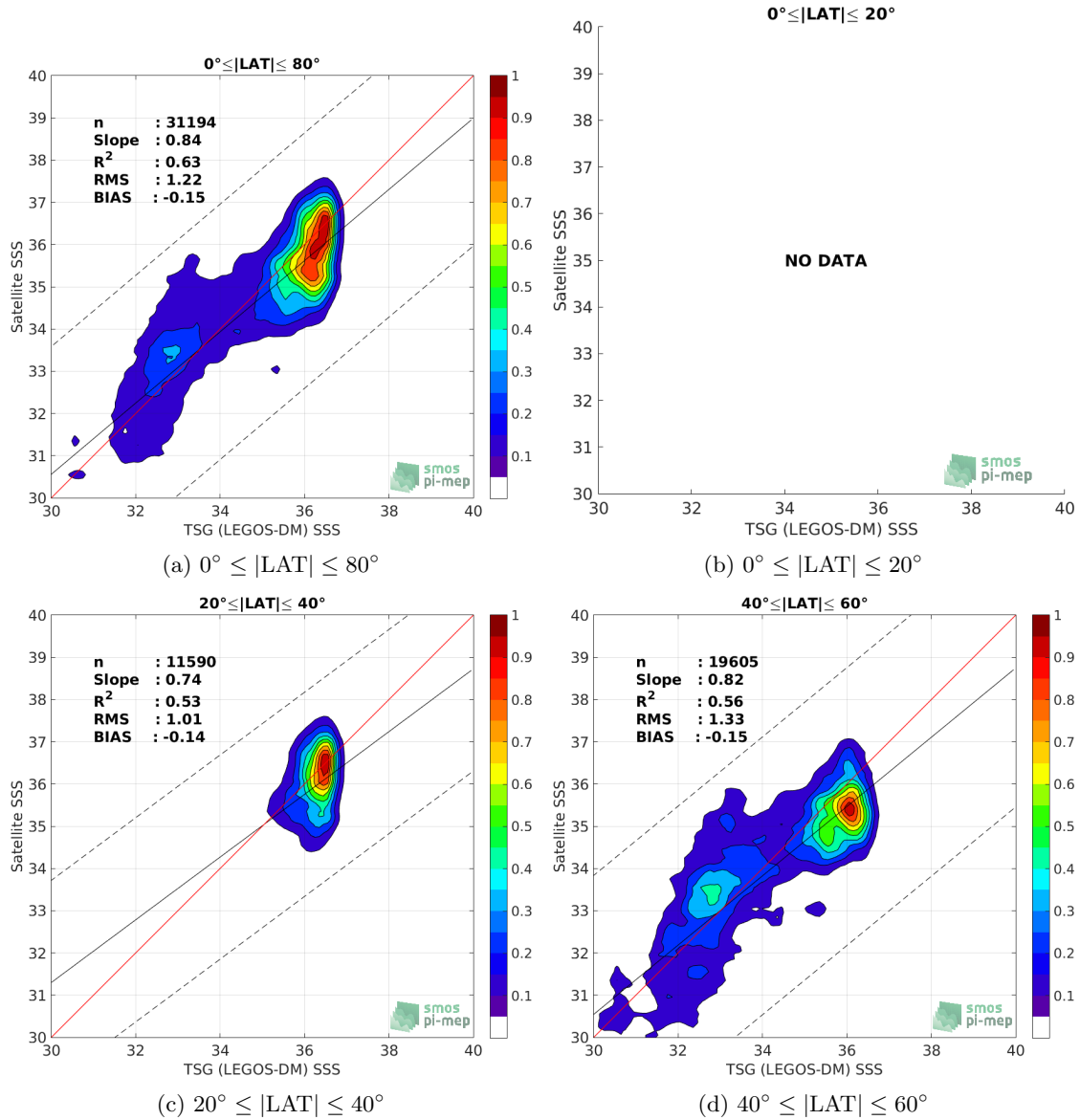
Figure 9: Contour maps of the concentration of SMOS SSS L3 v2 - Daily - 0.5 Deg (CATDS-CECOS-IFREMER) SSS ( y -axis) versus TSG (LEGOS-DM) SSS ( x -axis) at match-up pairs for different latitude bands. For each plot, the red line shows x=y . The black thin and dashed lines indicate a linear fit through the data cloud and the \pm 95\% confidence levels, respectively. The number match-up pairs n , the slope and R^2 coefficient of the linear fit, the root mean square (RMS) and the mean bias between satellite and in situ data are indicated for each latitude band in each plots.
