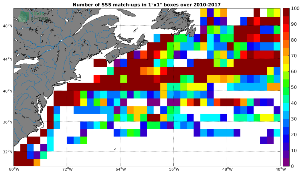
Figure 4: Number of SSS match-ups between TSG (LEGOS-DM) SSS and the SMOS SSS L3 v2 - Daily - 0.5 Deg (CATDS-CECOS-IFREMER) SSS product for the Gulf Stream Pi-MEP region over 1^\circ \times 1^\circ boxes and for the full satellite product period.
