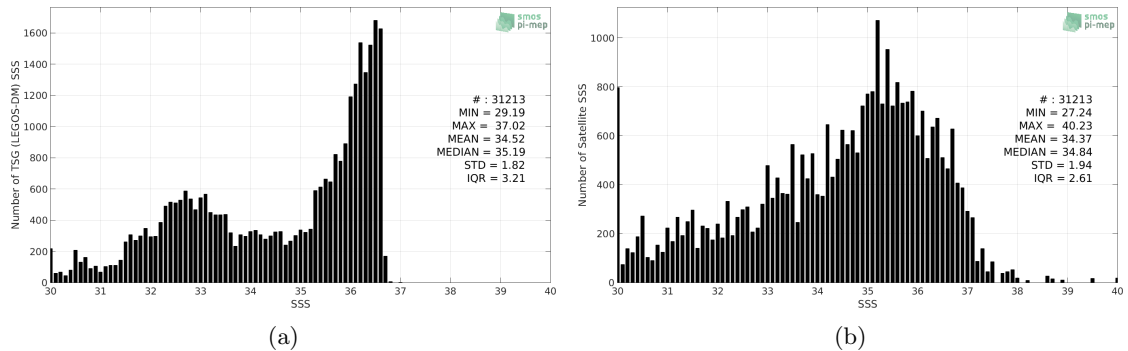
Figure 2: Histograms of SSS from TSG (LEGOS-DM) (a) and SMOS SSS L3 v2 - Daily - 0.5 Deg (CATDS-CECOS-IFREMER) (b) considering all match-up pairs per bins of 0.1 over the Gulf Stream Pi-MEP region and for the full satellite product period.
