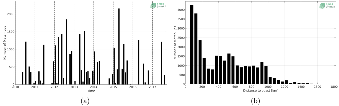
Figure 1: Number of match-ups between TSG-LEGOS-DM and SMOS L3 v2 - Daily - 0.5 Deg (CATDS-CECOS-IFREMER) SSS as a function of time (a) and as function of the distance to coast (b) over the Gulf Stream Pi-MEP region and for the full satellite product period.
