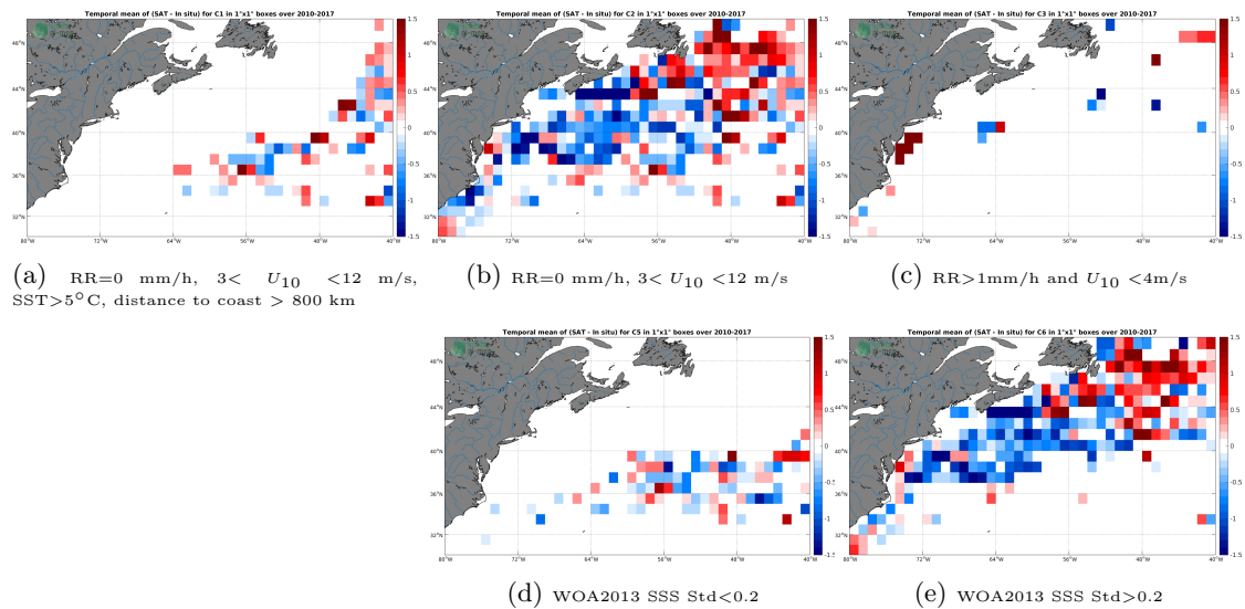
Figure 12: Temporal mean gridded over spatial boxes of size 1^{\circ}\times 1^{\circ} of \Delta\text{SSS} (SMOS L3 v2 - Daily - 0.5 Deg (CATDS-CECOS-IFREMER) - TSG-LEGOS-DM) for 5 different subdatasets corresponding to:RR=0 mm/h, 3 < U_{10} < 12 m/s, SST >5^{\circ}\text{C} , distance to coast > 800 km (a), RR=0 mm/h, 3 < U_{10} < 12 m/s (b), RR >1 mm/h and U_{10} < 4 m/s (c), WOA2013 SSS Std <0.2 (d), WOA2013 SSS Std >0.2 (e).
