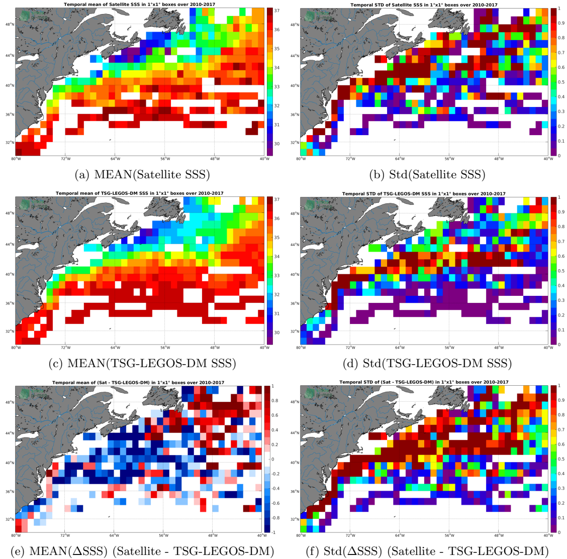
Figure 6: Temporal mean (left) and Std (right) of SSS from SMOS L3 v2 - Daily - 0.5 Deg (CATDS-CECOS-IFREMER) (top), TSG-LEGOS-DM (middle), and of \Delta SSS (Satellite - TSG-LEGOS-DM). Only match-up pairs are used to generate these maps.
