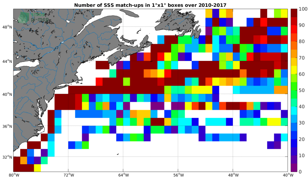
Figure 4: Number of SSS match-ups between TSG-LEGOS-DM SSS and the SMOS L3 v2 - Daily - 0.5 Deg (CATDS-CECOS-IFREMER) SSS product for the Gulf Stream Pi-MEP region over 1^\circ \times 1^\circ boxes and for the full satellite product period.
