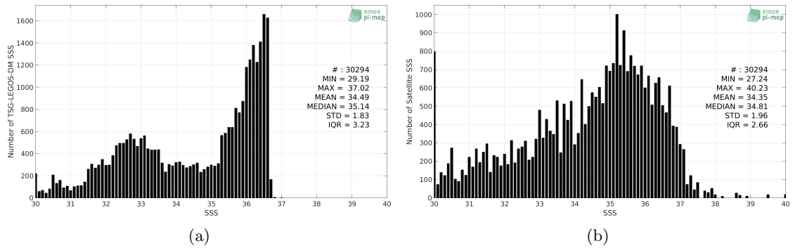
Figure 2: Histograms of SSS from TSG-LEGOS-DM (a) and SMOS L3 v2 - Daily - 0.5 Deg (CATDS-CECOS-IFREMER) (b) considering all match-up pairs per bins of 0.1 over the Gulf Stream Pi-MEP region and for the full satellite product period.
