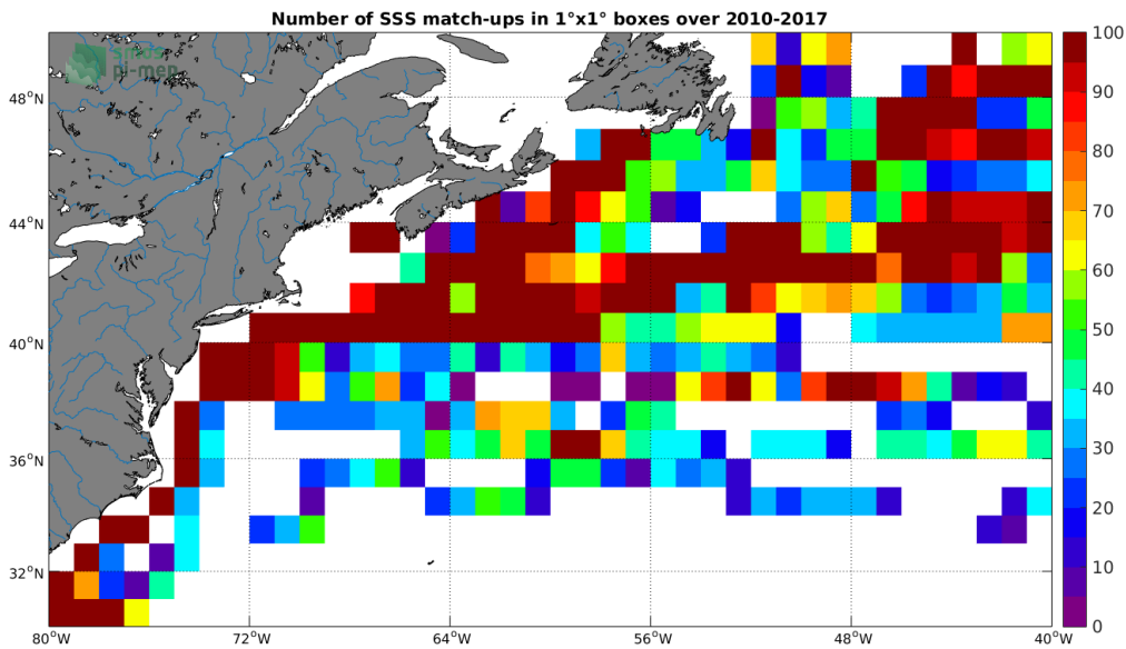
Figure 4: Number of SSS match-ups between TSG-LEGOS-DM SSS and the SMOS-L3-CATDS-CECOS-IFREMER-V2-1DAY-0.5DEG SSS product for the Gulf Stream Pi-MEP region over 1^\circ \times 1^\circ boxes and for the full satellite product period.
