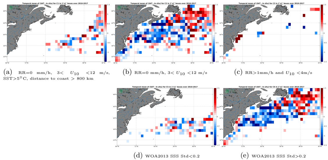
Figure 12: Temporal mean gridded over spatial boxes of size 1^\circ \times 1^\circ of \Delta SSS (SMOS-L3-CATDS-CECOS-IFREMER-V2-1DAY-0.5DEG - TSG-LEGOS-DM) for 5 different subdatasets corresponding to:RR=0 mm/h, 3 < U_{10} < 12 m/s, SST >5^\circ C, distance to coast > 800 km (a), RR=0 mm/h, 3 < U_{10} < 12 m/s (b), RR >1 mm/h and U_{10} < 4 m/s (c), WOA2013 SSS Std <0.2 (d), WOA2013 SSS Std >0.2 (e).
