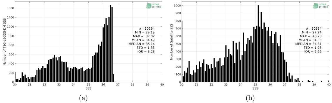
Figure 2: Histograms of SSS from TSG-LEGOS-DM (a) and SMOS-L3-CATDS-CECOS-IFREMER-V2-1DAY-0.5DEG (b) considering all match-up pairs per bins of 0.1 over the Gulf Stream Pi-MEP region and for the full satellite product period.
