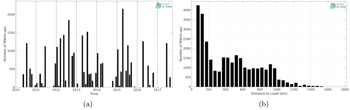
Figure 1: Number of match-ups between TSG-LEGOS-DM and SMOS-L3-CATDS-CECOS-IFREMER-V2-1DAY-0.5DEG SSS as a function of time (a) and as function of the distance to coast (b) over the Gulf Stream Pi-MEP region and for the full satellite product period.
