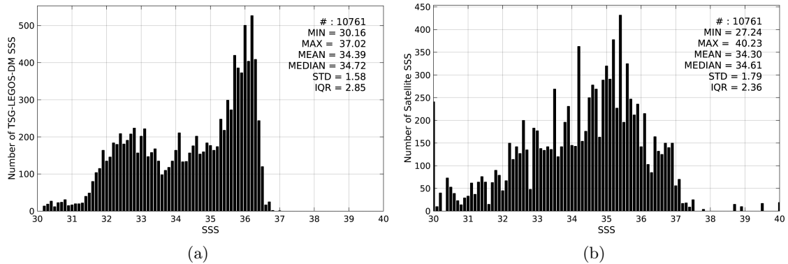
Figure 2: Histograms of SSS from TSG-LEGOS-DM (a) and SMOS-L3-CATDS-CECOS-IFREMER-V2-1DAY-0.5deg (b) considering all match-up pairs per bins of 0.1 over the Gulf Stream Pi-MEP region and for the full satellite product period.
