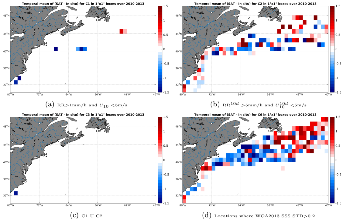
Figure 12: Temporal mean gridded over spatial boxes of size 1^\circ \times 1^\circ of \Delta SSS (SMOS-L3-CATDS-CECOS-IFREMER-V2-1DAY-0.5deg - TSG-LEGOS-DM) for 4 different subdatasets corresponding to: RR > 1mm/h and U_{10} < 5 m/s (a), RR^{10d} > 5 mm/h and U_{10}^{10d} < 5 m/s (b), C1 U C2 (c), Locations where WOA2013 SSS STD > 0.2 (d).
