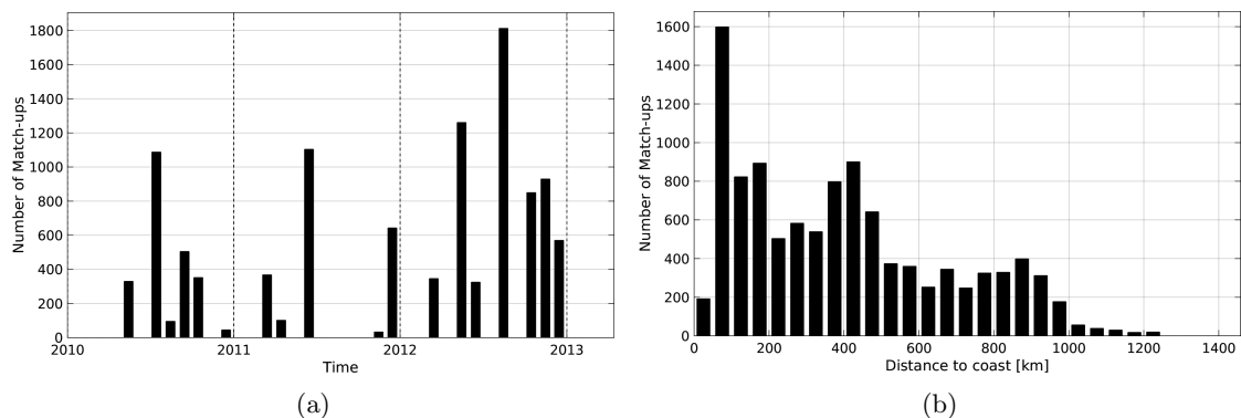
Figure 1: Number of match-ups between TSG-LEGOS-DM and SMOS-L3-CATDS-CECOS-IFREMER-V2-1DAY-0.5deg SSS as a function of time (a) and as function of the distance to coast (b) over the Gulf Stream Pi-MEP region and for the full satellite product period.
