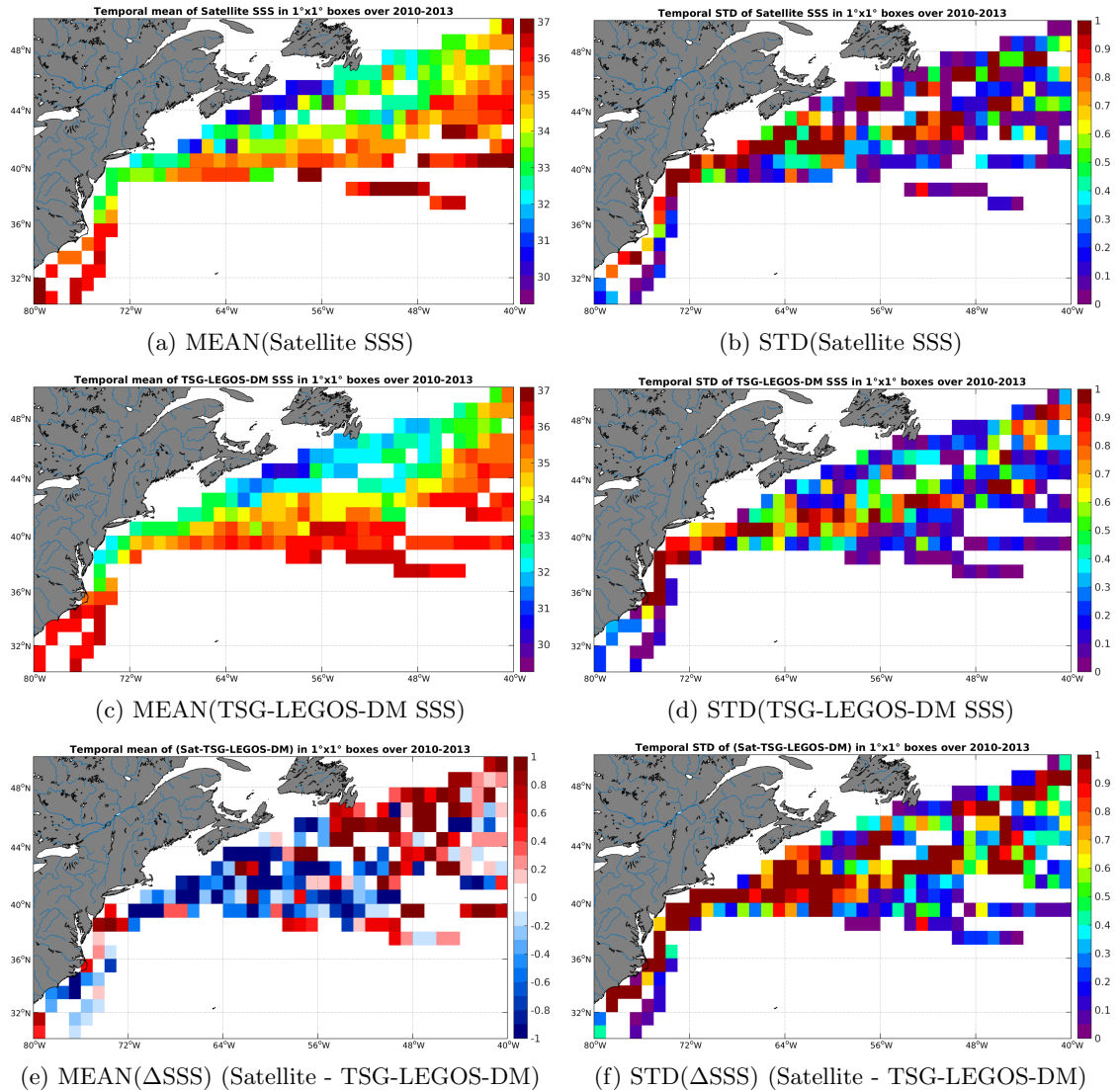
Figure 6: Temporal mean (left) and STD (right) of SSS from SMOS-L3-CATDS-CECOS-IFREMER-V2-1DAY-0.5deg (top), TSG-LEGOS-DM (middle), and of \Delta SSS (Satellite - TSG-LEGOS-DM). Only match-up pairs are used to generate these maps.
