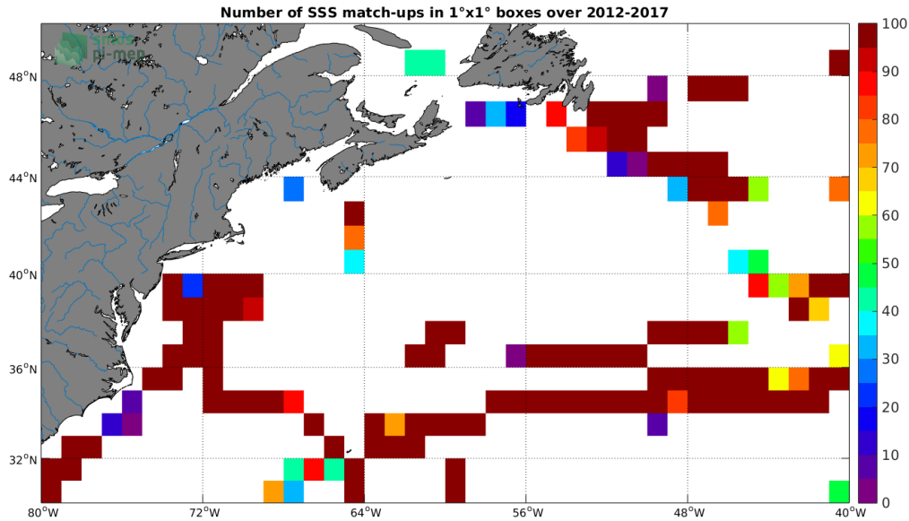
Figure 4: Number of SSS match-ups between TSG-GOSUD-Sailing-ship SSS and the SMOS L3 v2 - Daily - 0.5 Deg (CATDS-CECOS-IFREMER) SSS product for the Gulf Stream Pi-MEP region over 1^\circ \times 1^\circ boxes and for the full satellite product period.
