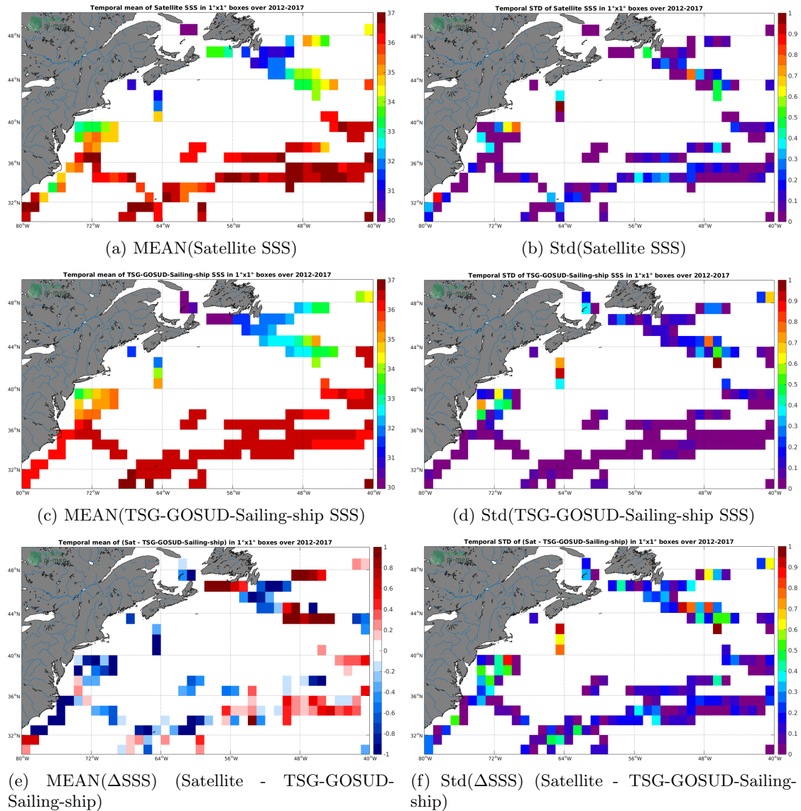
Figure 6: Temporal mean (left) and Std (right) of SSS from SMOS L3 v2 - Daily - 0.5 Deg (CATDS-CECOS-IFREMER) (top), TSG-GOSUD-Sailing-ship (middle), and of \Delta SSS (Satellite - TSG-GOSUD-Sailing-ship). Only match-up pairs are used to generate these maps.
