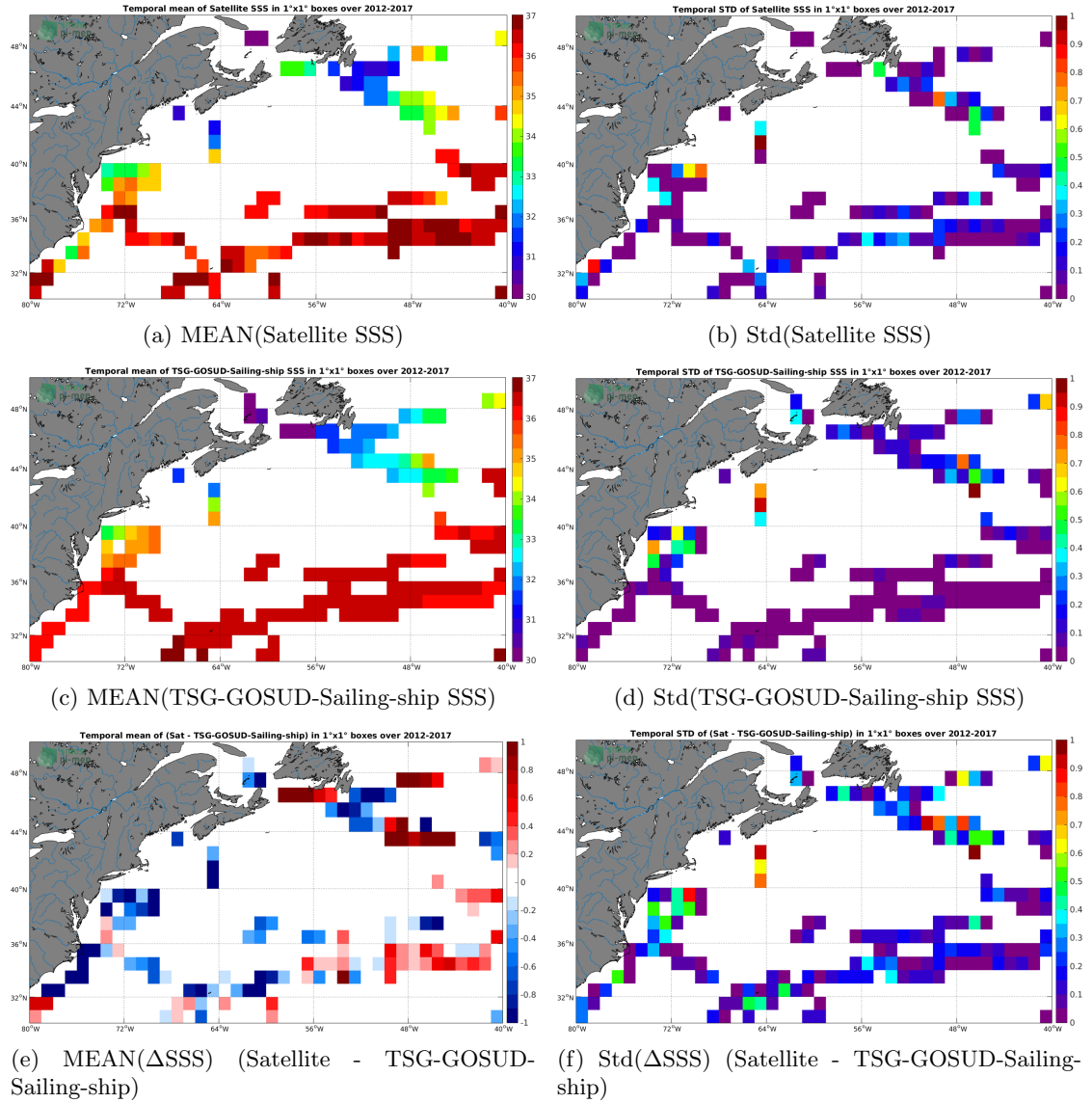
Figure 6: Temporal mean (left) and Std (right) of SSS from SMOS-L3-CATDS-CECOS-IFREMER-V2-1DAY-0.5DEG (top), TSG-GOSUD-Sailing-ship (middle), and of \Delta SSS (Satellite - TSG-GOSUD-Sailing-ship). Only match-up pairs are used to generate these maps.
