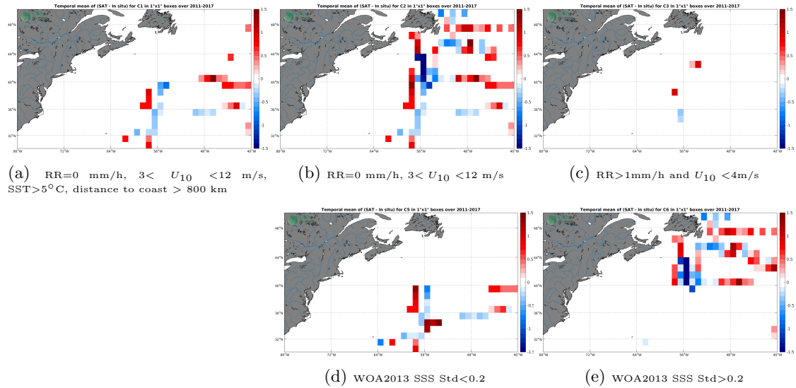
Figure 12: Temporal mean gridded over spatial boxes of size 1^{\circ}\times 1^{\circ} of \Delta SSS (SMOS L3 v2 - Daily - 0.5 Deg (CATDS-CECOS-IFREMER) - TSG-GOSUD-Research-vessel) for 5 different subdatasets corresponding to:RR=0 mm/h, 3 < U_{10} < 12 m/s, SST > 5^{\circ}\text{C} , distance to coast > 800 km (a), RR=0 mm/h, 3 < U_{10} < 12 m/s (b), RR > 1 mm/h and U_{10} < 4 m/s (c), WOA2013 SSS Std < 0.2 (d), WOA2013 SSS Std > 0.2 (e).
