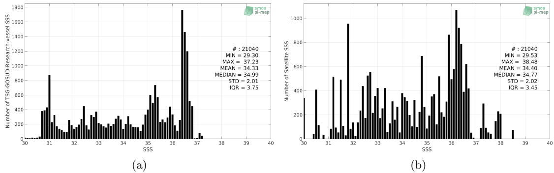
Figure 2: Histograms of SSS from TSG-GOSUD-Research-vessel (a) and SMOS L3 v2 - Daily - 0.5 Deg (CATDS-CECOS-IFREMER) (b) considering all match-up pairs per bins of 0.1 over the Gulf Stream Pi-MEP region and for the full satellite product period.
