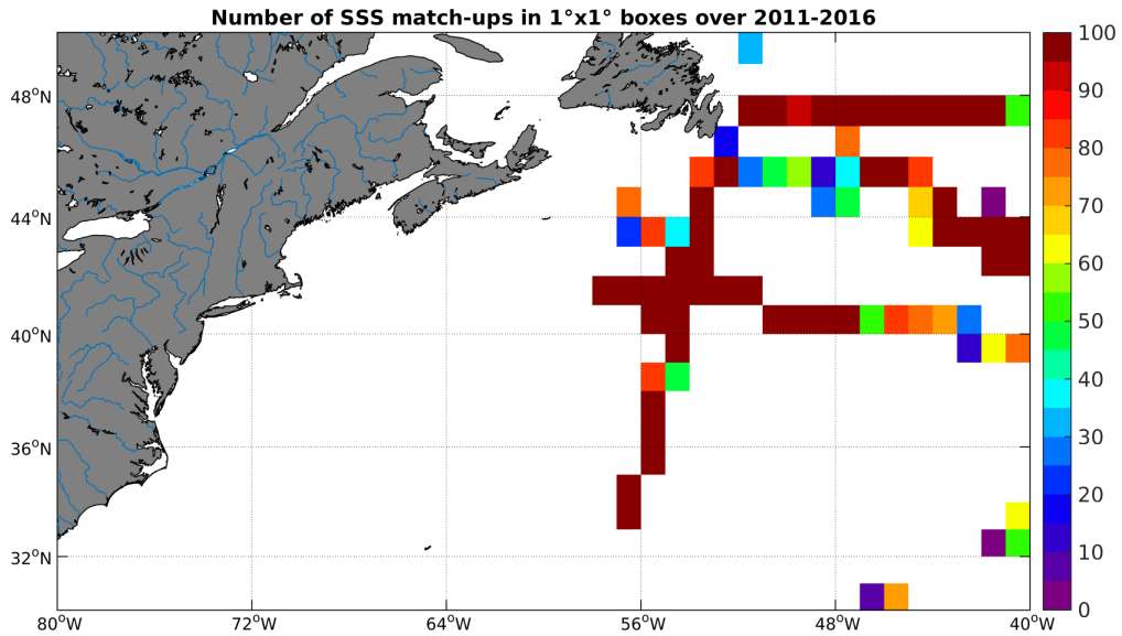
Figure 4: Number of SSS match-ups between TSG-GOSUD-Research-vessel SSS and the SMOS-L3-CATDS-CECOS-IFREMER-V2-1DAY-0.5deg SSS product for the Gulf Stream Pi-MEP region over 1^{\circ} \times 1^{\circ} boxes and for the full satellite product period.
