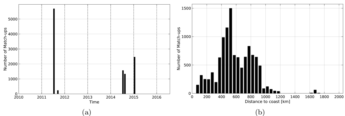
Figure 1: Number of match-ups between TSG-GOSUD-Research-vessel and SMOS-L3-CATDS-CECOS-IFREMER-V2-1DAY-0.5deg SSS as a function of time (a) and as function of the distance to coast (b) over the Gulf Stream Pi-MEP region and for the full satellite product period.
