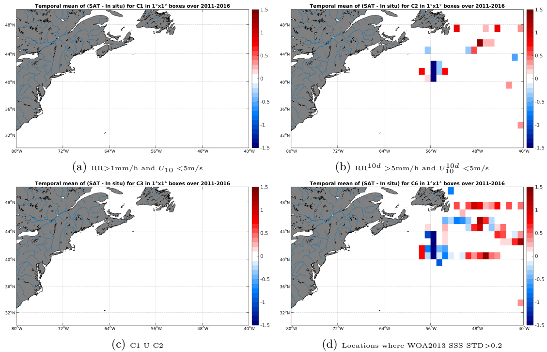
Figure 12: Temporal mean gridded over spatial boxes of size 1°x1° of \Delta SSS (SMOS-L3-CATDS-CECOS-IFREMER-V2-1DAY-0.5deg - TSG-GOSUD-Research-vessel) for 4 different subdatasets corresponding to:RR>1mm/h and U_{10} < 5m/s (a), RR^{10d} > 5mm/h and U_{10}^{10d} < 5m/s (b), C1 U C2 (c),Locations where WOA2013 SSS STD>0.2 (d).
