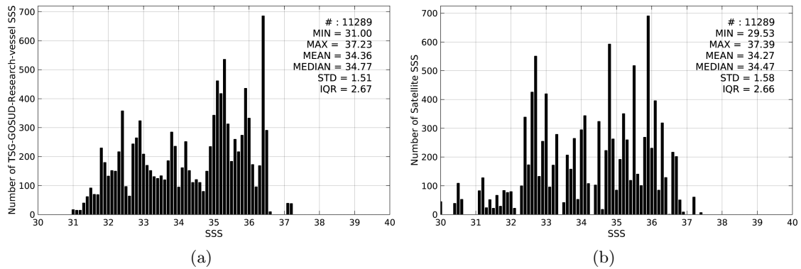
Figure 2: Histograms of SSS from TSG-GOSUD-Research-vessel (a) and SMOS-L3-CATDS-CECOS-IFREMER-V2-1DAY-0.5deg (b) considering all match-up pairs per bins of 0.1 over the Gulf Stream Pi-MEP region and for the full satellite product period.
