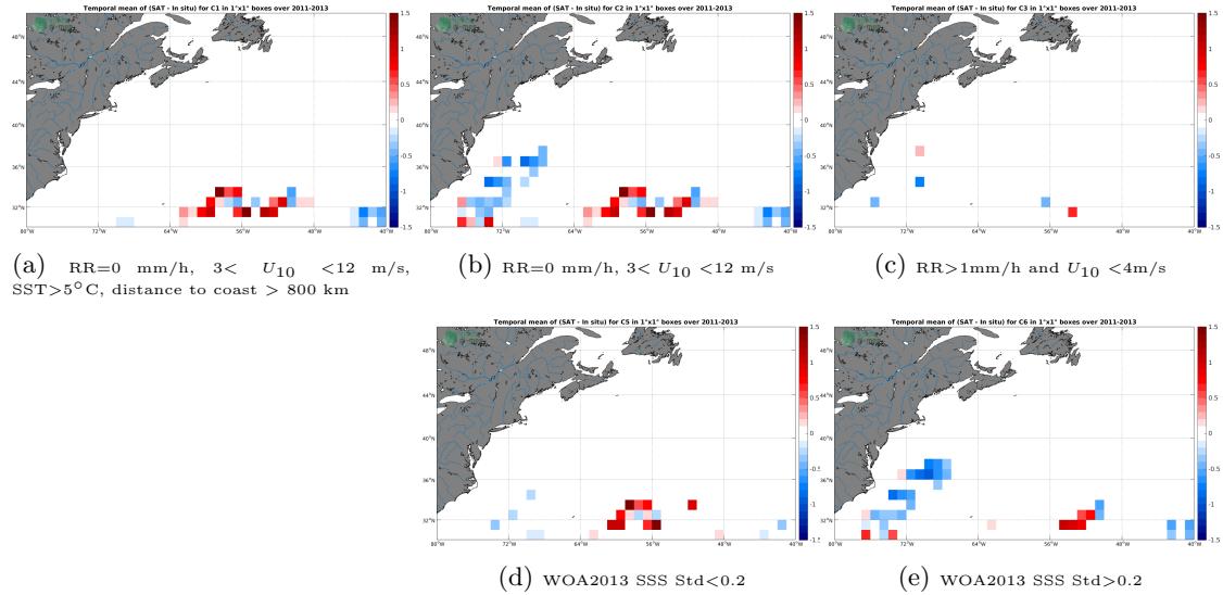
Figure 11: Temporal mean gridded over spatial boxes of size 1^{\circ}\times 1^{\circ} of \Delta\text{SSS} (SMOS SSS L3 v2 - Daily - 0.5 Deg (CATDS-CECOS-IFREMER) - Surface drifters) for 5 different subdatasets corresponding to:RR=0 mm/h, 3 < U_{10} < 12 m/s, SST >5^{\circ}\text{C} , distance to coast > 800 km (a), RR=0 mm/h, 3 < U_{10} < 12 m/s (b), RR >1 mm/h and U_{10} < 4 m/s (c), WOA2013 SSS Std <0.2 (d), WOA2013 SSS Std >0.2 (e).
