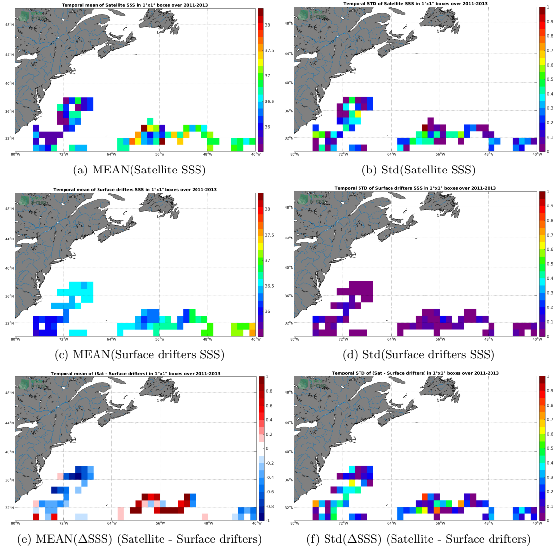
Figure 5: Temporal mean (left) and Std (right) of SSS from SMOS SSS L3 v2 - Daily - 0.5 Deg (CATDS-CECOS-IFREMER) (top), Surface drifters (middle), and of \Delta\text{SSS} (Satellite - Surface drifters). Only match-up pairs are used to generate these maps.
