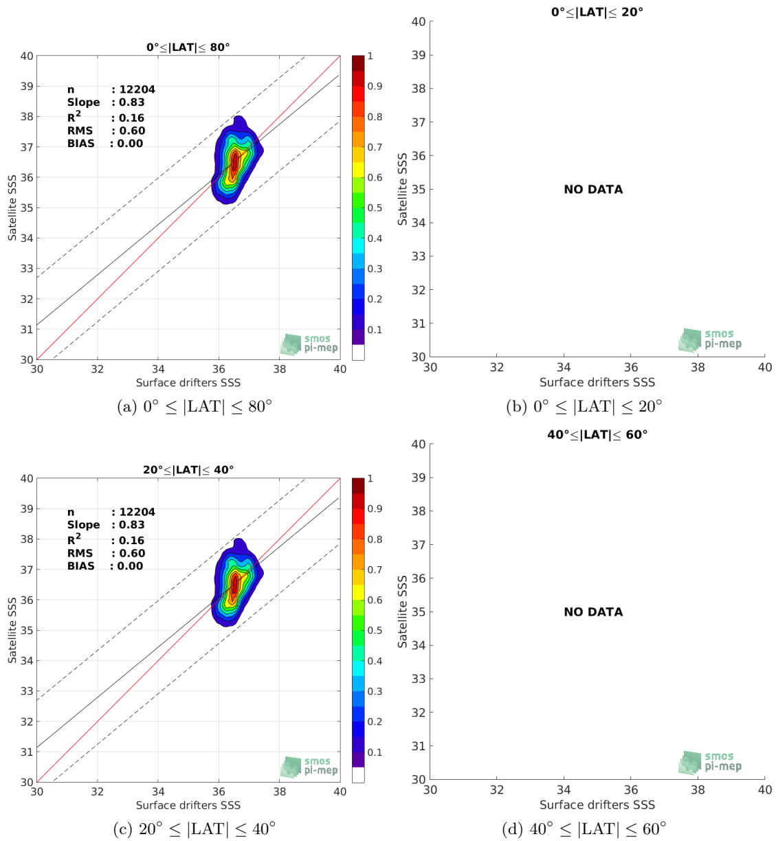
Figure 8: Contour maps of the concentration of SMOS SSS L3 v2 - Daily - 0.5 Deg (CATDS-CECOS-IFREMER) SSS (y-axis) versus Surface drifters SSS (x-axis) at match-up pairs for different latitude bands. For each plot, the red line shows x=y . The black thin and dashed lines indicate a linear fit through the data cloud and the \pm 95\% confidence levels, respectively. The number match-up pairs n , the slope and R^2 coefficient of the linear fit, the root mean square (RMS) and the mean bias between satellite and in situ data are indicated for each latitude band in each plots.
