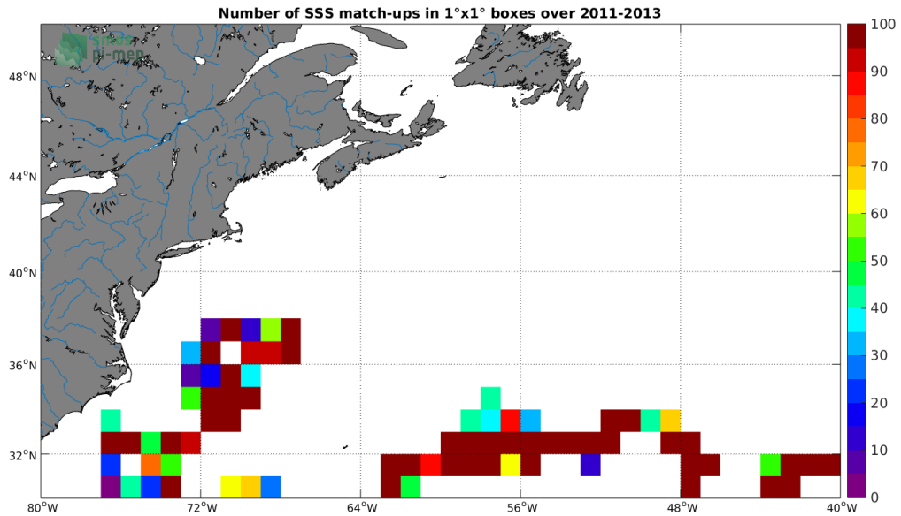
Figure 3: Number of SSS match-ups between Surface drifters SSS and the SMOS L3 v2 - Daily - 0.5 Deg (CATDS-CECOS-IFREMER) SSS product for the Gulf Stream Pi-MEP region over 1°x1° boxes and for the full satellite product period.
