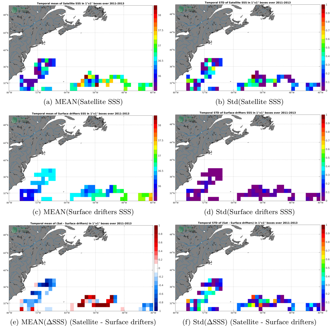
Figure 5: Temporal mean (left) and Std (right) of SSS from SMOS L3 v2 - Daily - 0.5 Deg (CATDS-CECOS-IFREMER) (top), Surface drifters (middle), and of \Delta SSS (Satellite - Surface drifters). Only match-up pairs are used to generate these maps.
