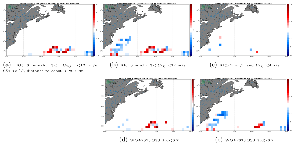
Figure 11: Temporal mean gridded over spatial boxes of size 1^{\circ}\times 1^{\circ} of \Delta\text{SSS} (SMOS L3 v2 - Daily - 0.5 Deg (CATDS-CECOS-IFREMER) - Surface drifters) for 5 different subdatasets corresponding to:RR=0 mm/h, 3 < U_{10} < 12 m/s, SST >5^{\circ}\text{C} , distance to coast > 800 km (a), RR=0 mm/h, 3 < U_{10} < 12 m/s (b), RR >1 mm/h and U_{10} < 4 m/s (c), WOA2013 SSS Std <0.2 (d), WOA2013 SSS Std >0.2 (e).
