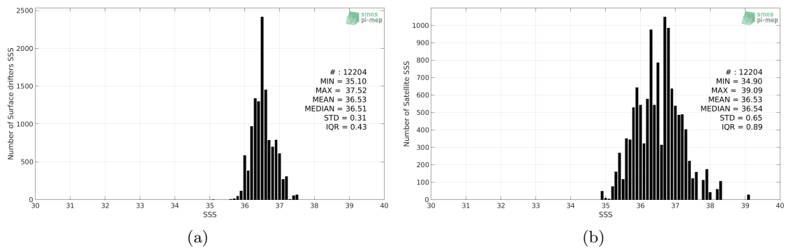
Figure 2: Histograms of SSS from Surface drifters (a) and SMOS L3 v2 - Daily - 0.5 Deg (CATDS-CECOS-IFREMER) (b) considering all match-up pairs per bins of 0.1 over the Gulf Stream Pi-MEP region and for the full satellite product period.
