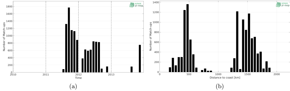
Figure 1: Number of match-ups between Surface drifters and SMOS L3 v2 - Daily - 0.5 Deg (CATDS-CECOS-IFREMER) SSS as a function of time (a) and as function of the distance to coast (b) over the Gulf Stream Pi-MEP region and for the full satellite product period.
