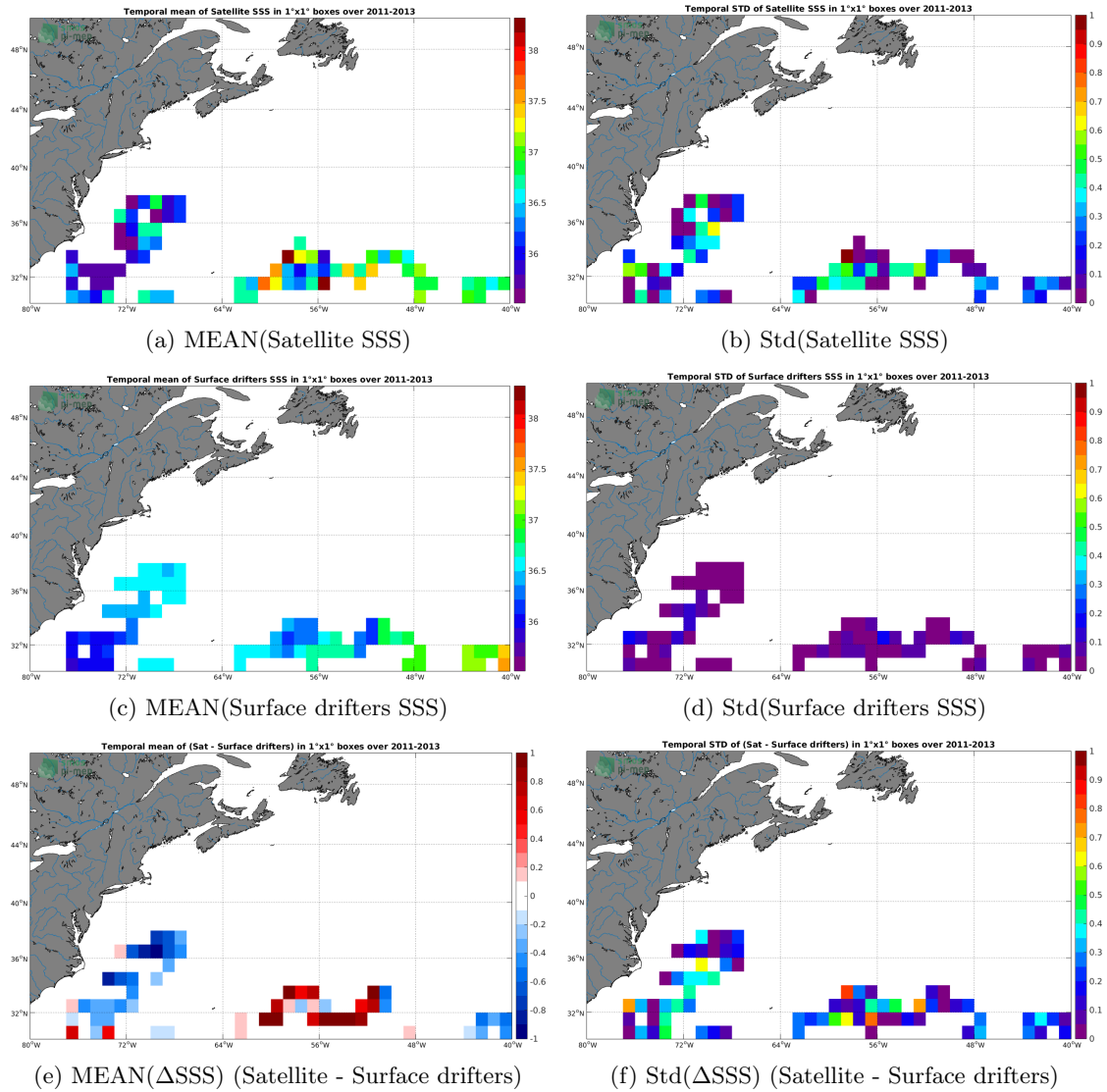
Figure 5: Temporal mean (left) and Std (right) of SSS from SMOS-L3-CATDS-CECOS-IFREMER-V2-1DAY-0.5DEG (top), Surface drifters (middle), and of \Delta SSS (Satellite - Surface drifters). Only match-up pairs are used to generate these maps.
