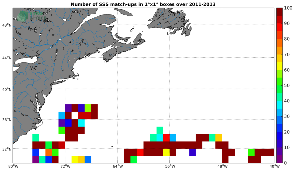
Figure 3: Number of SSS match-ups between Surface drifters SSS and the SMOS-L3-CATDS-CECOS-IFREMER-V2-1DAY-0.5DEG SSS product for the Gulf Stream Pi-MEP region over 1°x1° boxes and for the full satellite product period.
