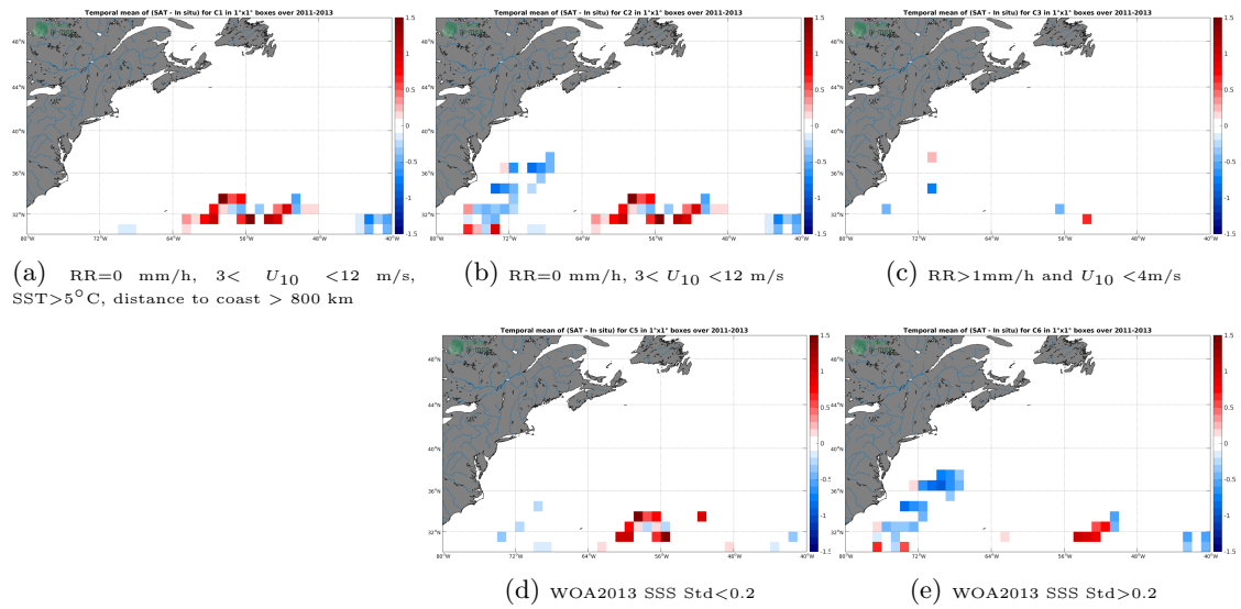
Figure 11: Temporal mean gridded over spatial boxes of size 1^\circ \times 1^\circ of \Delta SSS (SMOS-L3-CATDS-CECOS-IFREMER-V2-1DAY-0.5DEG - Surface drifters) for 5 different subdatasets corresponding to: RR=0 mm/h, 3 < U_{10} < 12 m/s, SST > 5^\circ C , distance to coast > 800 km (a), RR=0 mm/h, 3 < U_{10} < 12 m/s (b), RR > 1 mm/h and U_{10} < 4 m/s (c), WOA2013 SSS Std < 0.2 (d), WOA2013 SSS Std > 0.2 (e).
