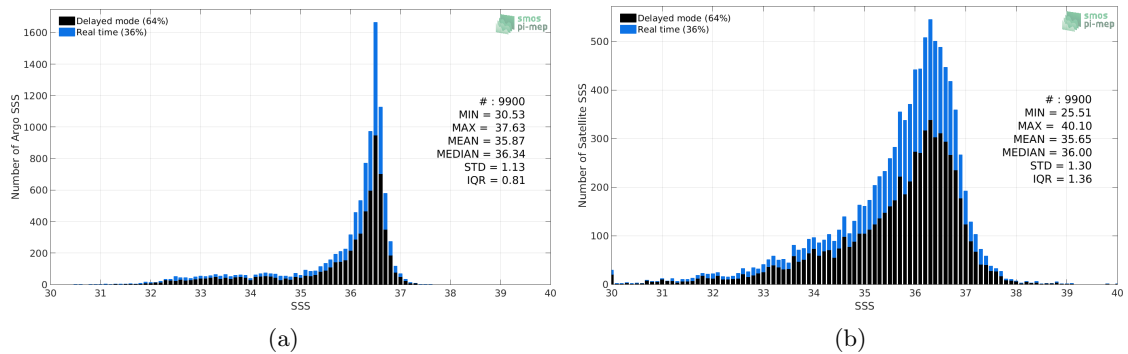
Figure 2: Histograms of SSS from Argo (a) and SMOS L3 v2 - Daily - 0.5 Deg (CATDS-CECOS-IFREMER) (b) considering all match-up pairs per bins of 0.1 over the Gulf Stream Pi-MEP region and for the full satellite product period.
