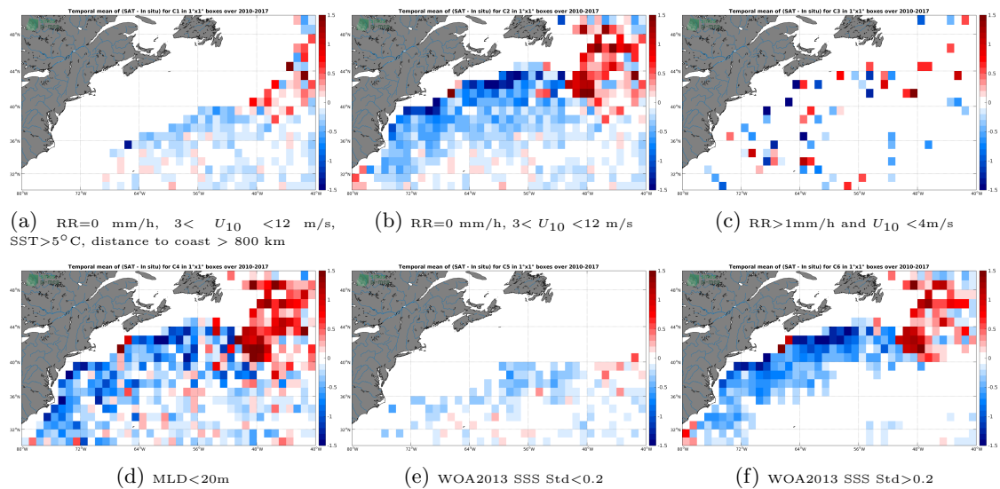
Figure 12: Temporal mean gridded over spatial boxes of size 1^\circ \times 1^\circ of \Delta SSS (SMOS L3 v2 - Daily - 0.5 Deg (CATDS-CECOS-IFREMER) - Argo) for 6 different subdatasets corresponding to:RR=0 mm/h, 3 < U_{10} < 12 m/s, SST >5^\circ C, distance to coast > 800 km (a), RR=0 mm/h, 3 < U_{10} < 12 m/s (b), RR >1 mm/h and U_{10} < 4 m/s (c),MLD <20 m (d),WOA2013 SSS Std <0.2 (e),WOA2013 SSS Std >0.2 (f).
