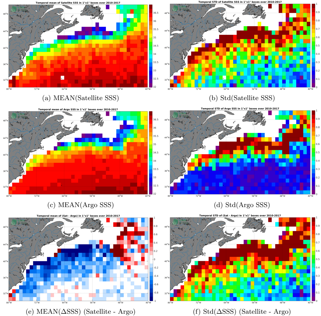
Figure 6: Temporal mean (left) and Std (right) of SSS from SMOS L3 v2 - Daily - 0.5 Deg (CATDS-CECOS-IFREMER) (top), Argo (middle), and of \Delta SSS (Satellite - Argo). Only match-up pairs are used to generate these maps.
