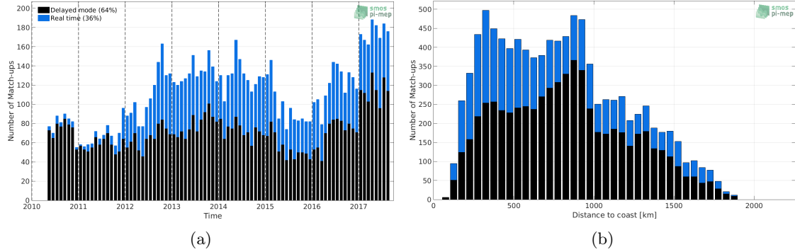
Figure 1: Number of match-ups between Argo and SMOS L3 v2 - Daily - 0.5 Deg (CATDS-CECOS-IFREMER) SSS as a function of time (a) and as function of the distance to coast (b) over the Gulf Stream Pi-MEP region and for the full satellite product period.
