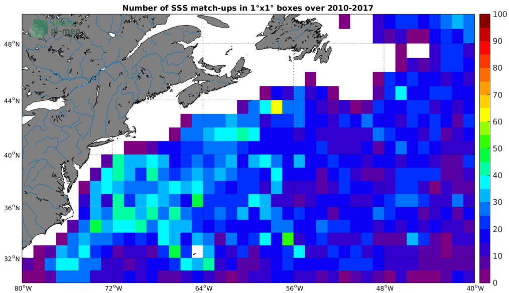
Figure 4: Number of SSS match-ups between Argo SSS and the SMOS L3 v2 - Daily - 0.5 Deg (CATDS-CECOS-IFREMER) SSS product for the Gulf Stream Pi-MEP region over 1^\circ \times 1^\circ boxes and for the full satellite product period.
