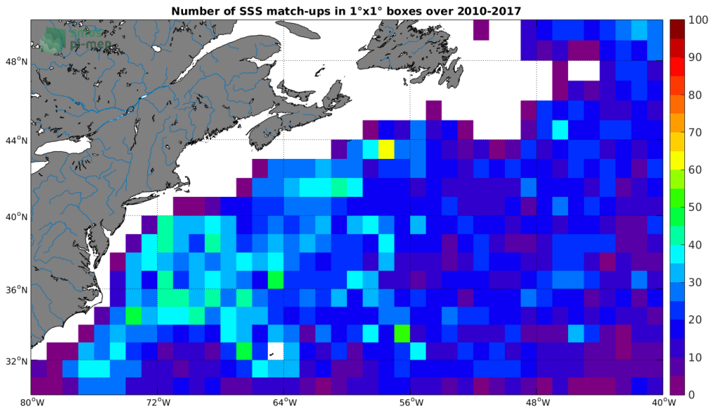
Figure 4: Number of SSS match-ups between Argo SSS and the SMOS-L3-CATDS-CECOS-IFREMER-V2-1DAY-0.5DEG SSS product for the Gulf Stream Pi-MEP region over 1^\circ \times 1^\circ boxes and for the full satellite product period.
