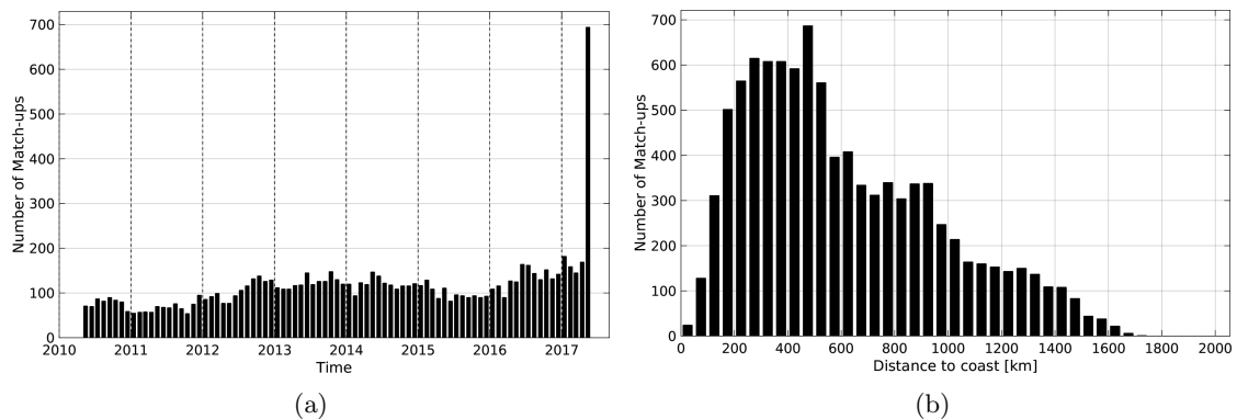
Figure 1: Number of match-ups between Argo and SMOS-L3-CATDS-CECOS-IFREMER-V2-1DAY-0.5deg SSS as a function of time (a) and as function of the distance to coast (b) over the Gulf Stream Pi-MEP region and for the full satellite product period.
