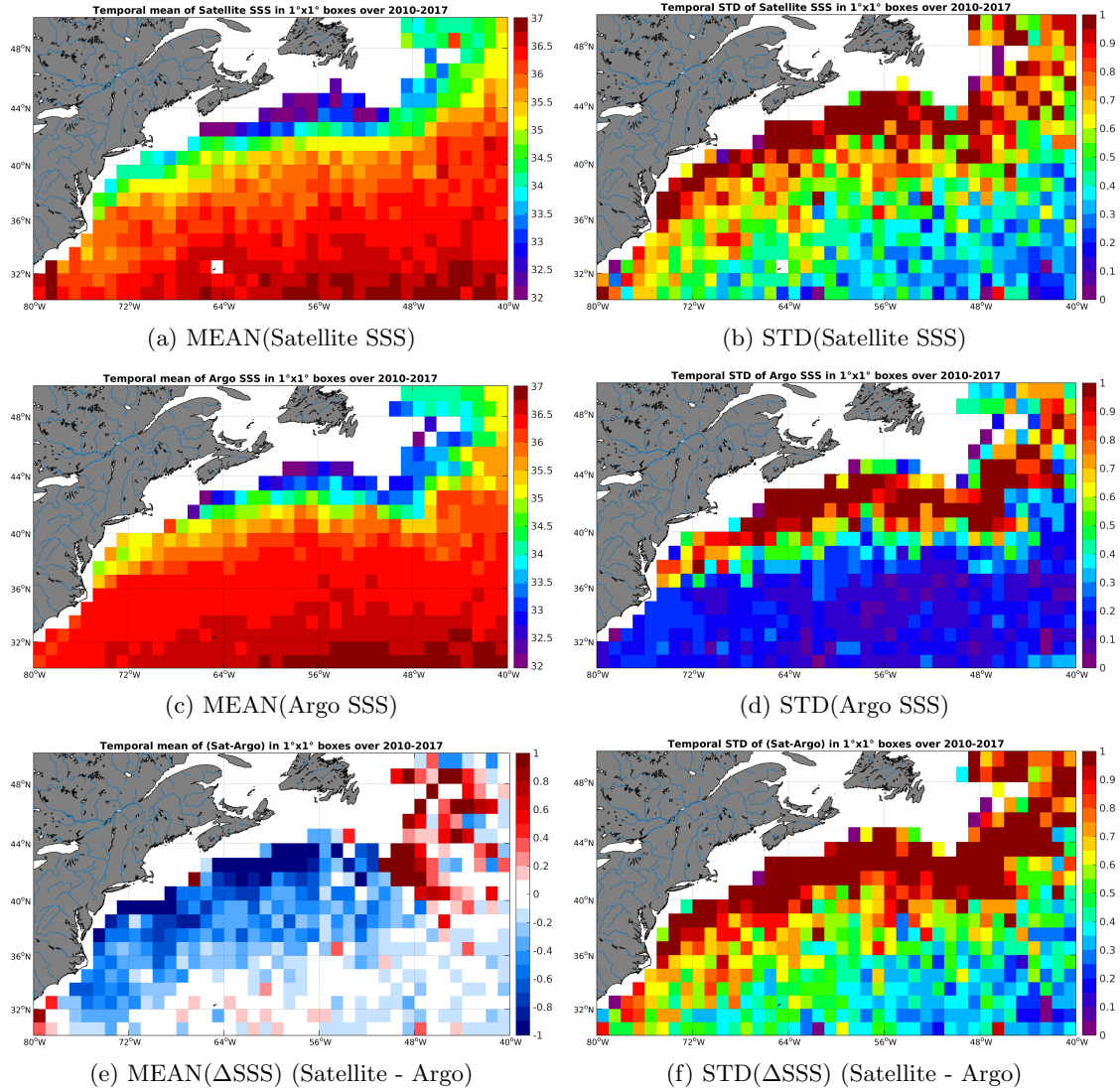
Figure 6: Temporal mean (left) and STD (right) of SSS from SMOS-L3-CATDS-CECOS-IFREMER-V2-1DAY-0.5deg (top), Argo (middle), and of \Delta SSS (Satellite - Argo). Only match-up pairs are used to generate these maps.
