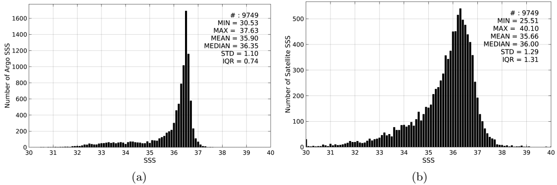
Figure 2: Histograms of SSS from Argo (a) and SMOS-L3-CATDS-CECOS-IFREMER-V2-1DAY-0.5deg (b) considering all match-up pairs per bins of 0.1 over the Gulf Stream Pi-MEP region and for the full satellite product period.
