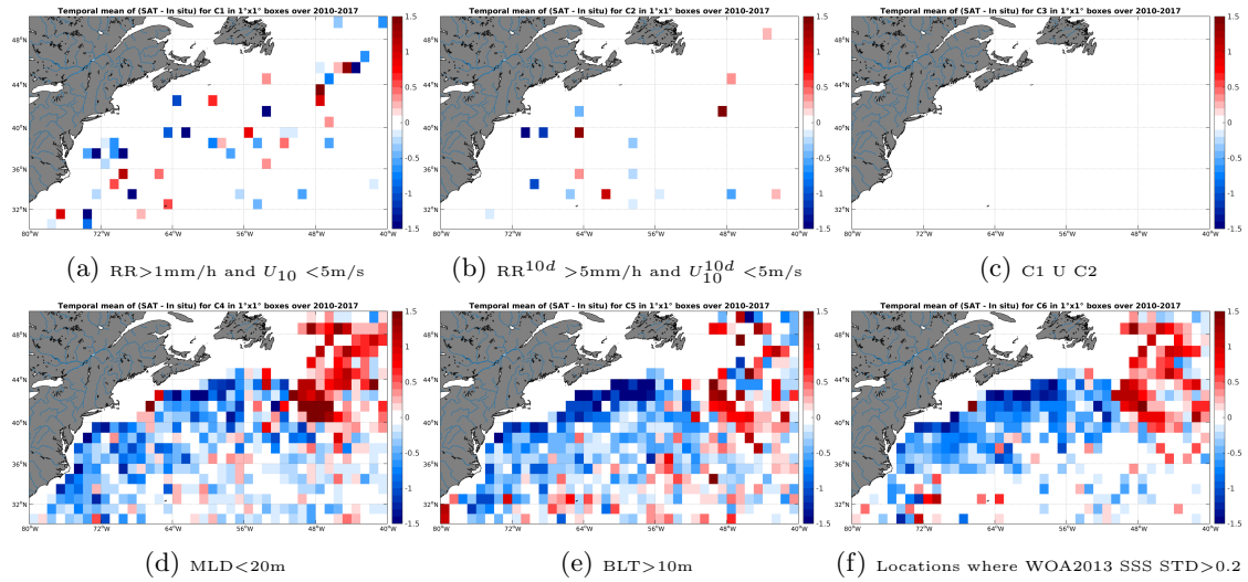
Figure 12: Temporal mean gridded over spatial boxes of size 1^\circ \times 1^\circ of \Delta SSS (SMOS-L3-CATDS-CECOS-IFREMER-V2-1DAY-0.5deg - Argo) for 6 different subdatasets corresponding to: RR > 1\text{mm/h} and U_{10} < 5\text{m/s} (a), RR^{10d} > 5\text{mm/h} and U_{10}^{10d} < 5\text{m/s} (b), C1 U C2 (c), MLD < 20\text{m} (d), BLT > 10\text{m} (e), Locations where WOA2013 SSS STD > 0.2 (f).
