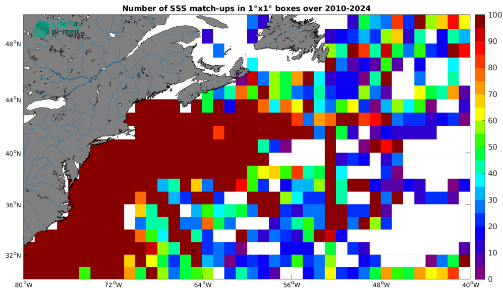
Figure 5: Number of SSS match-ups between TSG (SAMOS) SSS and the SMOS SSS L3 v335 - Monthly - 25 km (CATDS-CPDC) SSS product for the Gulf Stream Pi-MEP region over 1^\circ \times 1^\circ boxes and for the full satellite product period.
