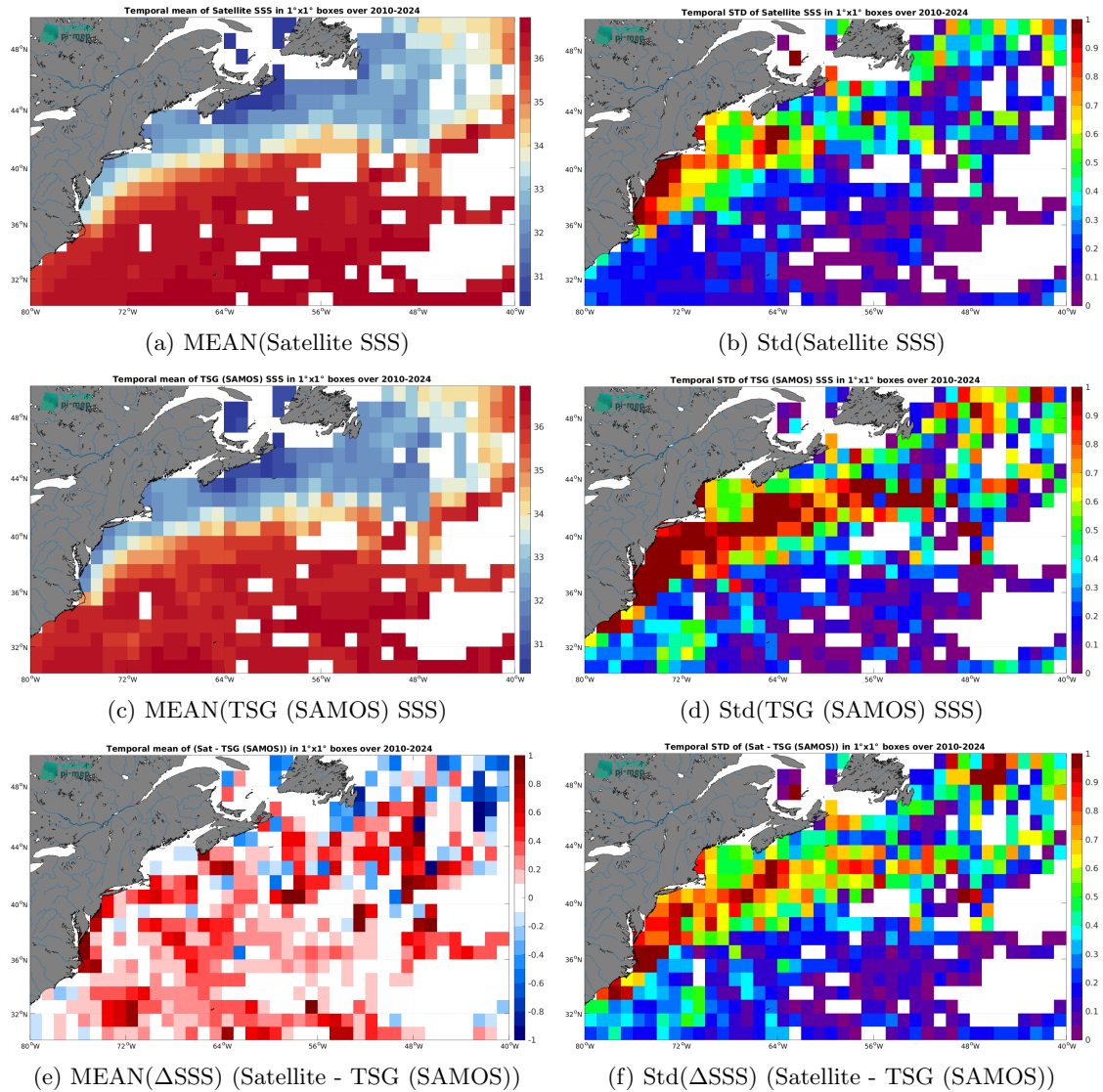
Figure 7: Temporal mean (left) and Std (right) of SSS from SMOS SSS L3 v335 - Monthly - 25 km (CATDS-CPDC) (top), TSG (SAMOS) (middle), and of \Delta SSS (Satellite - TSG (SAMOS)). Only match-up pairs are used to generate these maps.
