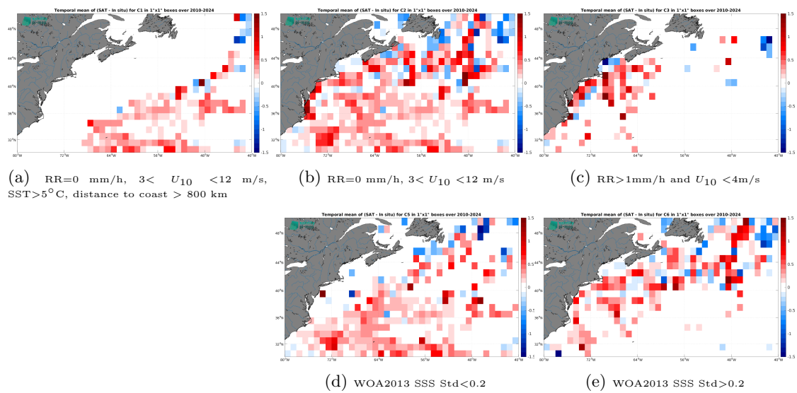
Figure 14: Temporal mean gridded over spatial boxes of size 1^\circ \times 1^\circ of \Delta SSS (SMOS SSS L3 v335 - Monthly - 25 km (CATDS-CPDC) - TSG (SAMOS)) for 5 different subdatasets corresponding to: RR=0 mm/h, 3 < U_{10} < 12 m/s, SST > 5^\circ\text{C} , distance to coast > 800 km (a), RR=0 mm/h, 3 < U_{10} < 12 m/s (b), RR > 1 mm/h and U_{10} < 4 m/s (c), WOA2013 SSS Std < 0.2 (d), WOA2013 SSS Std > 0.2 (e).
