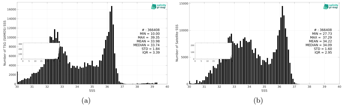
Figure 3: Histograms of SSS from TSG (SAMOS) (a) and SMOS SSS L3 v335 - Monthly - 25 km (CATDS-CPDC) (b) considering all match-up pairs per bins of 0.1 over the Gulf Stream Pi-MEP region and for the full satellite product period.
