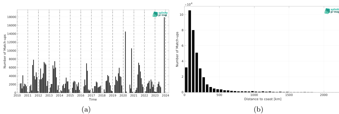
Figure 2: Number of match-ups between TSG (SAMOS) and SMOS SSS L3 v335 - Monthly - 25 km (CATDS-CPDC) SSS as a function of time (a) and as function of the distance to coast (b) over the Gulf Stream Pi-MEP region and for the full satellite product period.
