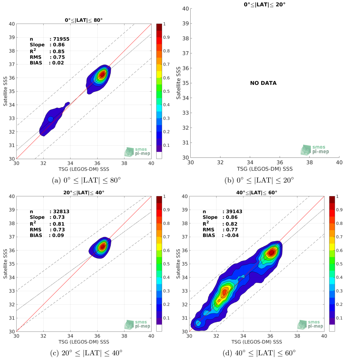
Figure 9: Contour maps of the concentration of SMOS SSS L3 v335 - Monthly - 25 km (CATDS-CPDC) SSS ( y -axis) versus TSG (LEGOS-DM) SSS ( x -axis) at match-up pairs for different latitude bands. For each plot, the red line shows x=y . The black thin and dashed lines indicate a linear fit through the data cloud and the \pm 95\% confidence levels, respectively. The number match-up pairs n , the slope and R^2 coefficient of the linear fit, the root mean square (RMS) and the mean bias between satellite and in situ data are indicated for each latitude band in each plots.
