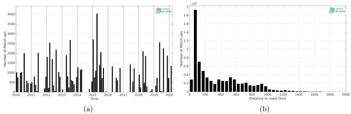
Figure 1: Number of match-ups between TSG (LEGOS-DM) and SMOS SSS L3 v335 - Monthly - 25 km (CATDS-CPDC) SSS as a function of time (a) and as function of the distance to coast (b) over the Gulf Stream Pi-MEP region and for the full satellite product period.
