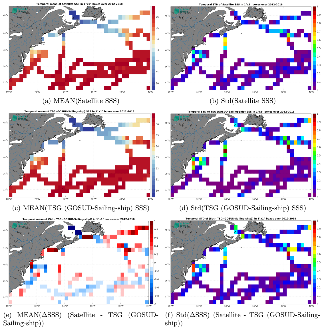
Figure 7: Temporal mean (left) and Std (right) of SSS from SMOS SSS L3 v335 - Monthly - 25 km (CATDS-CPDC) (top), TSG (GOSUD-Sailing-ship) (middle), and of \Delta SSS (Satellite - TSG (GOSUD-Sailing-ship)). Only match-up pairs are used to generate these maps.
