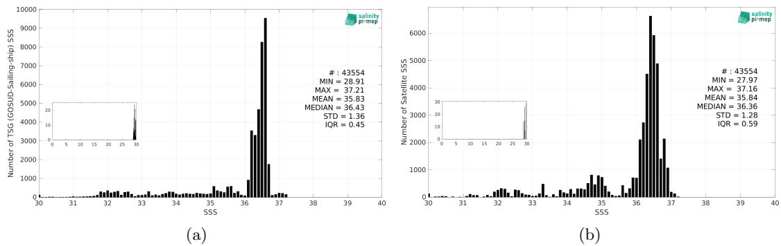
Figure 3: Histograms of SSS from TSG (GOSUD-Sailing-ship) (a) and SMOS SSS L3 v335 - Monthly - 25 km (CATDS-CPDC) (b) considering all match-up pairs per bins of 0.1 over the Gulf Stream Pi-MEP region and for the full satellite product period.
