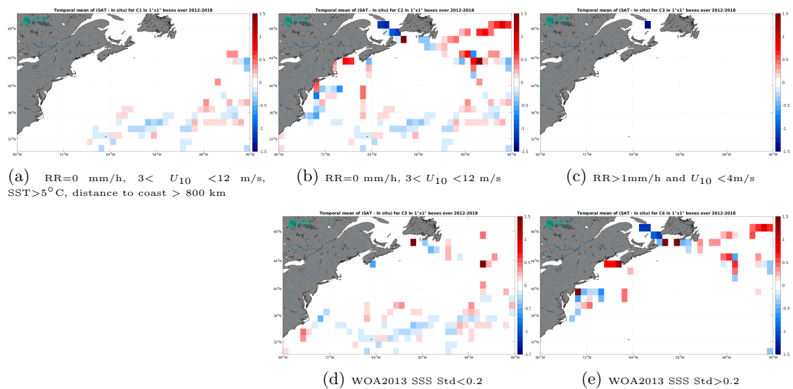
Figure 14: Temporal mean gridded over spatial boxes of size 1^\circ \times 1^\circ of \Delta SSS (SMOS SSS L3 v335 - Monthly - 25 km (CATDS-CPDC) - TSG (GOSUD-Sailing-ship)) for 5 different subdatasets corresponding to:RR=0 mm/h, 3 < U_{10} < 12 m/s, SST >5^\circ\text{C} , distance to coast > 800 km (a), RR=0 mm/h, 3 < U_{10} < 12 m/s (b), RR >1 mm/h and U_{10} < 4 m/s (c), WOA2013 SSS Std <0.2 (d), WOA2013 SSS Std >0.2 (e).
