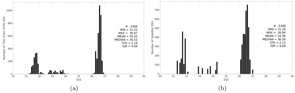
Figure 3: Histograms of SSS from TSG (CSIC-UTM) (a) and SMOS SSS L3 v335 - Monthly - 25 km (CATDS-CPDC) (b) considering all match-up pairs per bins of 0.1 over the Gulf Stream Pi-MEP region and for the full satellite product period.
