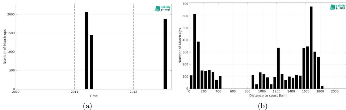
Figure 2: Number of match-ups between TSG (CSIC-UTM) and SMOS SSS L3 v335 - Monthly - 25 km (CATDS-CPDC) SSS as a function of time (a) and as function of the distance to coast (b) over the Gulf Stream Pi-MEP region and for the full satellite product period.
