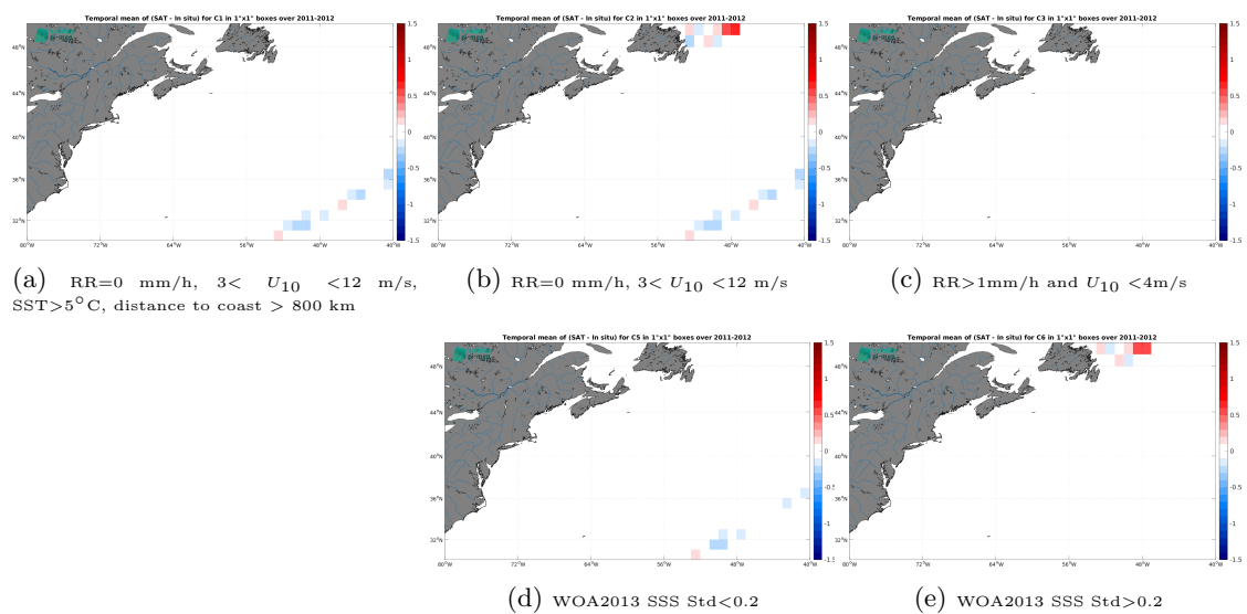
Figure 14: Temporal mean gridded over spatial boxes of size 1^\circ \times 1^\circ of \Delta SSS (SMOS SSS L3 v335 - Monthly - 25 km (CATDS-CPDC) - TSG (CSIC-UTM)) for 5 different subdatasets corresponding to:RR=0 mm/h, 3 < U_{10} < 12 m/s, SST >5^\circ C, distance to coast > 800 km (a), RR=0 mm/h, 3 < U_{10} < 12 m/s (b), RR >1 mm/h and U_{10} < 4 m/s (c), WOA2013 SSS Std <0.2 (d), WOA2013 SSS Std >0.2 (e).
