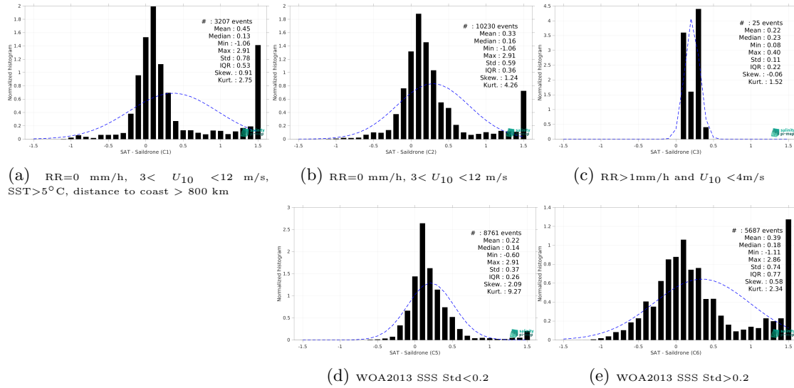
Figure 15: Normalized histogram of \Delta SSS (SMOS SSS L3 v335 - Monthly - 25 km (CATDS-CPDC) - Saldrone) for 5 different subdatasets corresponding to: RR=0 mm/h, 3 < U_{10} < 12 m/s, SST > 5°C, distance to coast > 800 km (a), RR=0 mm/h, 3 < U_{10} < 12 m/s (b), RR > 1mm/h and U_{10} < 4 m/s (c), WOA2013 SSS Std < 0.2 (d), WOA2013 SSS Std > 0.2 (e).
