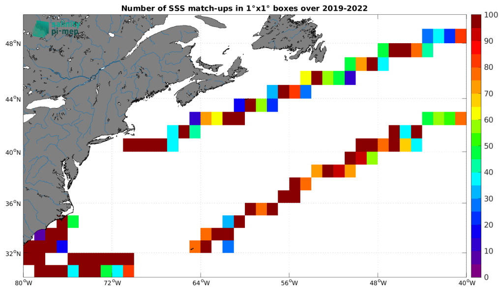
Figure 5: Number of SSS match-ups between Saildrone SSS and the SMOS SSS L3 v335 - Monthly - 25 km (CATDS-CPDC) SSS product for the Gulf Stream Pi-MEP region over 1^\circ \times 1^\circ boxes and for the full satellite product period.
