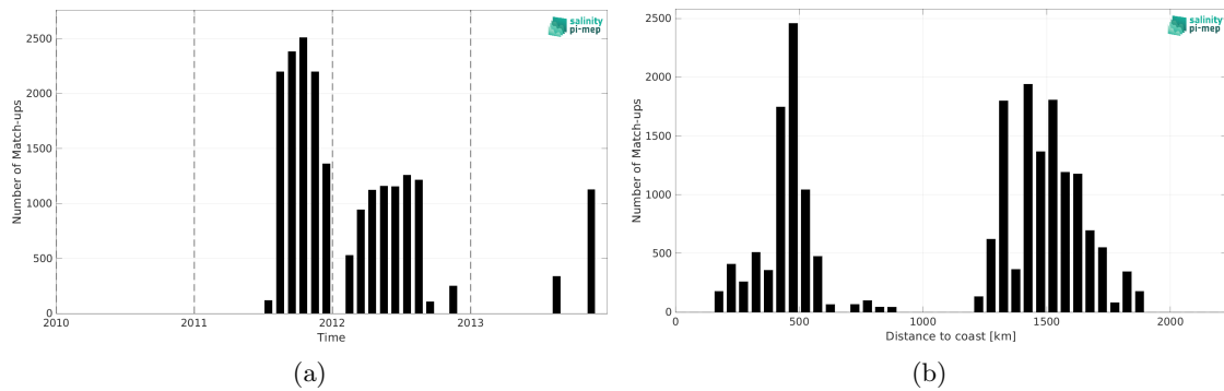
Figure 2: Number of match-ups between Surface drifters and SMOS SSS L3 v335 - Monthly - 25 km (CATDS-CPDC) SSS as a function of time (a) and as function of the distance to coast (b) over the Gulf Stream Pi-MEP region and for the full satellite product period.
