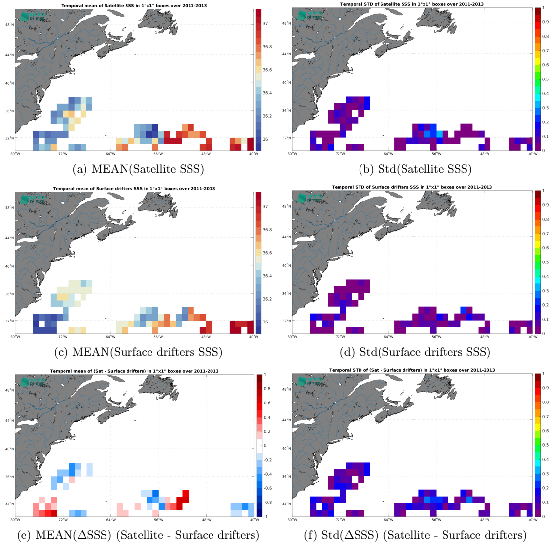
Figure 6: Temporal mean (left) and Std (right) of SSS from SMOS SSS L3 v335 - Monthly - 25 km (CATDS-CPDC) (top), Surface drifters (middle), and of \Delta SSS (Satellite - Surface drifters). Only match-up pairs are used to generate these maps.
