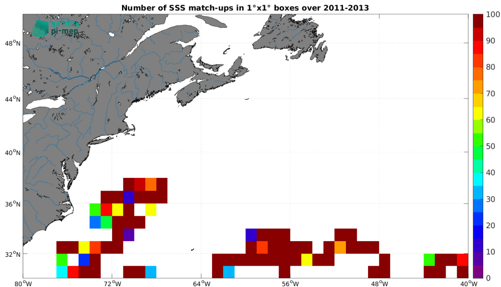
Figure 4: Number of SSS match-ups between Surface drifters SSS and the SMOS SSS L3 v335 - Monthly - 25 km (CATDS-CPDC) SSS product for the Gulf Stream Pi-MEP region over 1^\circ \times 1^\circ boxes and for the full satellite product period.
