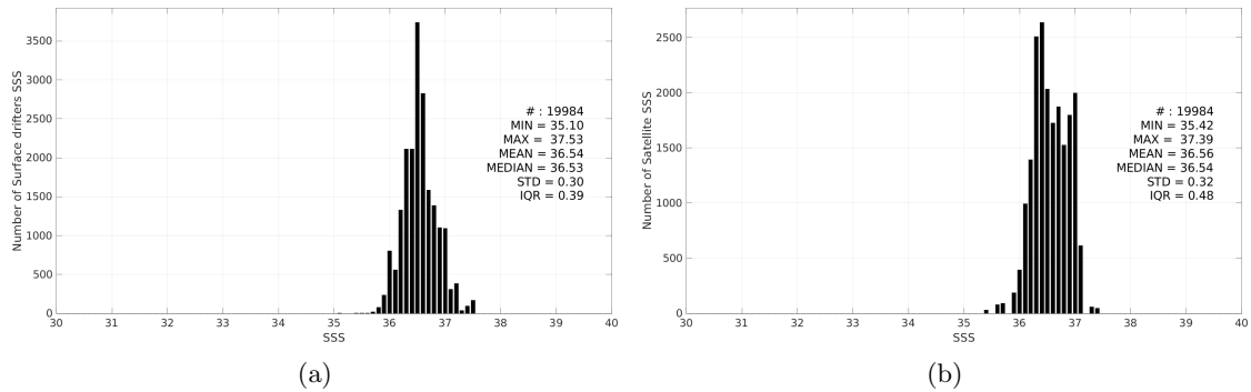
Figure 3: Histograms of SSS from Surface drifters (a) and SMOS SSS L3 v335 - Monthly - 25 km (CATDS-CPDC) (b) considering all match-up pairs per bins of 0.1 over the Gulf Stream Pi-MEP region and for the full satellite product period.
