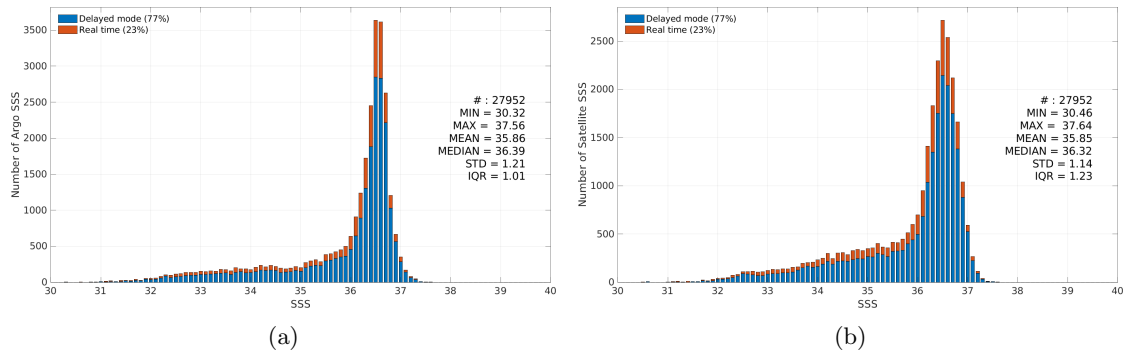
Figure 3: Histograms of SSS from Argo (a) and SMOS SSS L3 v335 - Monthly - 25 km (CATDS-CPDC) (b) considering all match-up pairs per bins of 0.1 over the Gulf Stream Pi-MEP region and for the full satellite product period.
