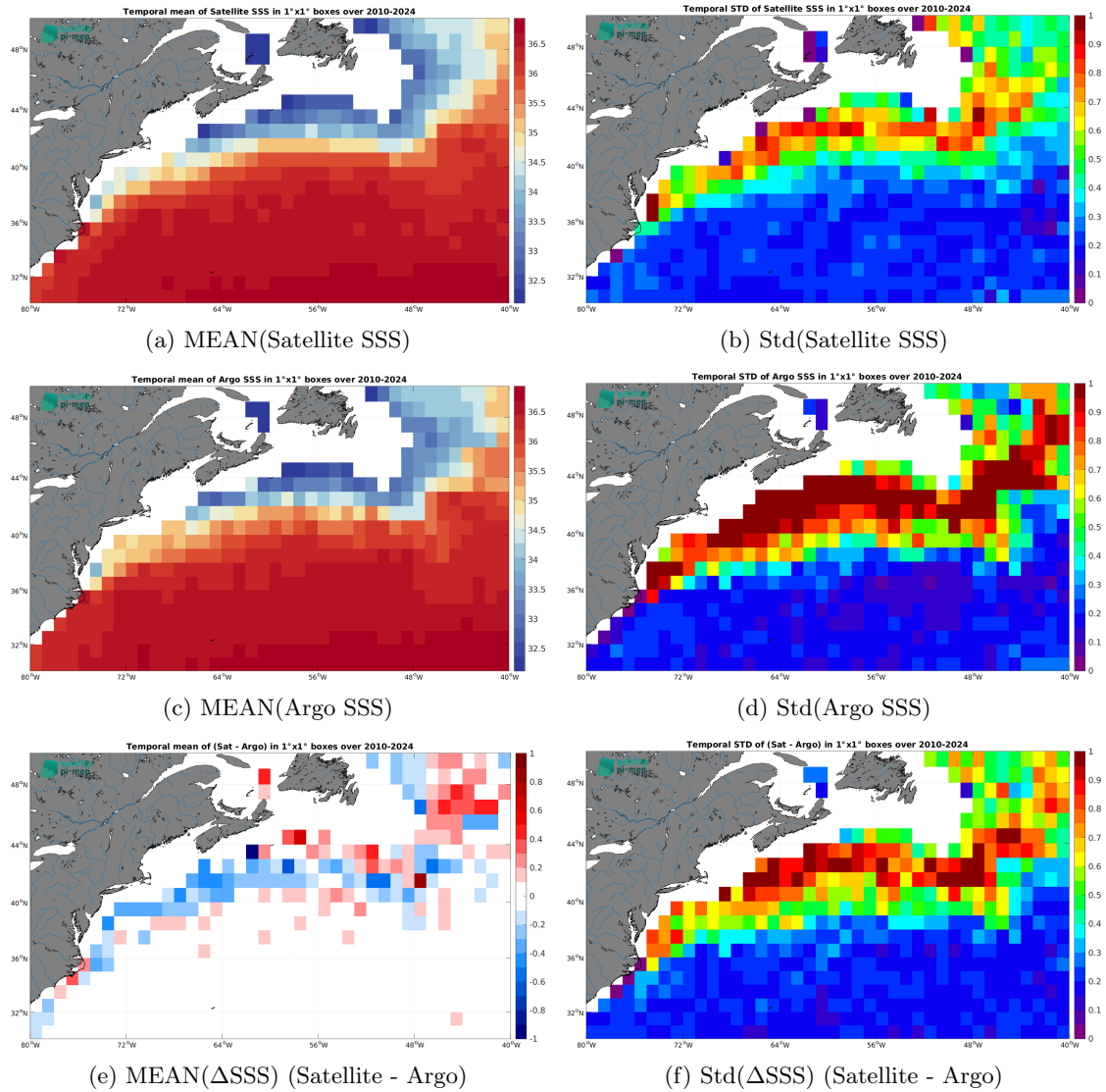
Figure 7: Temporal mean (left) and Std (right) of SSS from SMOS SSS L3 v335 - Monthly - 25 km (CATDS-CPDC) (top), Argo (middle), and of \Delta SSS (Satellite - Argo). Only match-up pairs are used to generate these maps.
