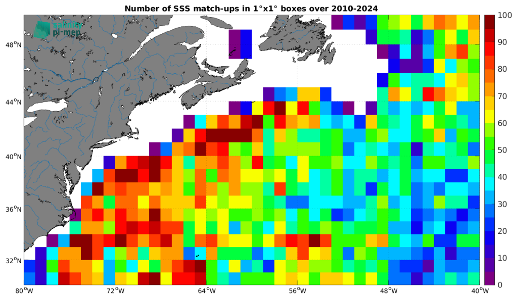
Figure 5: Number of SSS match-ups between Argo SSS and the SMOS SSS L3 v335 - Monthly - 25 km (CATDS-CPDC) SSS product for the Gulf Stream Pi-MEP region over 1^\circ \times 1^\circ boxes and for the full satellite product period.
