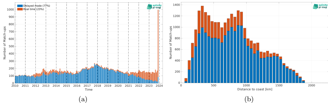
Figure 2: Number of match-ups between Argo and SMOS SSS L3 v335 - Monthly - 25 km (CATDS-CPDC) SSS as a function of time (a) and as function of the distance to coast (b) over the Gulf Stream Pi-MEP region and for the full satellite product period.
