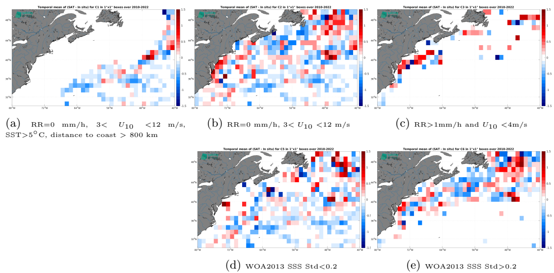
Figure 14: Temporal mean gridded over spatial boxes of size 1^\circ \times 1^\circ of \Delta\text{SSS} (SMOS SSS L3 v335 - 10 Days - 25 km (CATDS-CPDC) - TSG (LEGOS-DM)) for 5 different subdatasets corresponding to:RR=0 mm/h, 3 < U_{10} < 12 m/s, SST >5^\circ\text{C} , distance to coast > 800 km (a), RR=0 mm/h, 3 < U_{10} < 12 m/s (b), RR >1 mm/h and U_{10} < 4 m/s (c), WOA2013 SSS Std <0.2 (d), WOA2013 SSS Std >0.2 (e).
