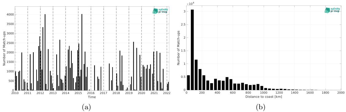
Figure 2: Number of match-ups between TSG (LEGOS-DM) and SMOS SSS L3 v335 - 10 Days - 25 km (CATDS-CPDC) SSS as a function of time (a) and as function of the distance to coast (b) over the Gulf Stream Pi-MEP region and for the full satellite product period.
