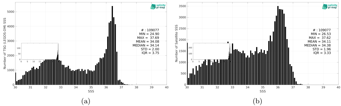
Figure 3: Histograms of SSS from TSG (LEGOS-DM) (a) and SMOS SSS L3 v335 - 10 Days - 25 km (CATDS-CPDC) (b) considering all match-up pairs per bins of 0.1 over the Gulf Stream Pi-MEP region and for the full satellite product period.
