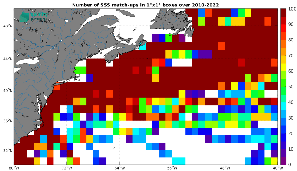
Figure 5: Number of SSS match-ups between TSG (LEGOS-DM) SSS and the SMOS SSS L3 v335 - 10 Days - 25 km (CATDS-CPDC) SSS product for the Gulf Stream Pi-MEP region over 1^\circ \times 1^\circ boxes and for the full satellite product period.
