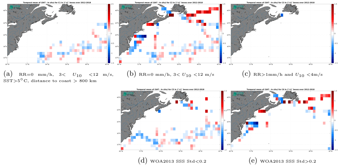
Figure 12: Temporal mean gridded over spatial boxes of size 1^{\circ}\times 1^{\circ} of \Delta SSS (SMOS SSS L3 v335 - 10 Days - 25 km (CATDS-CPDC) - TSG (GOSUD-Sailing-ship)) for 5 different subdatasets corresponding to:RR=0 mm/h, 3 < U_{10} < 12 m/s, SST >5^{\circ}\text{C} , distance to coast > 800 km (a), RR=0 mm/h, 3 < U_{10} < 12 m/s (b), RR >1 mm/h and U_{10} < 4 m/s (c), WOA2013 SSS Std <0.2 (d), WOA2013 SSS Std >0.2 (e).
