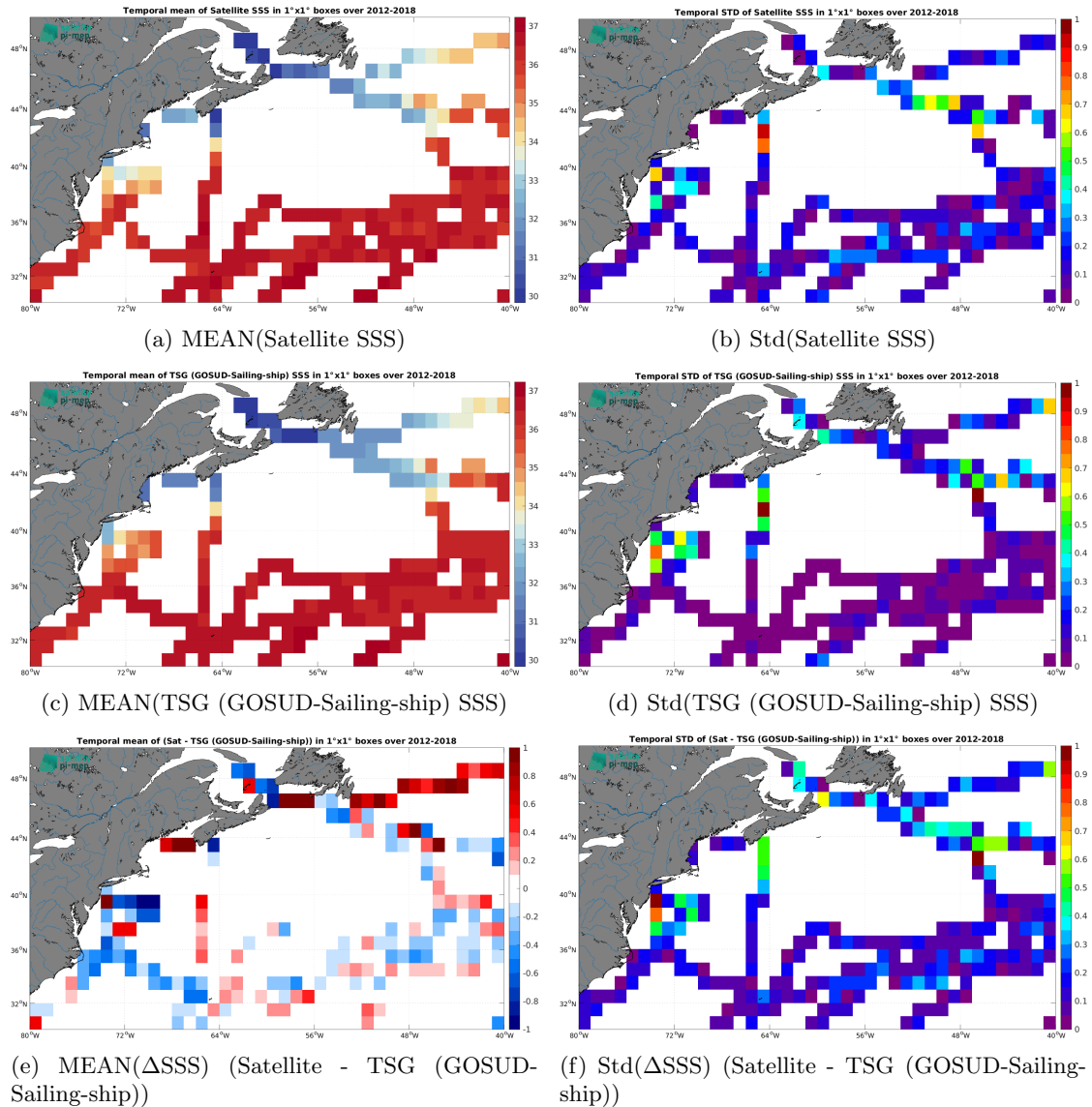
Figure 6: Temporal mean (left) and Std (right) of SSS from SMOS SSS L3 v335 - 10 Days - 25 km (CATDS-CPDC) (top), TSG (GOSUD-Sailing-ship) (middle), and of \Delta SSS (Satellite - TSG (GOSUD-Sailing-ship)). Only match-up pairs are used to generate these maps.
