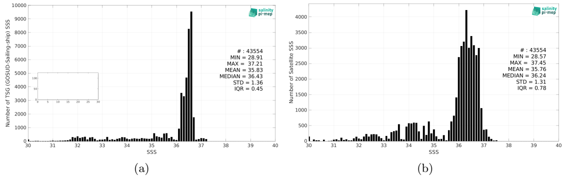
Figure 2: Histograms of SSS from TSG (GOSUD-Sailing-ship) (a) and SMOS SSS L3 v335 - 10 Days - 25 km (CATDS-CPDC) (b) considering all match-up pairs per bins of 0.1 over the Gulf Stream Pi-MEP region and for the full satellite product period.
