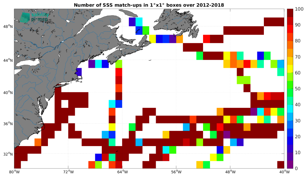
Figure 4: Number of SSS match-ups between TSG (GOSUD-Sailing-ship) SSS and the SMOS SSS L3 v335 - 10 Days - 25 km (CATDS-CPDC) SSS product for the Gulf Stream Pi-MEP region over 1^\circ \times 1^\circ boxes and for the full satellite product period.
