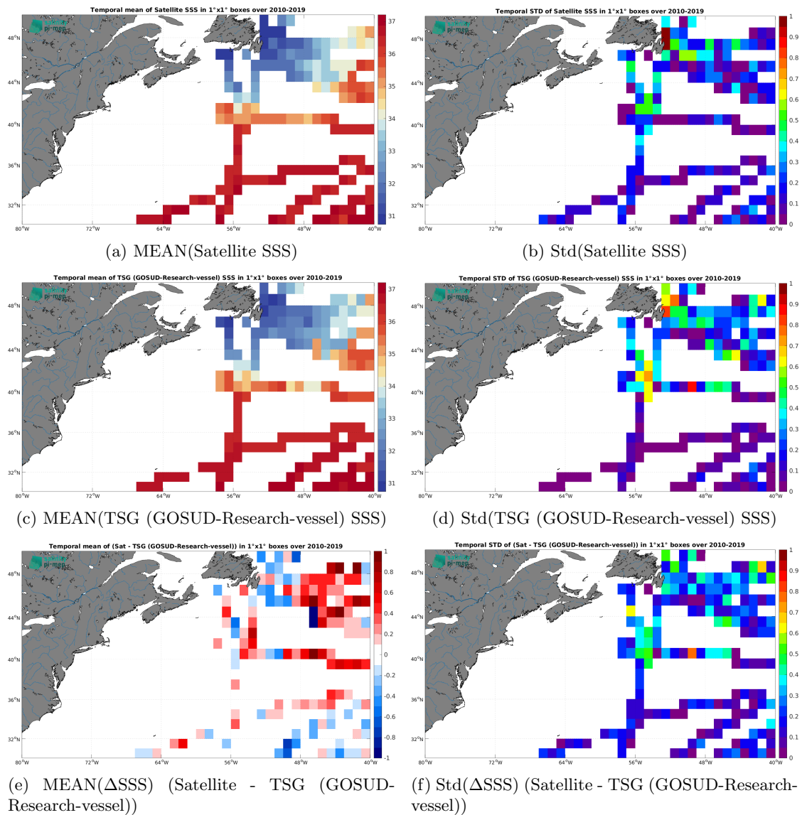
Figure 7: Temporal mean (left) and Std (right) of SSS from SMOS SSS L3 v335 - 10 Days - 25 km (CATDS-CPDC) (top), TSG (GOSUD-Research-vessel) (middle), and of \Delta SSS (Satellite - TSG (GOSUD-Research-vessel)). Only match-up pairs are used to generate these maps.
