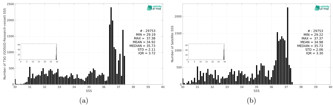
Figure 3: Histograms of SSS from TSG (GOSUD-Research-vessel) (a) and SMOS SSS L3 v335 - 10 Days - 25 km (CATDS-CPDC) (b) considering all match-up pairs per bins of 0.1 over the Gulf Stream Pi-MEP region and for the full satellite product period.
