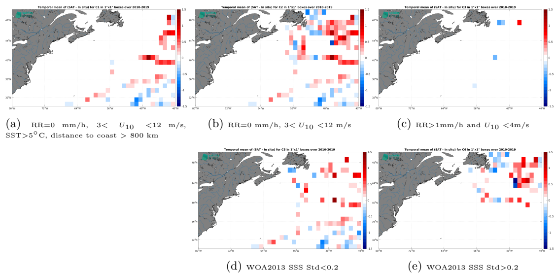
Figure 14: Temporal mean gridded over spatial boxes of size 1^\circ \times 1^\circ of \Delta\text{SSS} (SMOS SSS L3 v335 - 10 Days - 25 km (CATDS-CPDC) - TSG (GOSUD-Research-vessel)) for 5 different subdatasets corresponding to:RR=0 mm/h, 3 < U_{10} < 12 m/s, SST >5^\circ\text{C} , distance to coast > 800 km (a), RR=0 mm/h, 3 < U_{10} < 12 m/s (b), RR >1 mm/h and U_{10} < 4 m/s (c), WOA2013 SSS Std <0.2 (d), WOA2013 SSS Std >0.2 (e).
