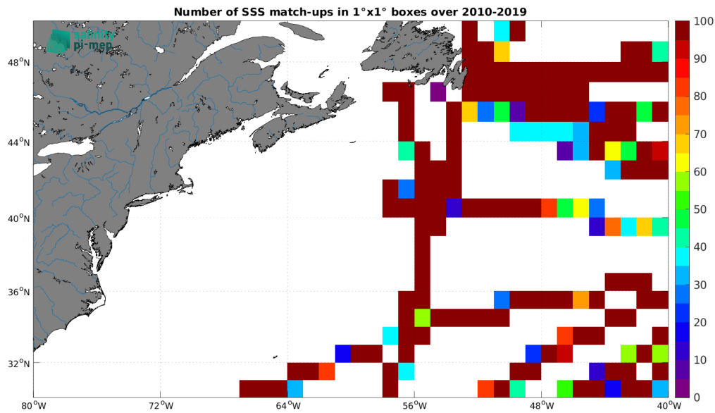
Figure 5: Number of SSS match-ups between TSG (GOSUD-Research-vessel) SSS and the SMOS SSS L3 v335 - 10 Days - 25 km (CATDS-CPDC) SSS product for the Gulf Stream Pi-MEP region over 1^\circ \times 1^\circ boxes and for the full satellite product period.
