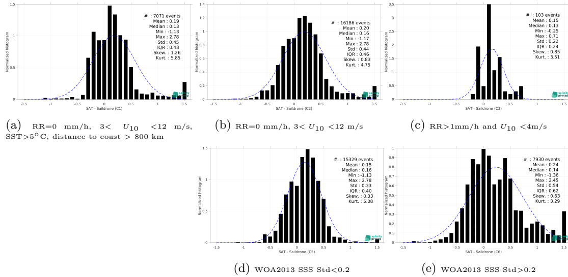
Figure 15: Normalized histogram of \Delta SSS (SMOS SSS L3 v335 - 10 Days - 25 km (CATDS-CPDC) - Salldrone) for 5 different subdatasets corresponding to: RR=0 mm/h, 3 < U_{10} < 12 m/s, SST > 5°C, distance to coast > 800 km (a), RR=0 mm/h, 3 < U_{10} < 12 m/s (b), RR > 1mm/h and U_{10} < 4 m/s (c), WOA2013 SSS Std < 0.2 (d), WOA2013 SSS Std > 0.2 (e).
